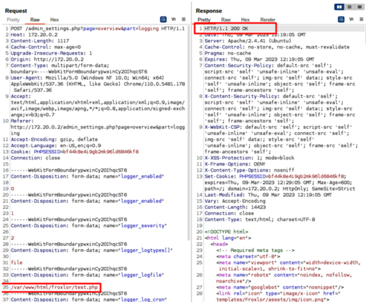
Figure 5-4. Modifying the filepath by intercepting the request in Burp Suite
