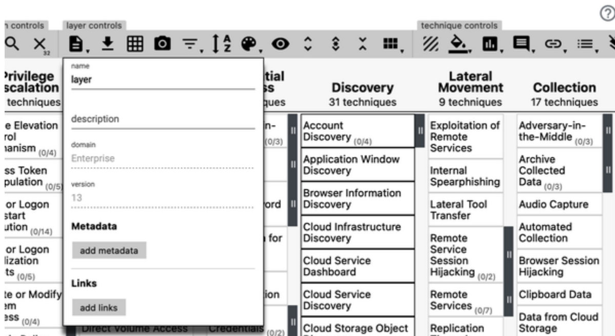
Figure 6-3. Layer name and description
