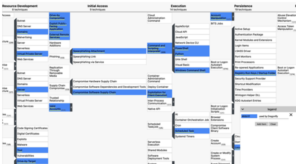
Figure 6-8. APT Dragonfly visualized in ATT&CK Navigator
