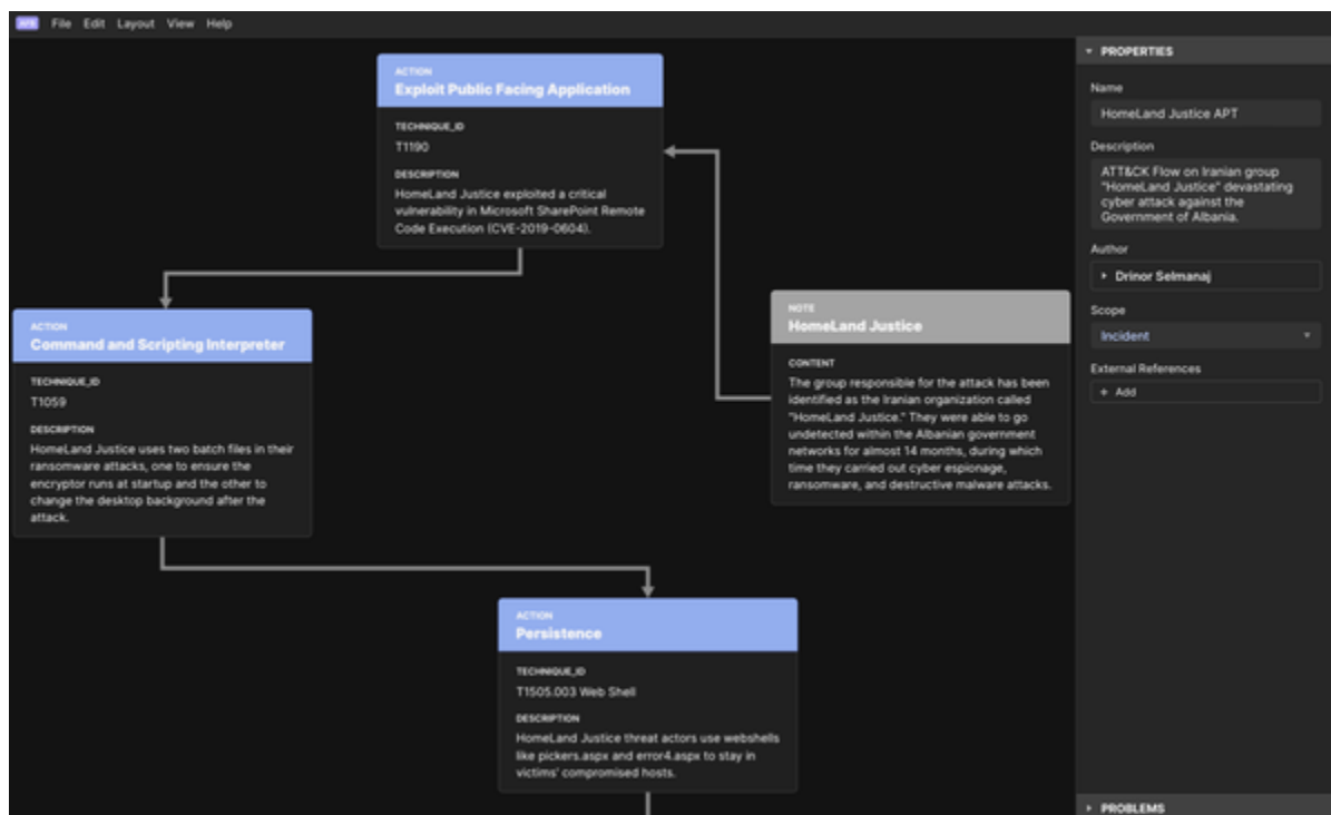
Figure 6-11. Attack Flow of the Iranian APT group
