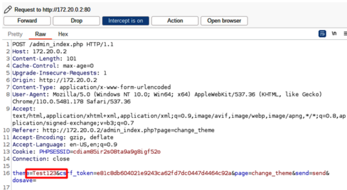
Figure 5-6. Testing theme manipulation by changing it using Burp Suite
