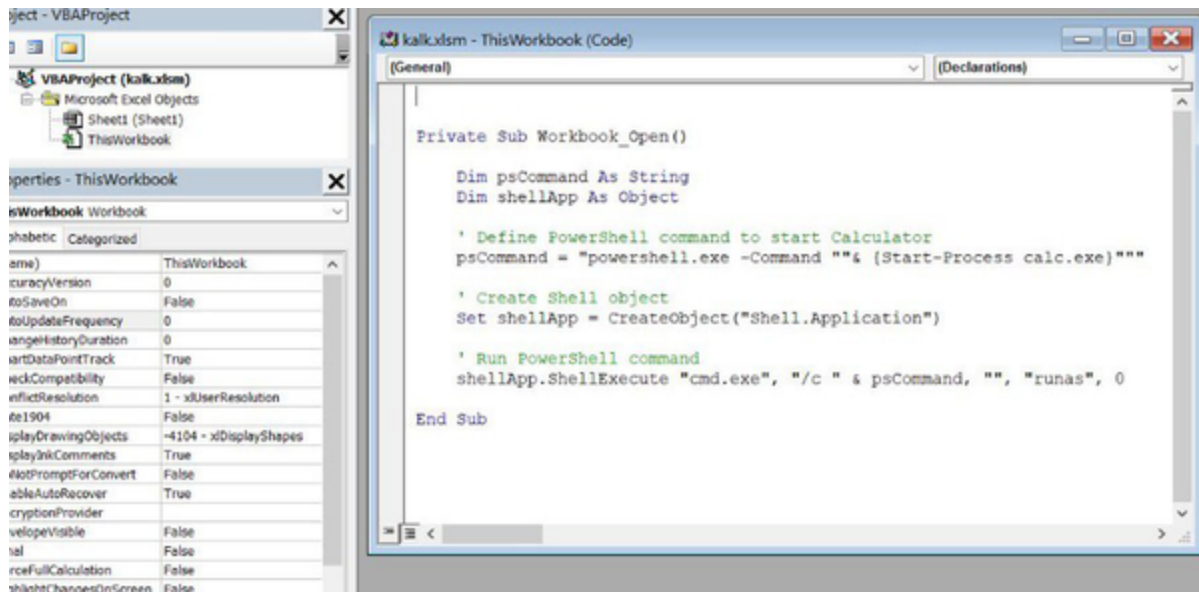
Figure 5-1. Example of creating a macro-enabled Excel file
