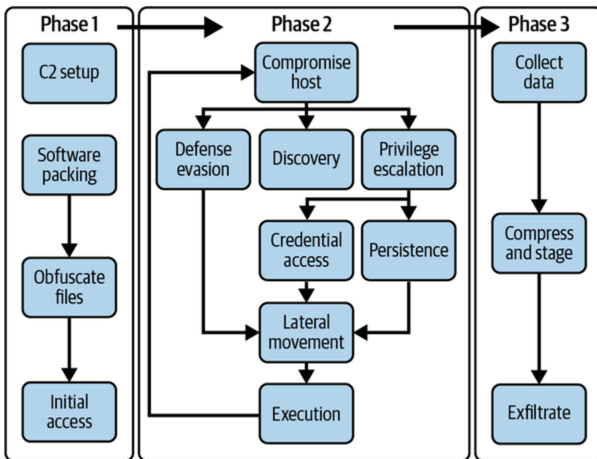
Figure 1-4. APT3's three phases of action according to MITRE
