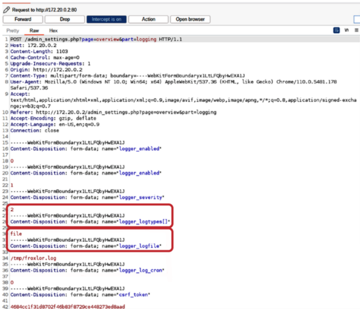
Figure 5-3. Intercepting the file creation request with Burp Suite
