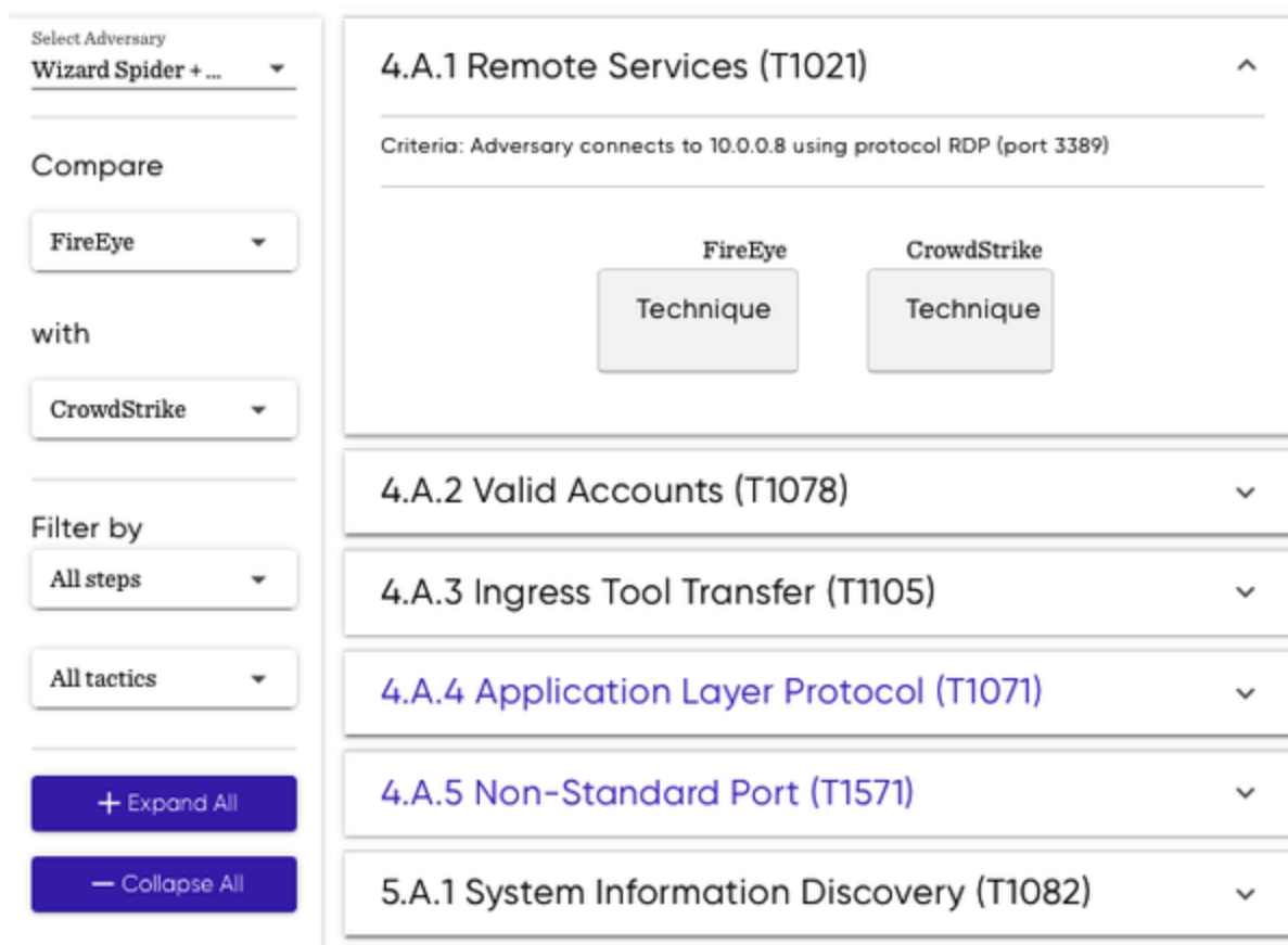
Figure 1-3. MITRE Engenuity ATT&CK Evaluation results for Wizard Spider and Sandworm emulation plans
