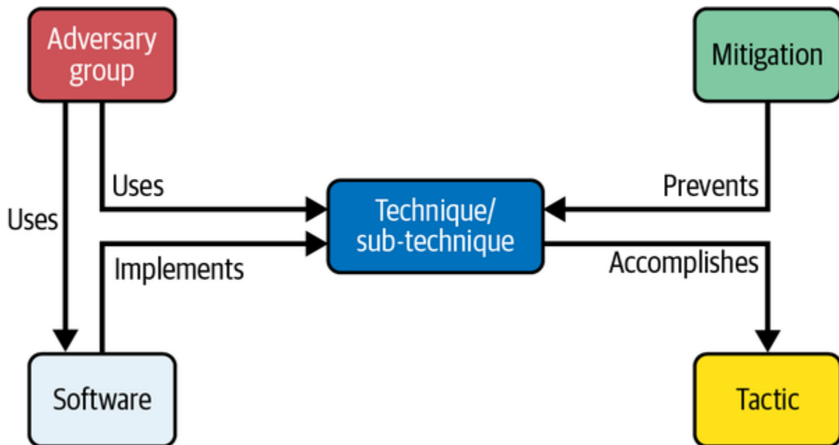
Figure 3-5. ATT&CK object model relationships
