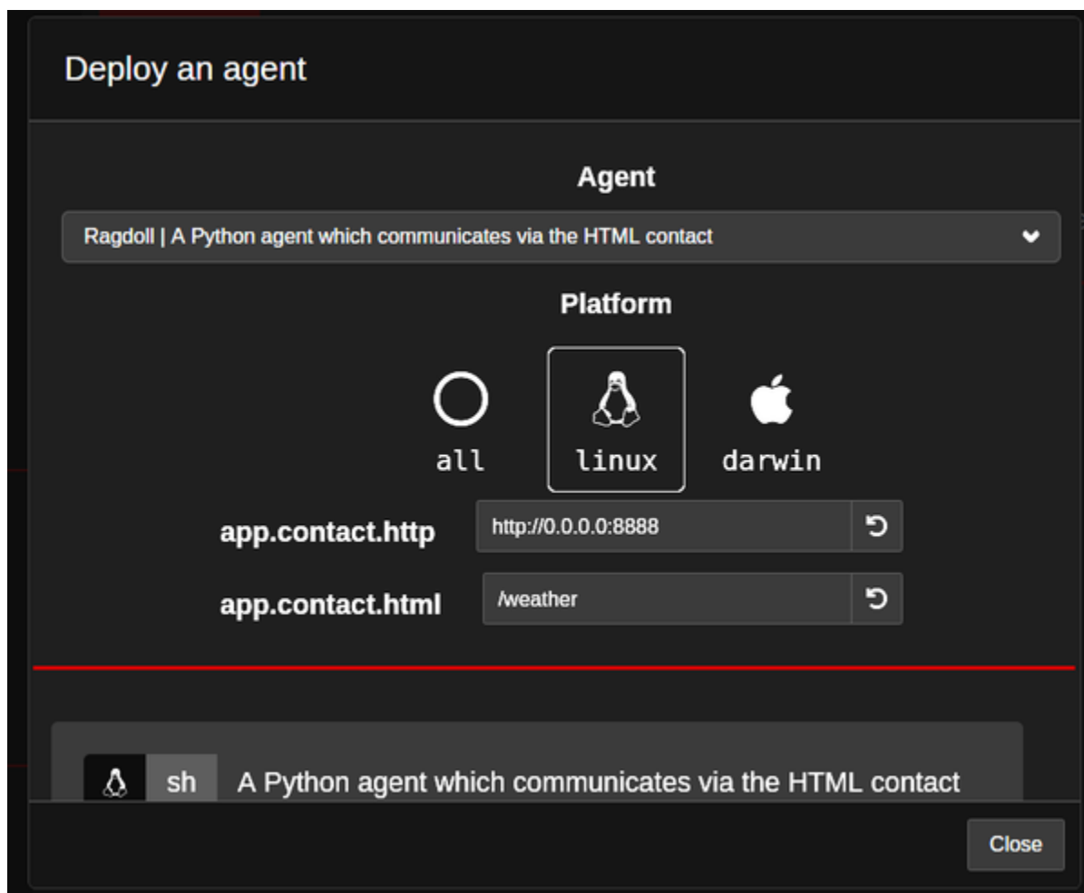
Figure 13-2. Deploying an agent in Caldera
