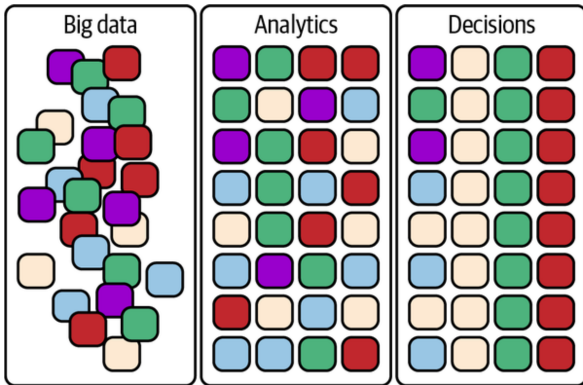
Figure 7-5. Pattern recognition 4
