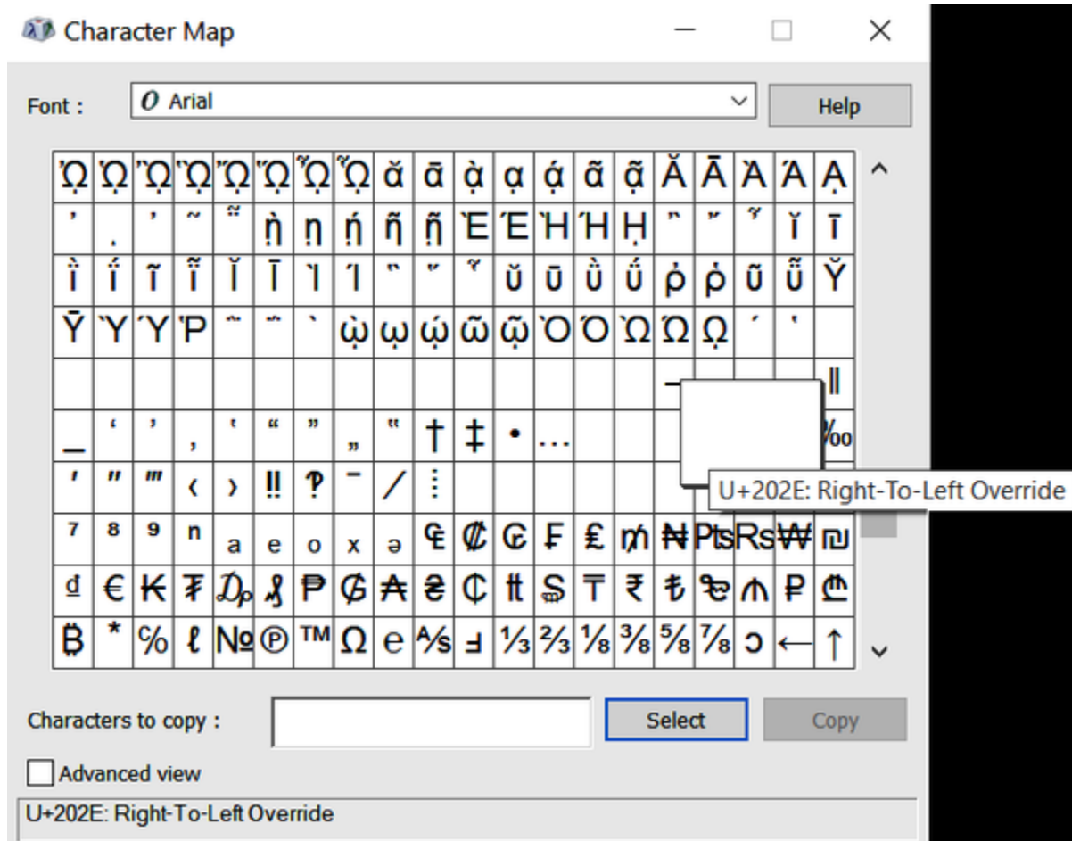
Figure 5-2. RLO character in the Character Map
