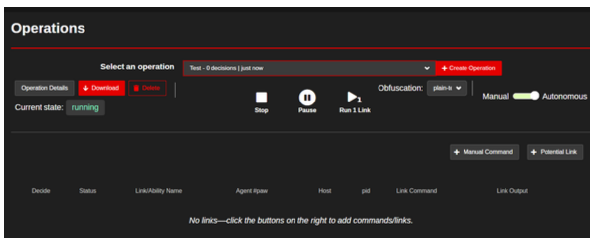
Figure 13-7. Running operations
