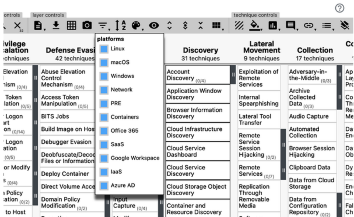
Figure 6-4. Filtering platforms
