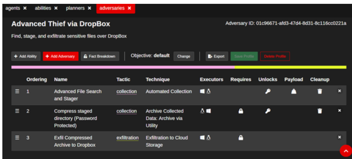
Figure 13-4. Mapped adversary
