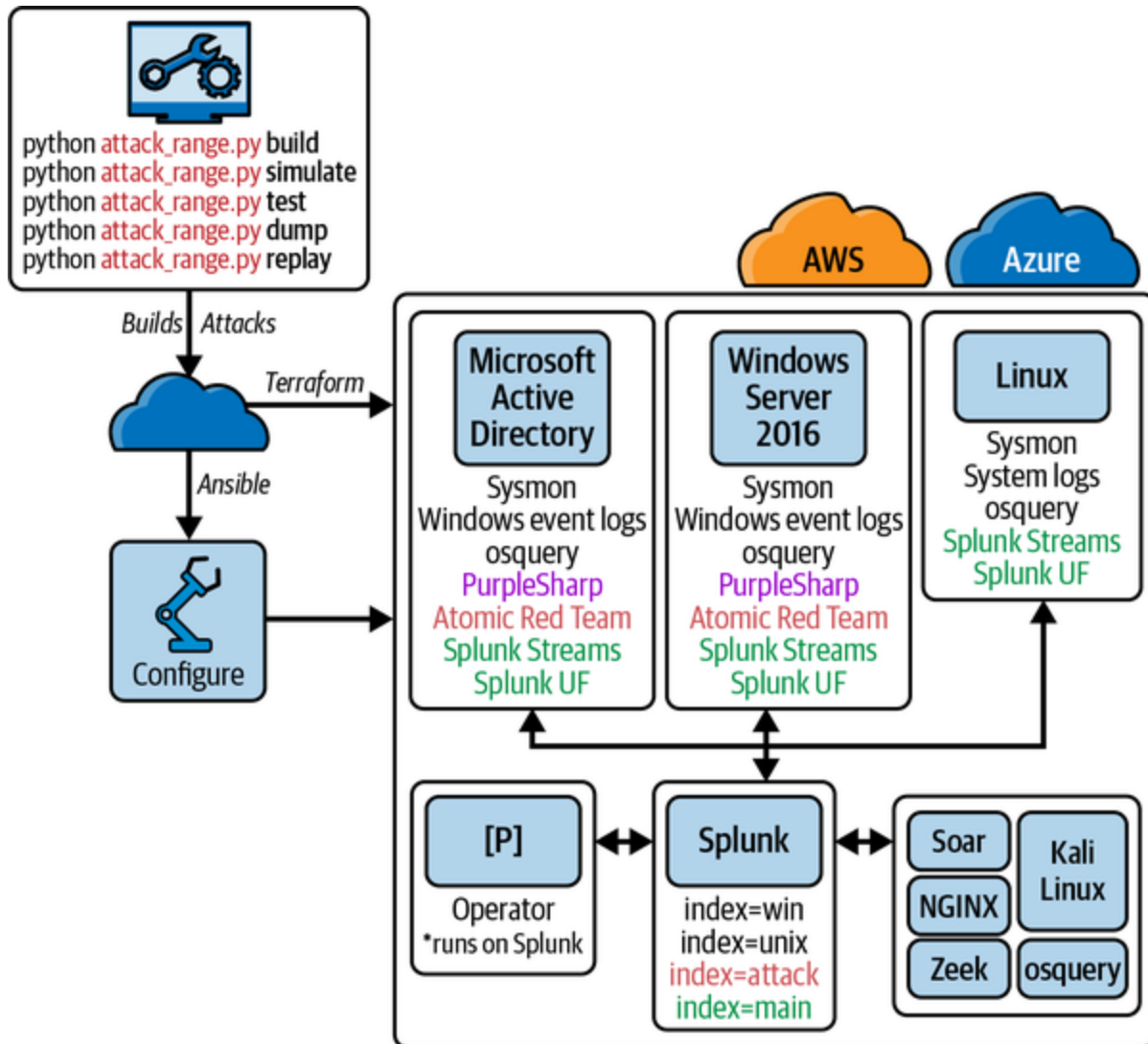
Figure 11-1. Architectural overview of the Splunk Attack Range and its integrated components
