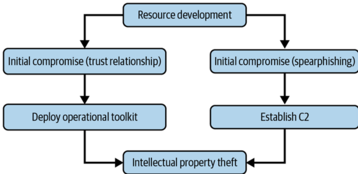
Figure 11-4. Adversary Emulation Library: menuPass Operations Flow
