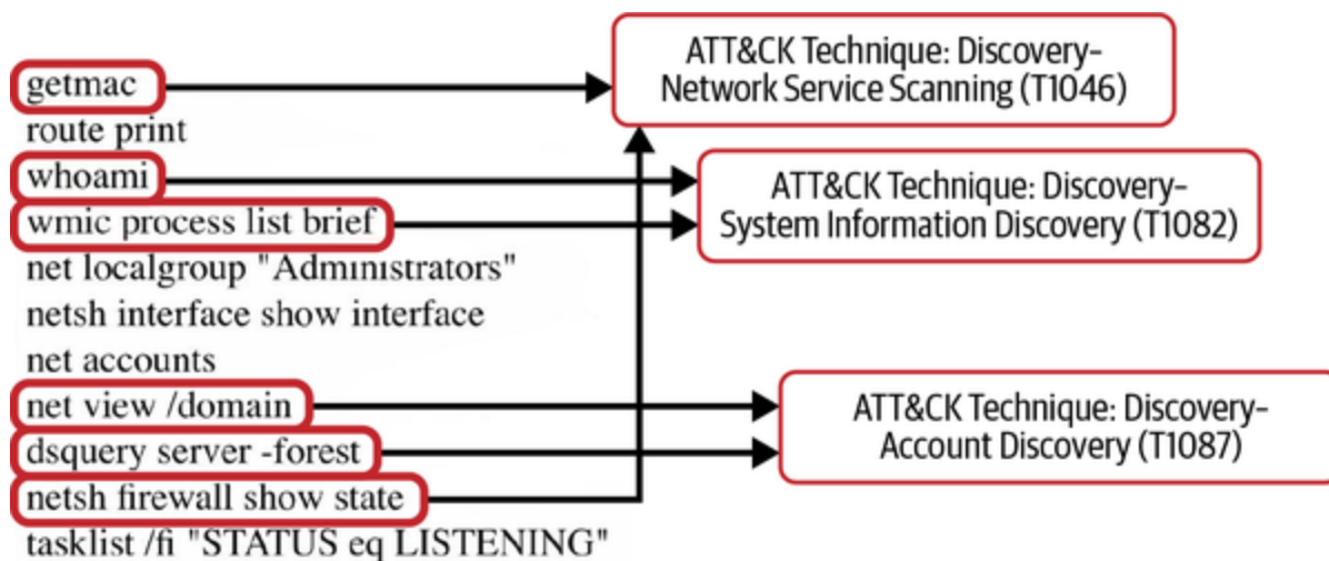
Figure 7-4. Mapping intelligence from raw data to the MITRE ATT&CK framework
