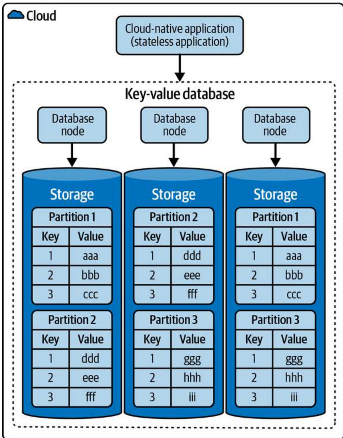
Figure 7-16. Key-Value Database
