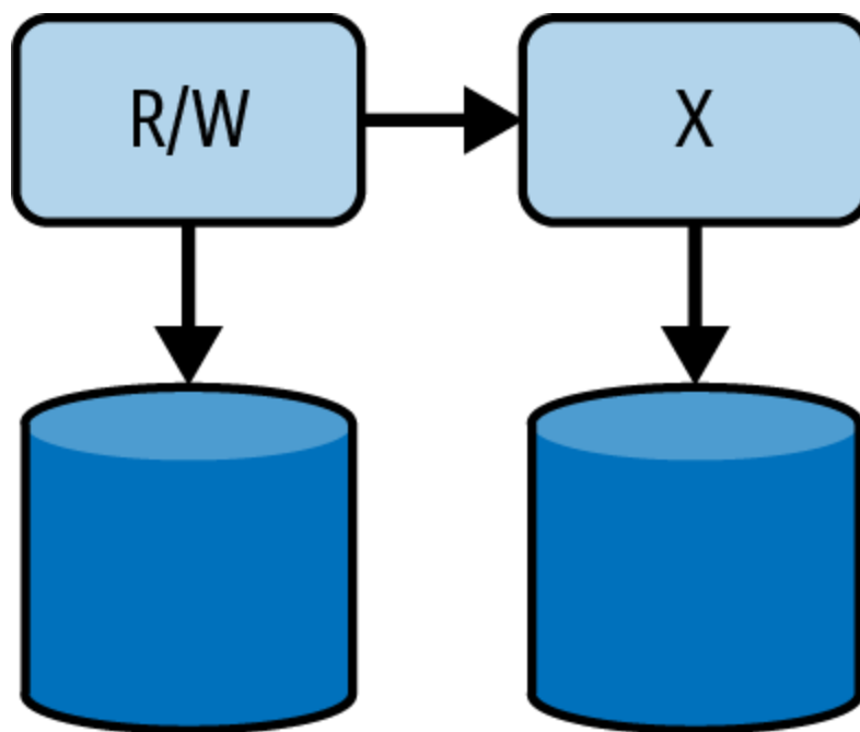
Figure 7-3. Leader-follower topology
