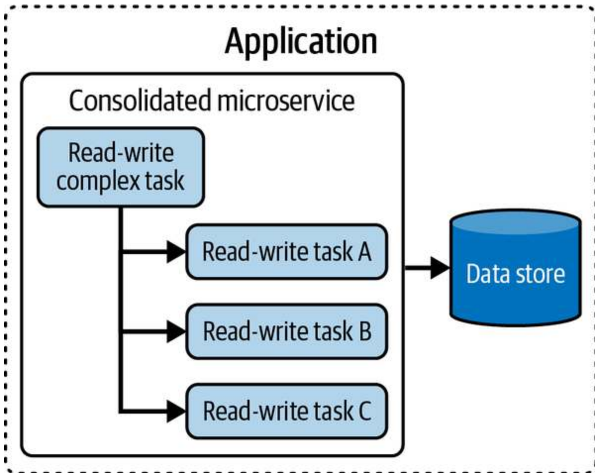
Figure 4-26. Consolidated microservice
