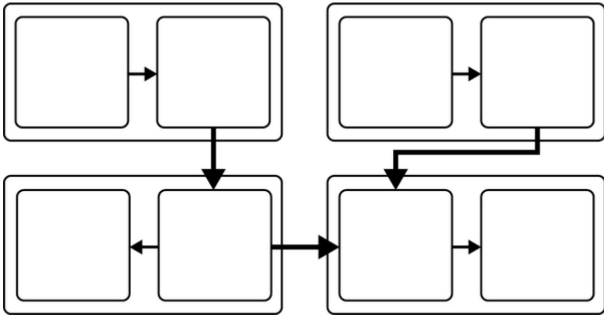
Figure 2-10. Distributed Architecture
