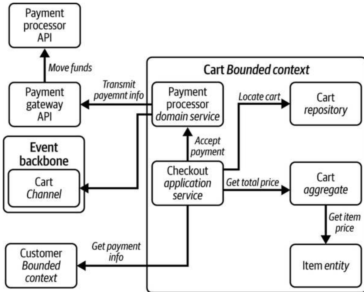
Figure 5-23. Checkout process
