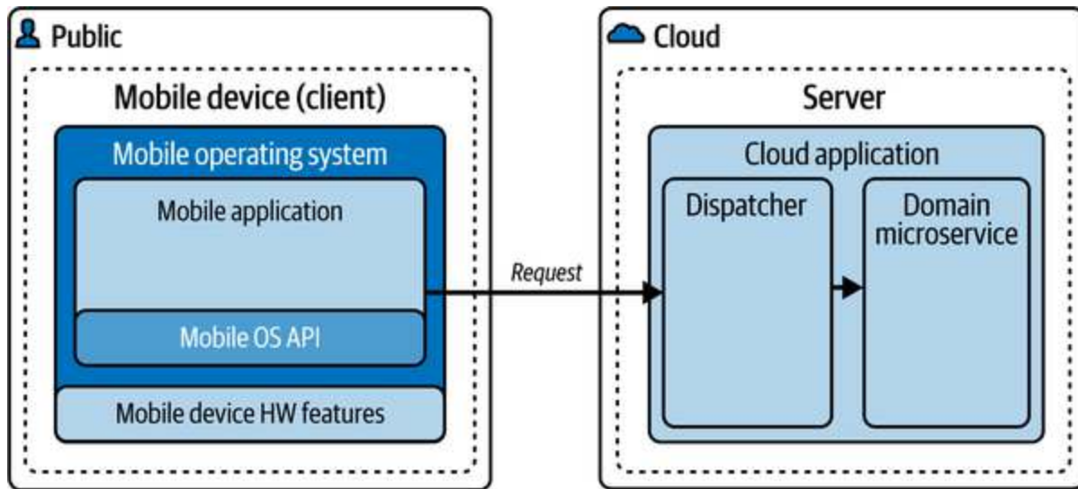
Figure 8-17. Mobile Application
