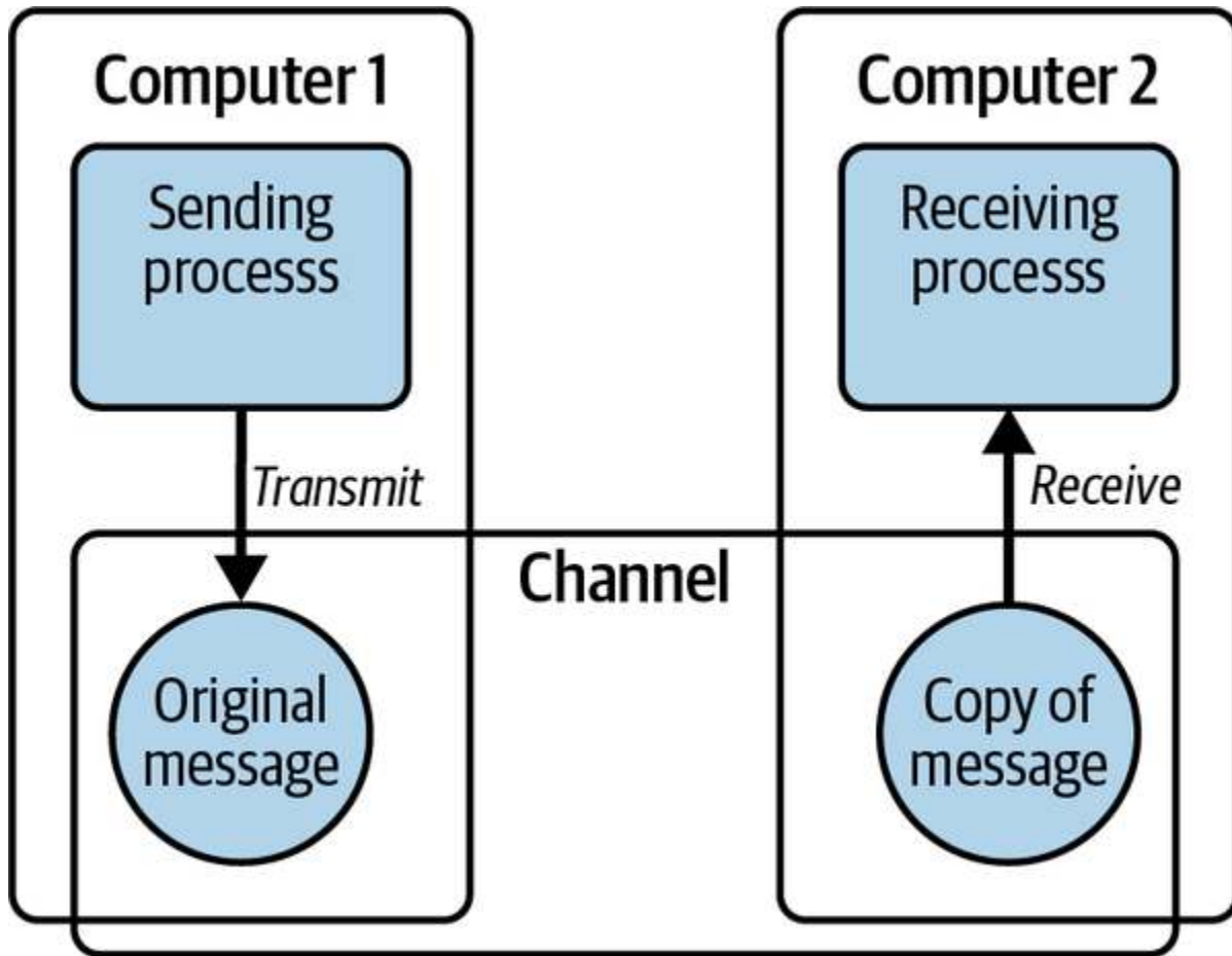
Figure 6-3. Messaging pattern
