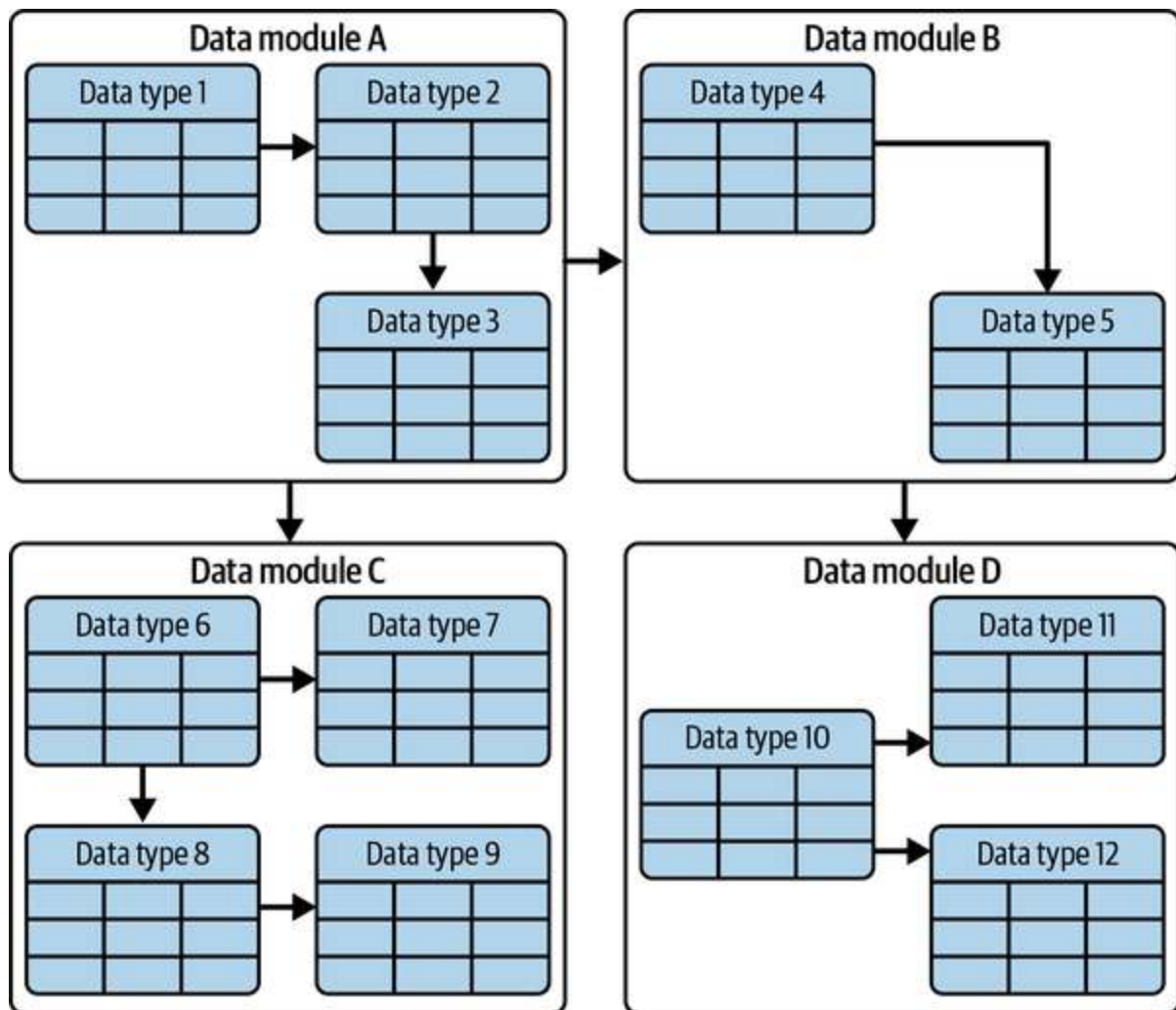
Figure 7-25. Data Module
