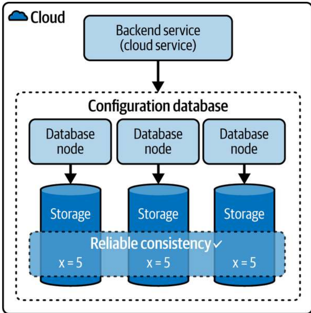
Figure 7-12. Configuration Database
