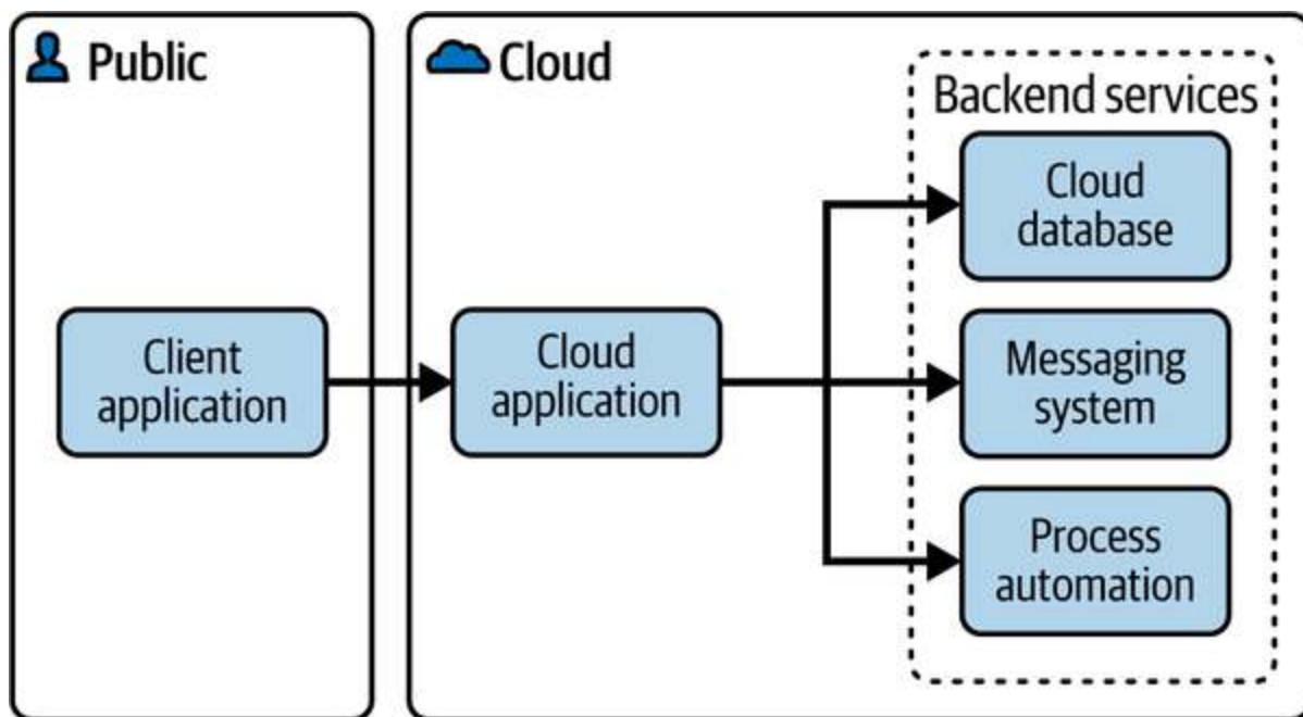
Figure 3-15. Backend Services
