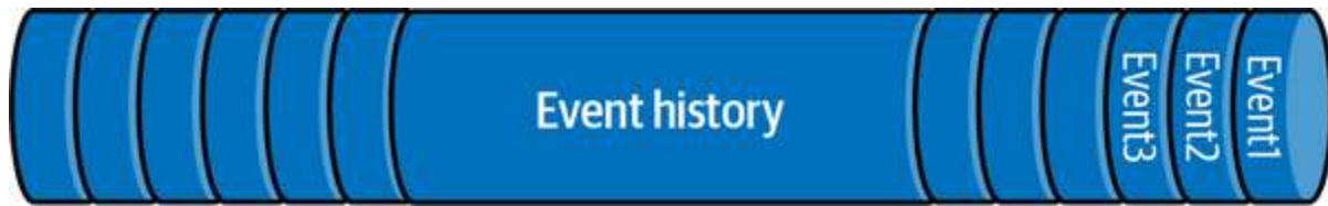
Figure 6-25. Event sourcing
