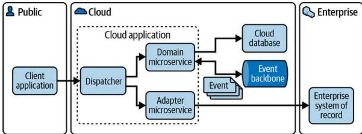
Figure 1-1. Cloud Application
