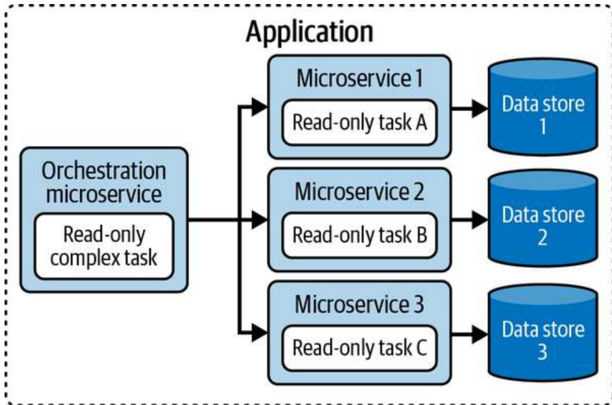
Figure 4-25. Orchestration microservice
