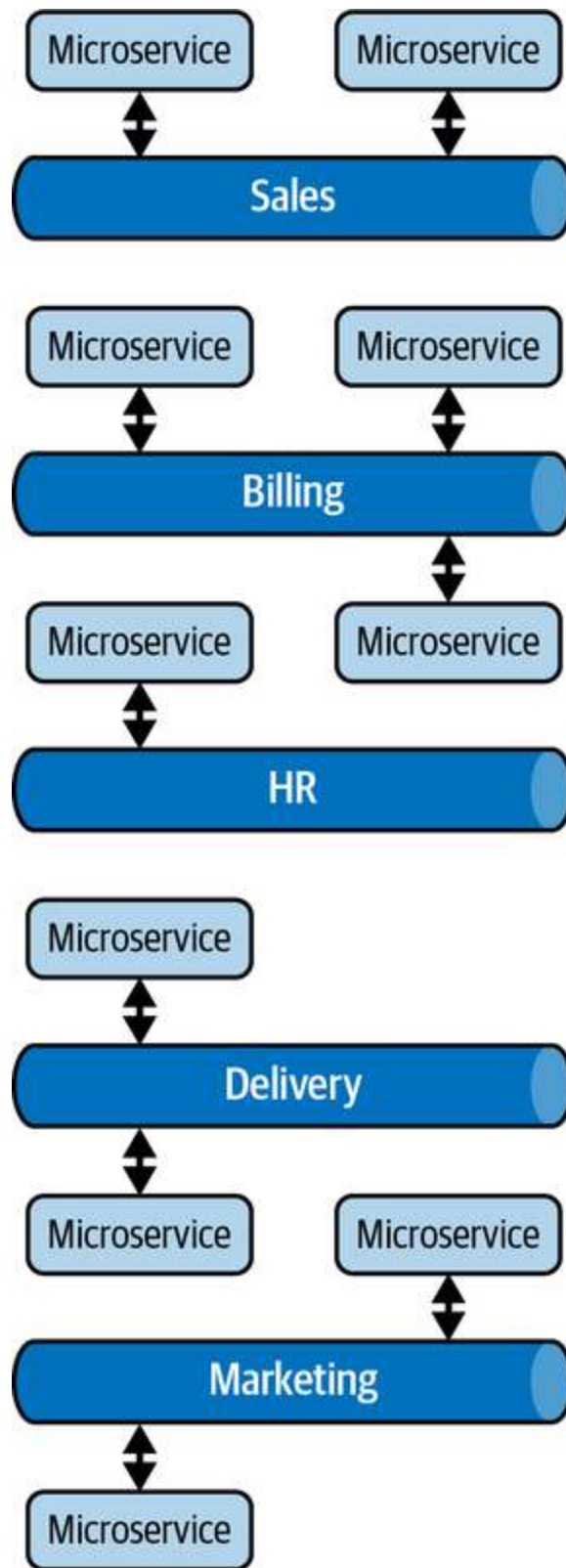
Figure 6-22. Multiple backbones
