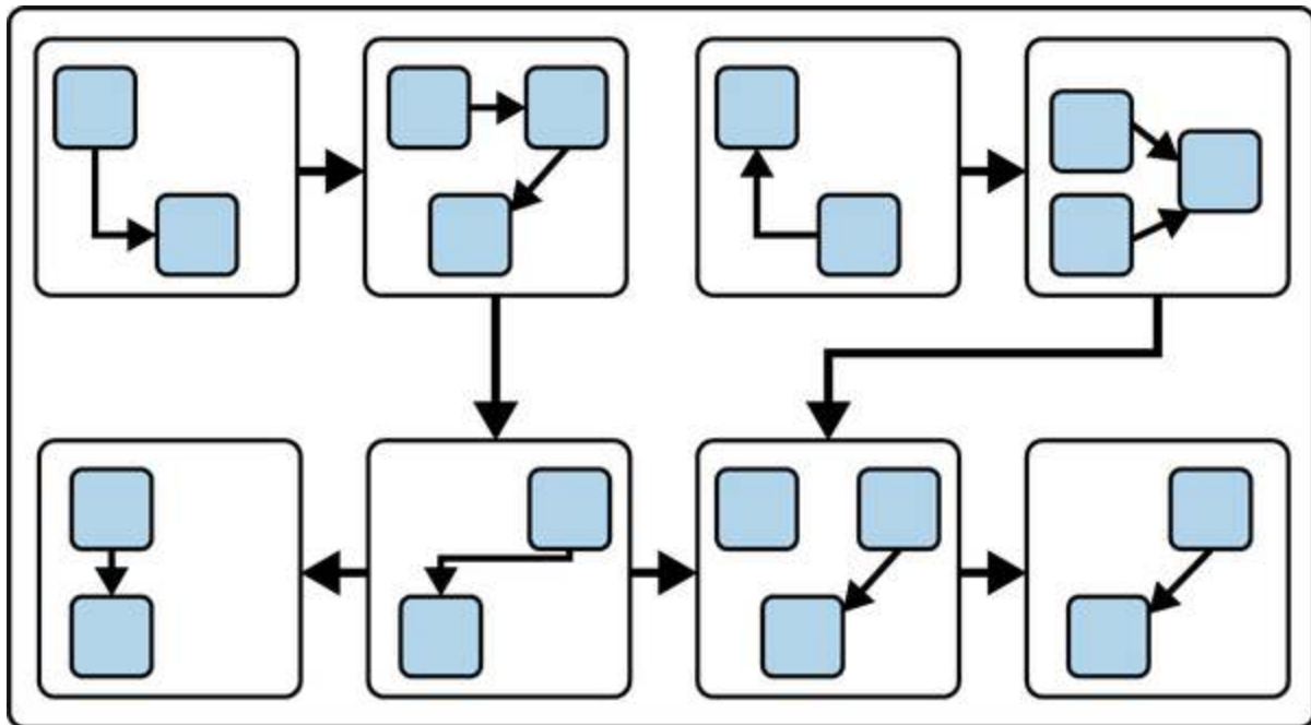
Figure 2-4. Modular Monolith
