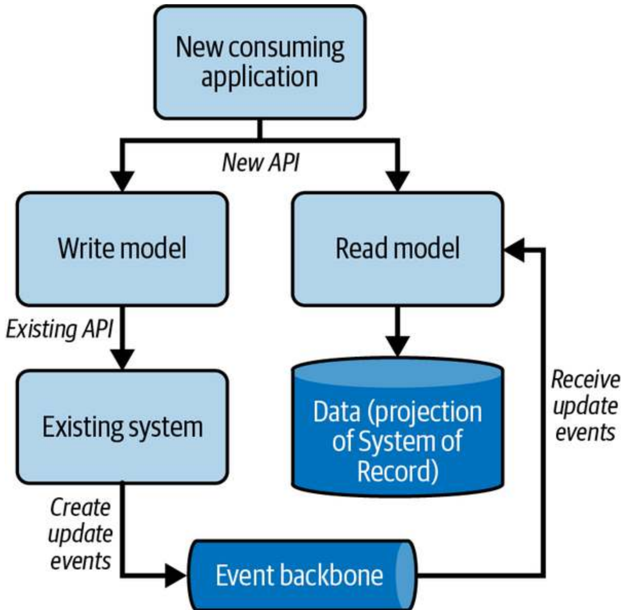
Figure 7-36. CQRS with Event Backbone
