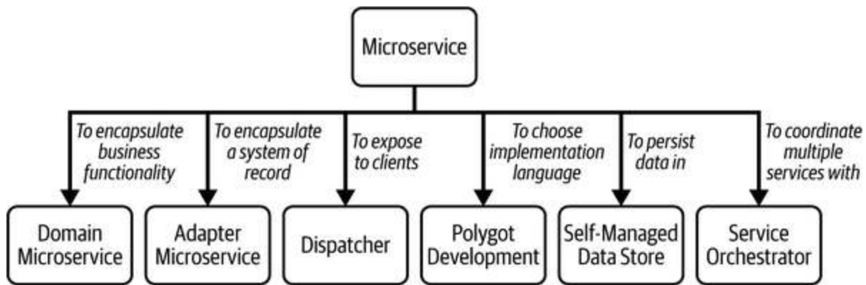
Figure 4-1. Microservices Architecture patterns
