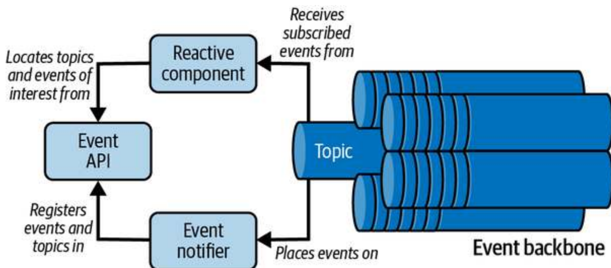
Figure 6-19. Event Backbone
