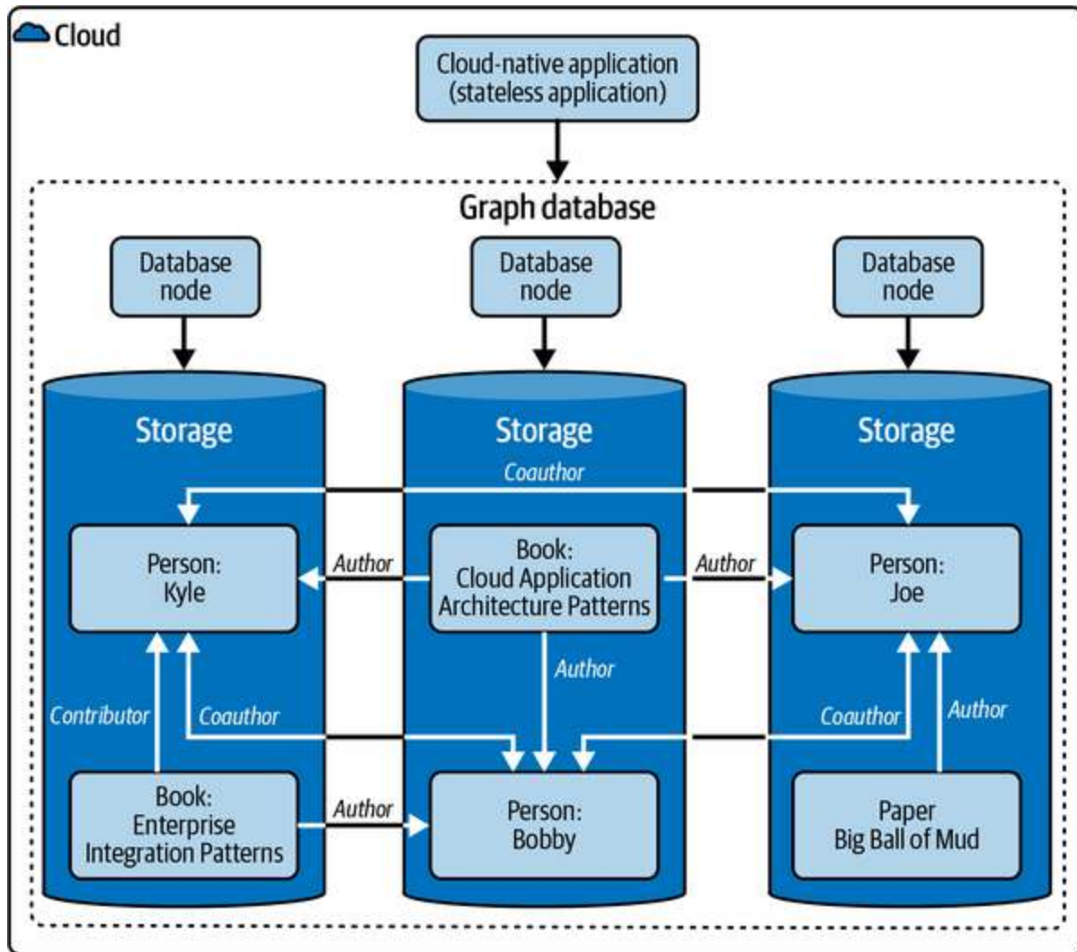
Figure 7-19. Graph Database
