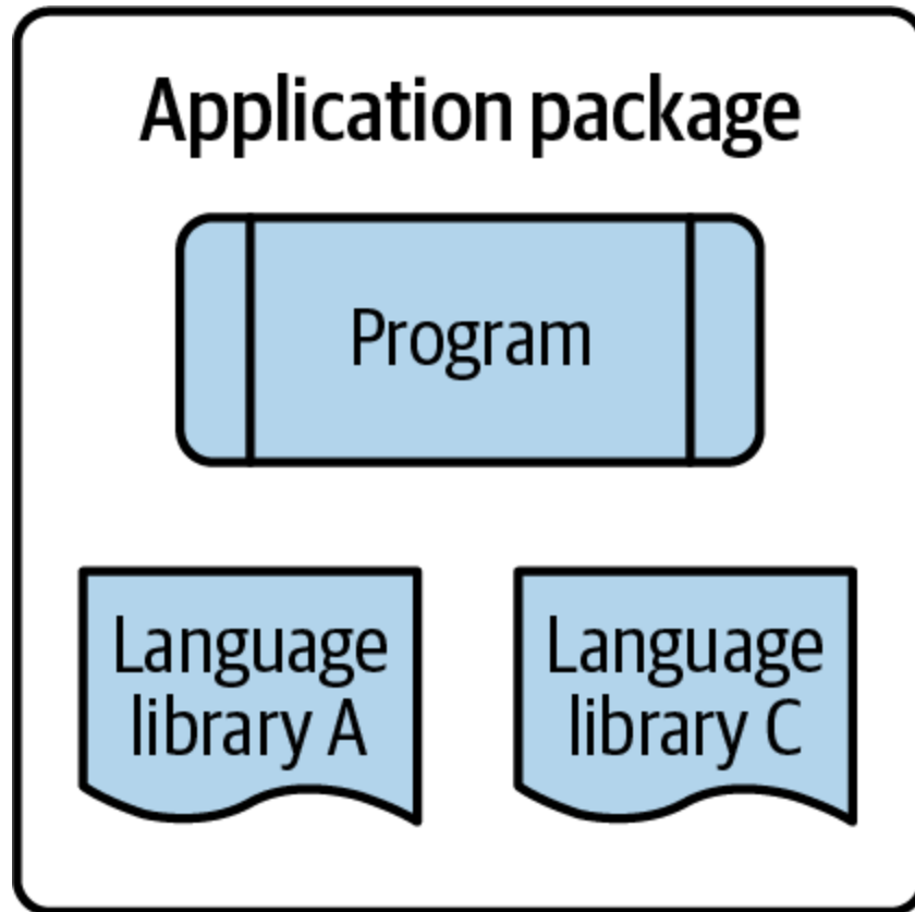
Figure 3-4. Application Package
