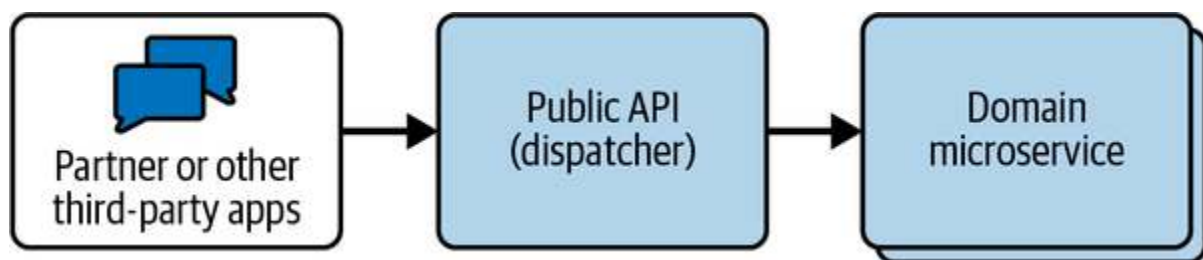
Figure 8-22. Public API
