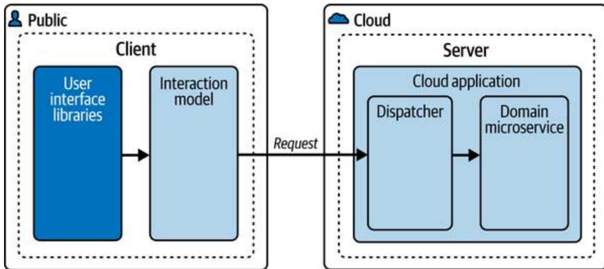
Figure 8-24. Interaction Model
