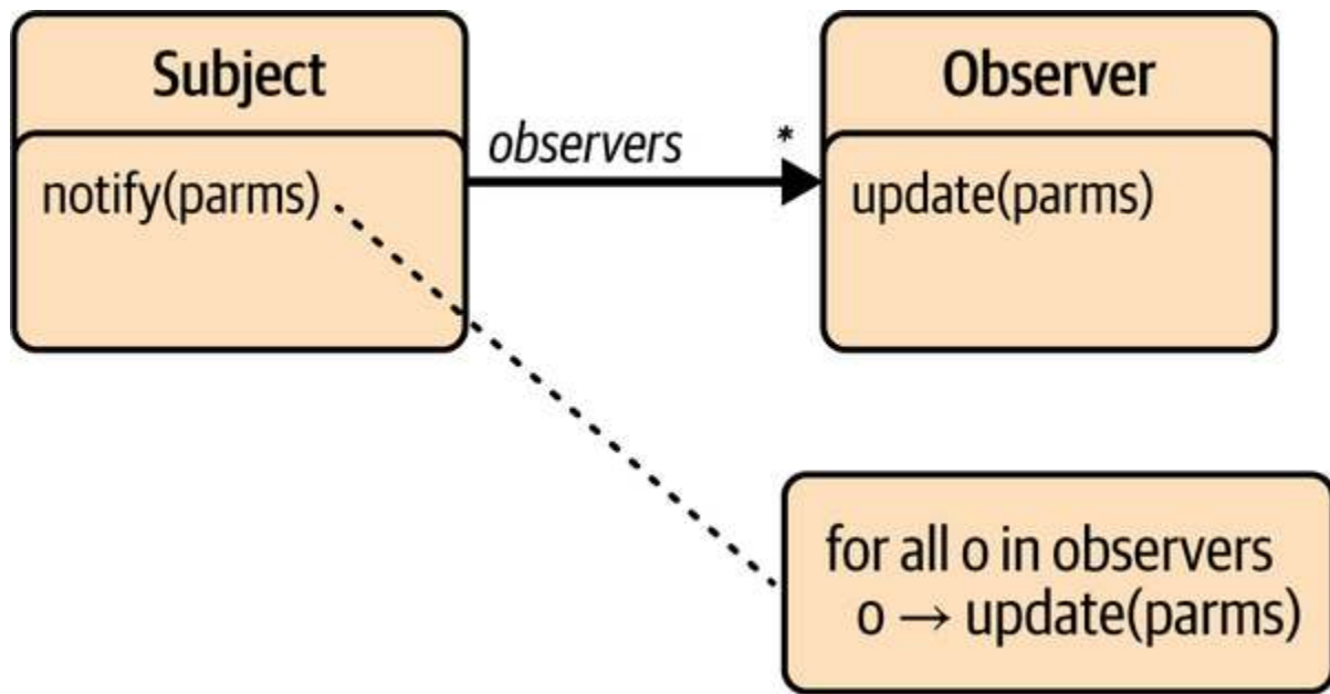
Figure 6-2. Observer pattern
