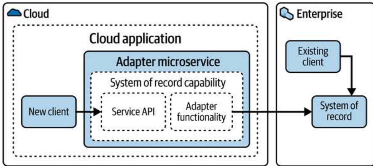
Figure 4-12. Adapter Microservice
