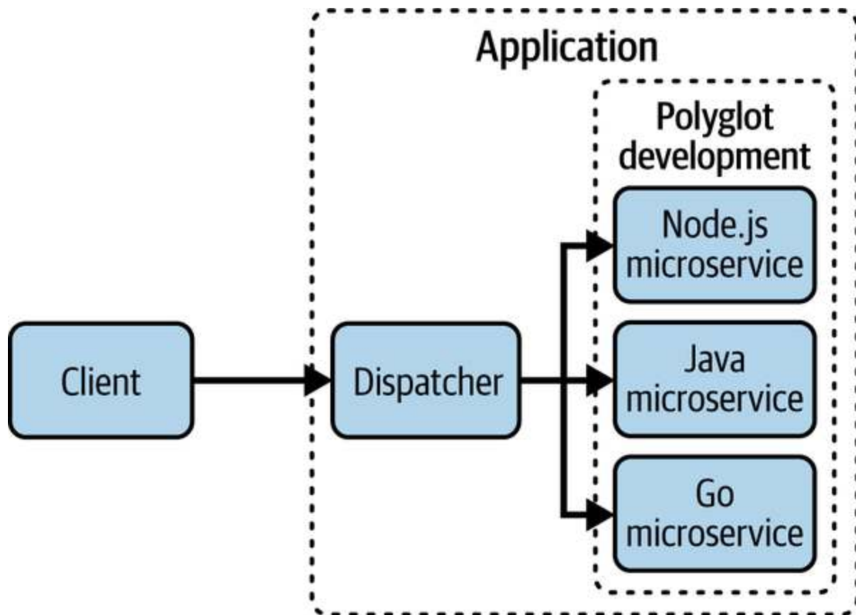
Figure 4-18. Polyglot Development
