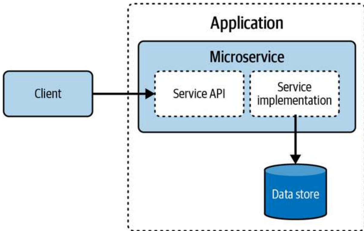
Figure 4-4. Microservice
