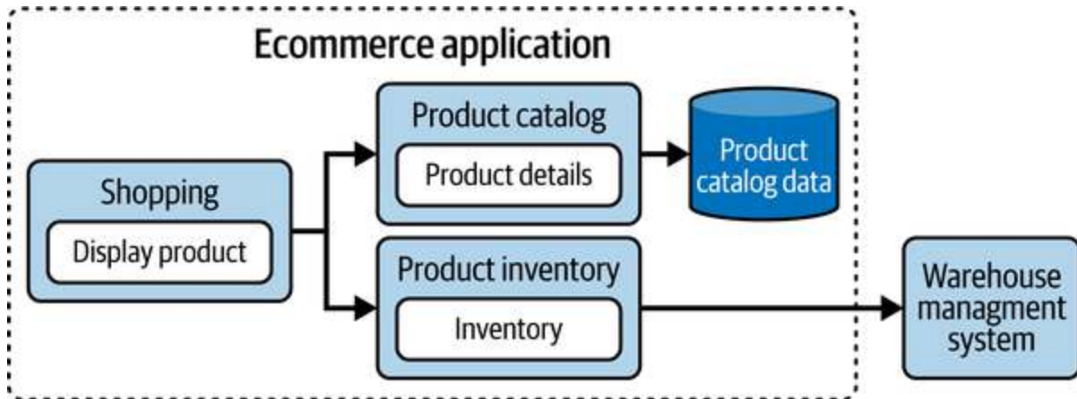
Figure 4-28. Displaying availability
