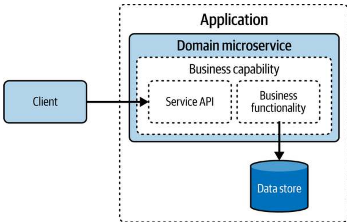
Figure 4-9. Domain Microservice
