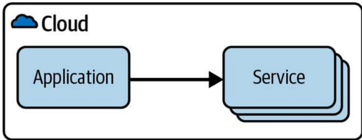
Figure 3-2. Cloud-Native Architecture
