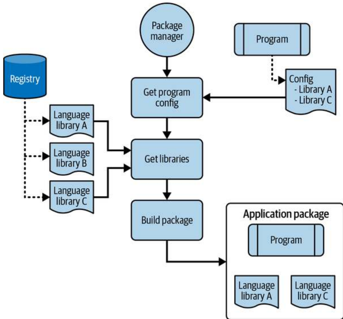
Figure 3-7. Package manager
