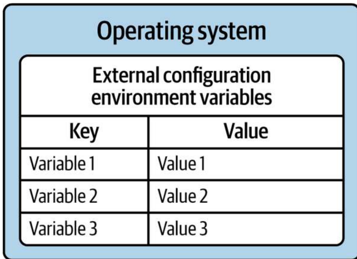
Figure 3-13. Environment variables
