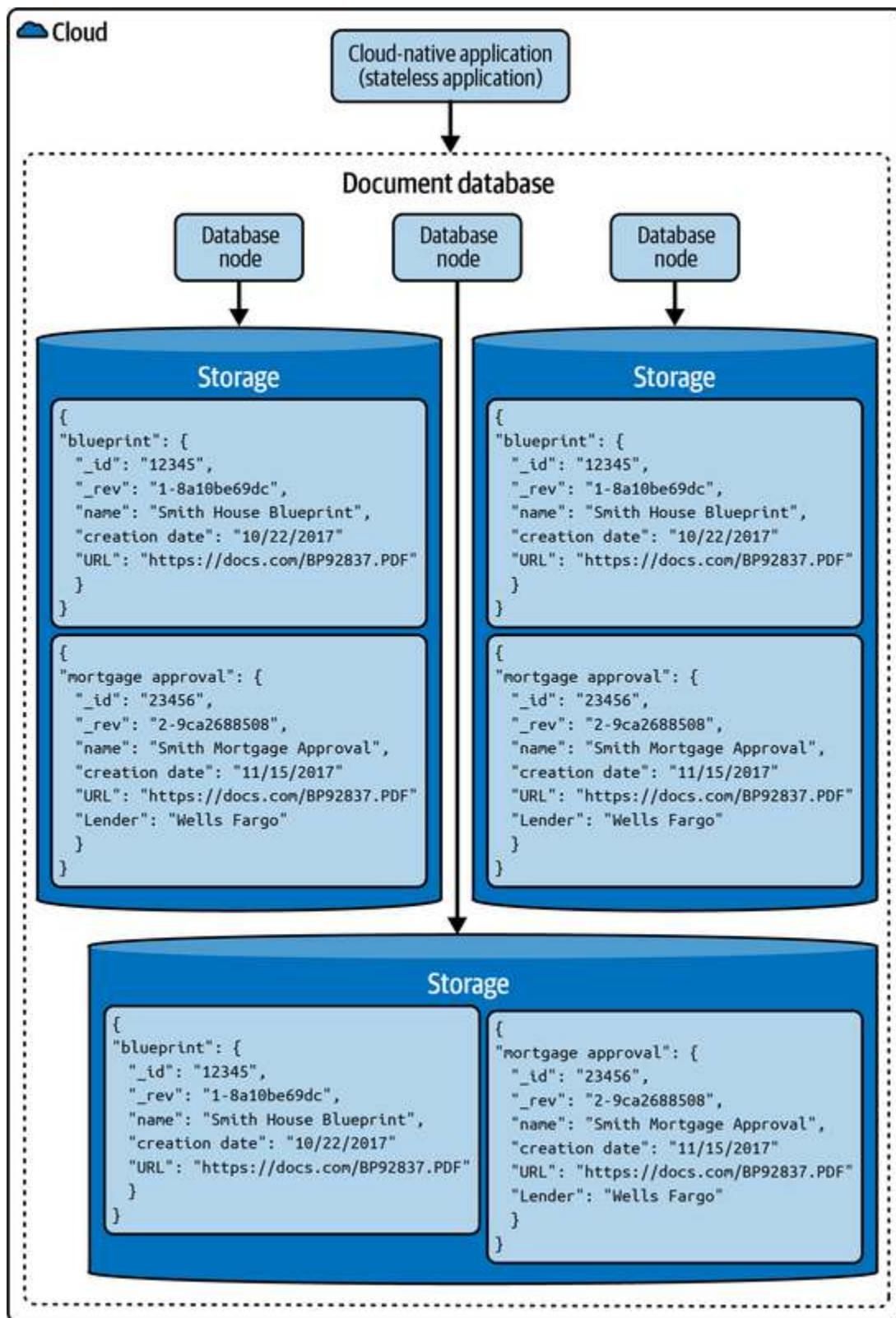
Figure 7-15. Document Database
