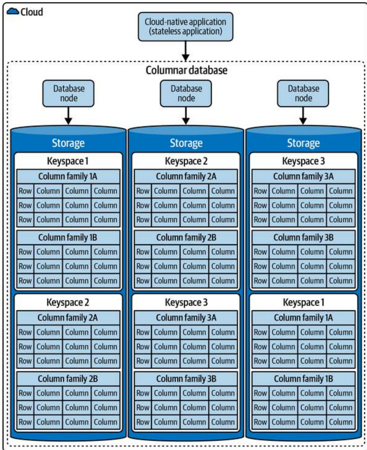
Figure 7-20. Columnar Database
