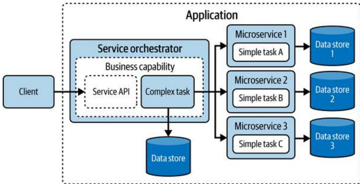
Figure 4-24. Service Orchestrator
