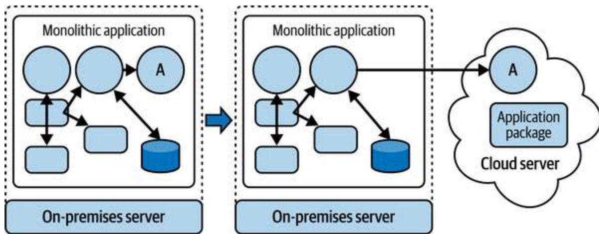
Figure 9-13. Start Small
