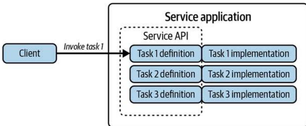
Figure 3-8. Service API
