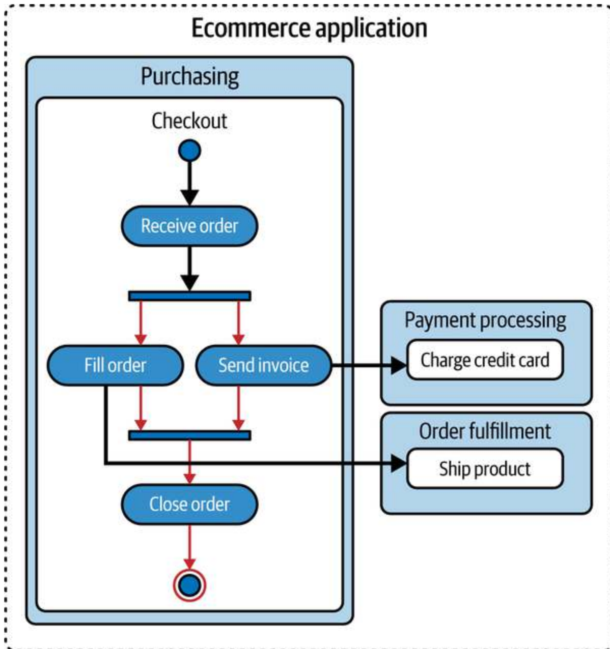
Figure 4-30. Purchasing business process
