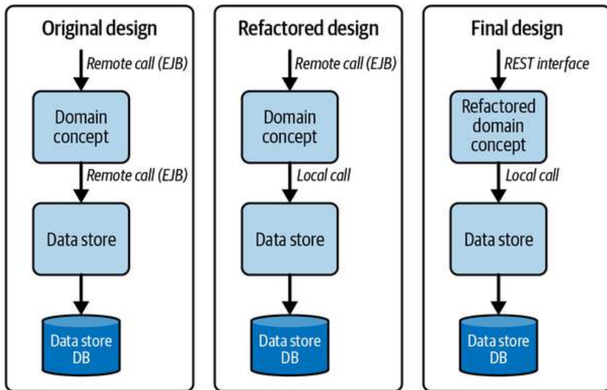
Figure 10-16. Financial services refactoring and then Extract to Microservices
