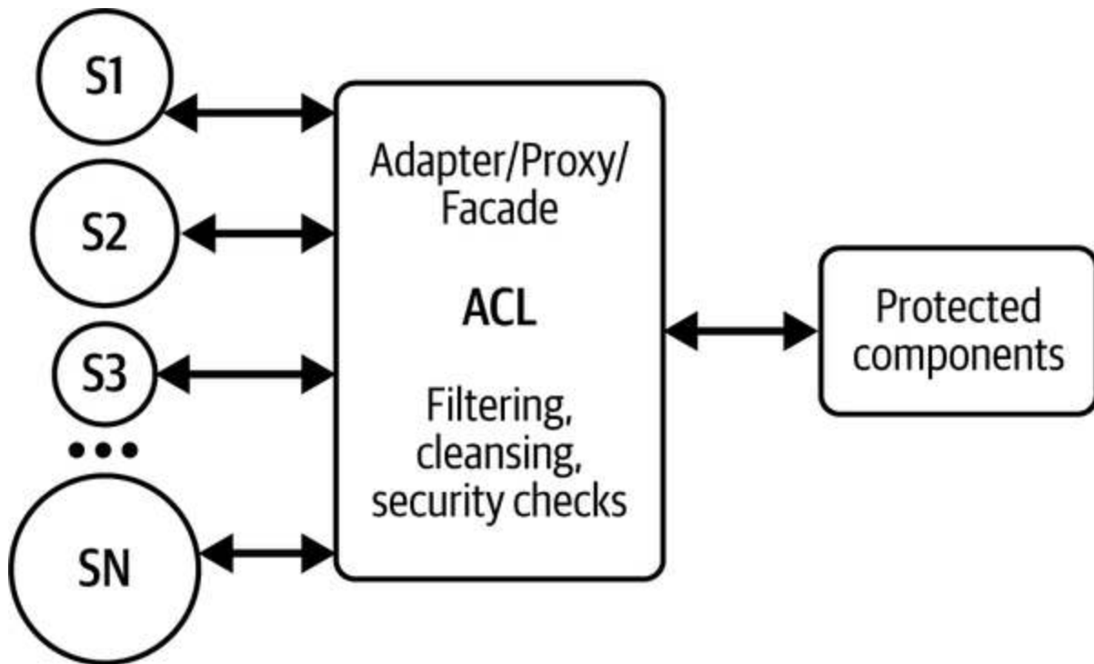
Figure 5-24. Anti-Corruption Layer protecting components
