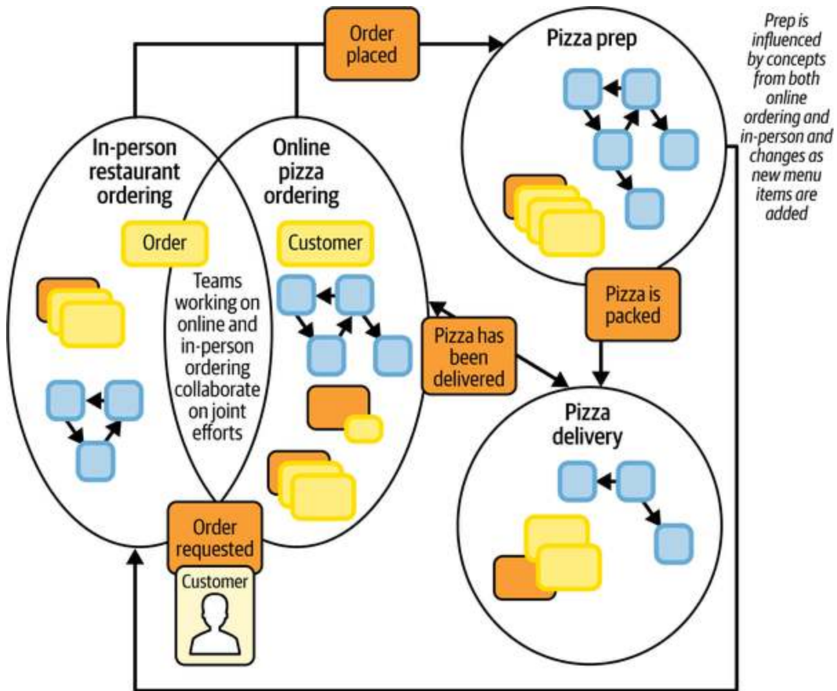
Figure 5-10. Context Map example
