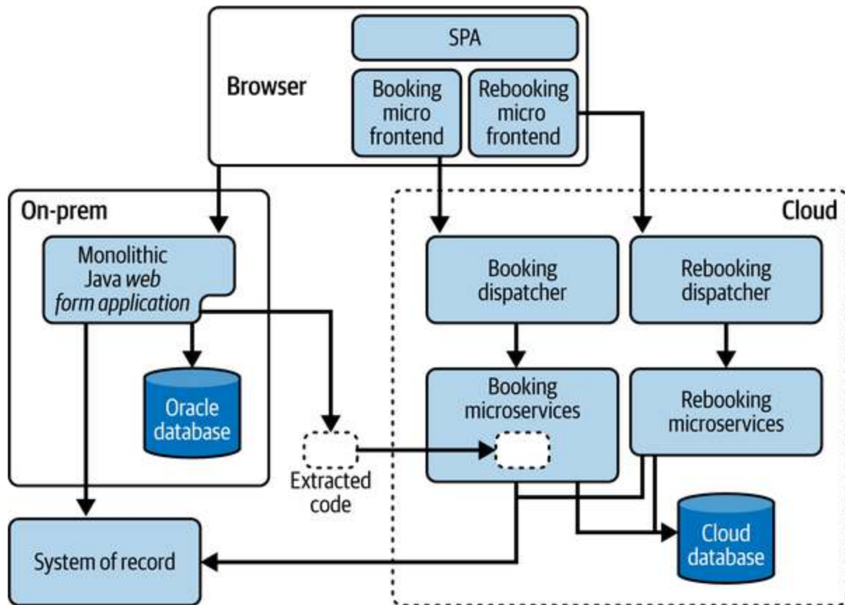
Figure 9-11. Refactoring Pave the Road example
