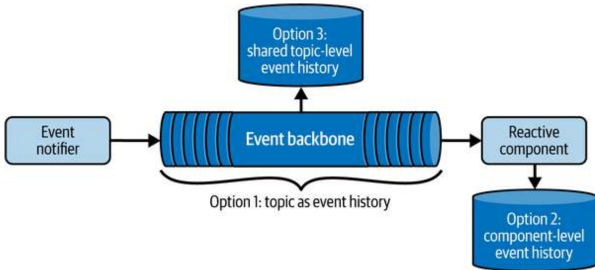
Figure 6-27. Alternatives for Event Sourcing
