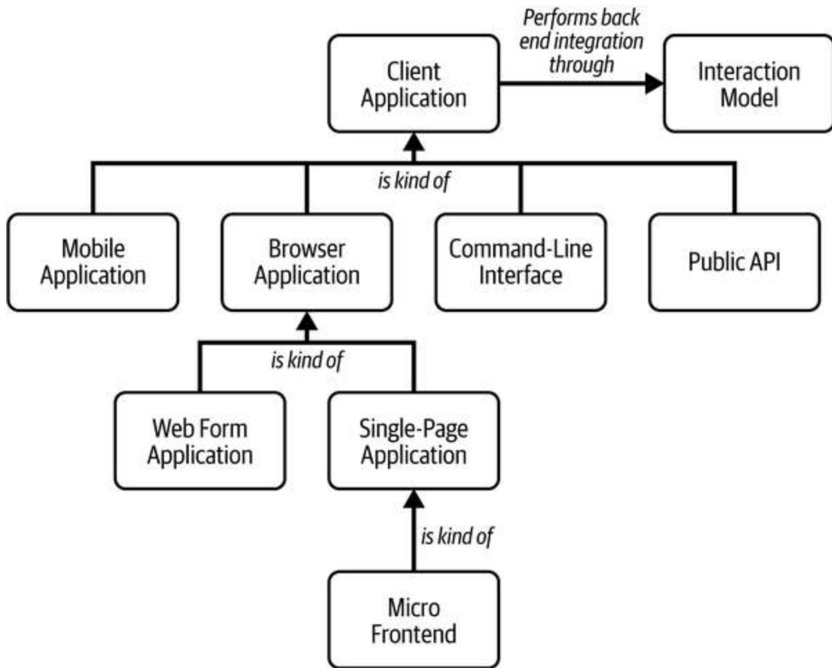
Figure 8-5. Client Application patterns
