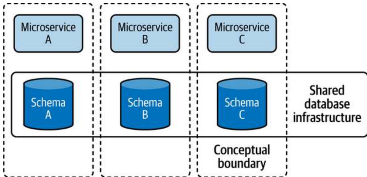
Figure 7-26. Schema per service
