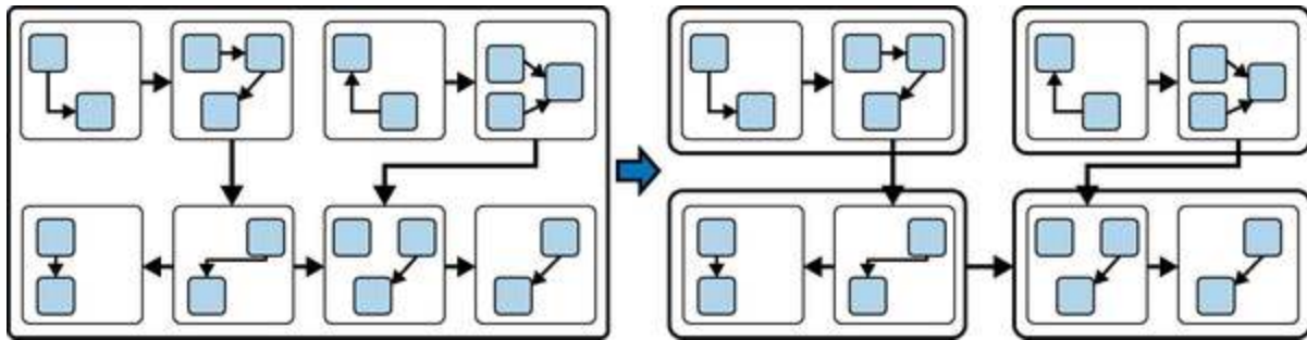
Figure 2-11. Modular Monolith to Distributed Architecture evolution
