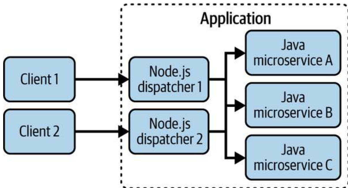
Figure 4-20. Polyglot Node.js Dispatchers with Java Microservices
