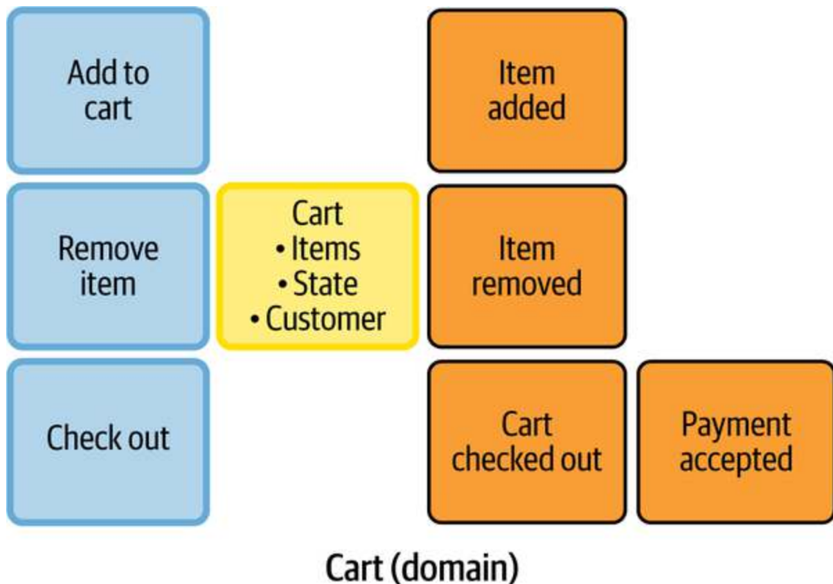
Figure 5-22. Cart Bounded Context
