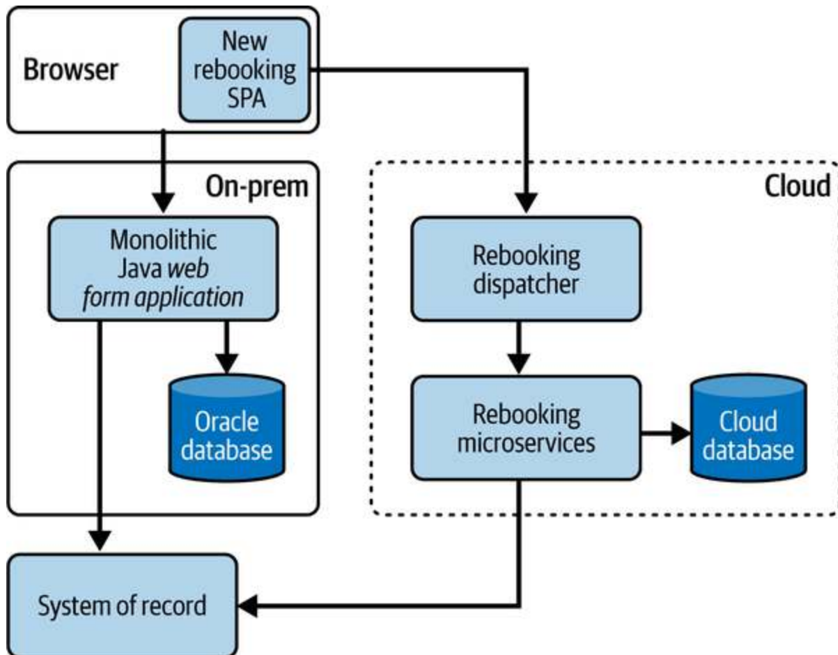
Figure 9-10. Start Small example with rebooking
