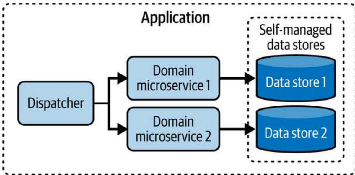
Figure 4-21. Self-Managed Data Stores
