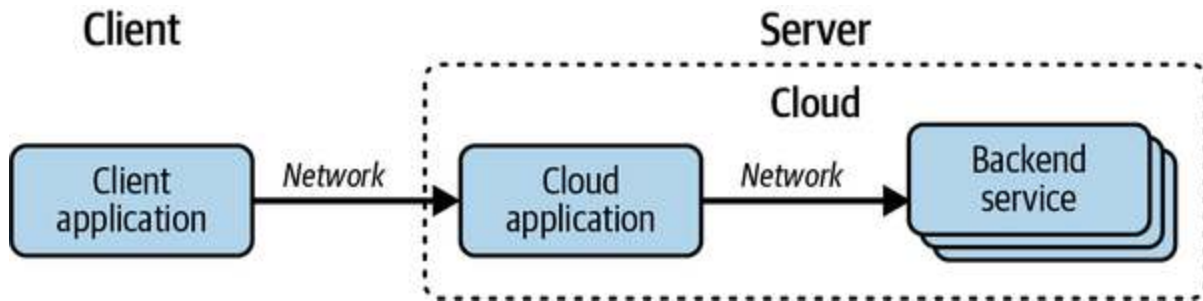
Figure I-4. Cloud-native application structure
