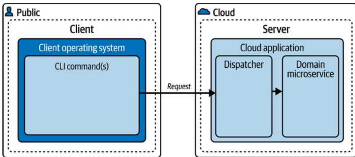
Figure 8-20. Command-Line Interface (CLI)
