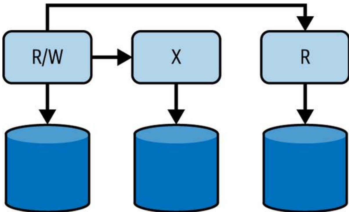
Figure 7-4. Leader-follower with read replicas topology
