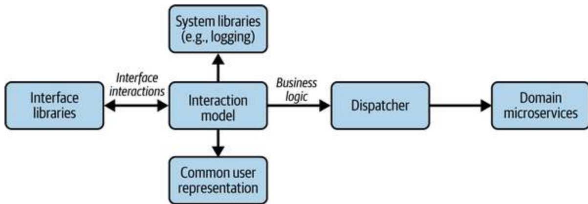
Figure 8-25. Interaction Model Relation to common code
