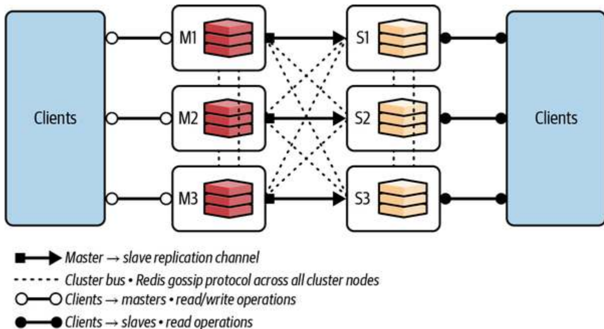
Figure 7-10. Redis grid cluster architecture
