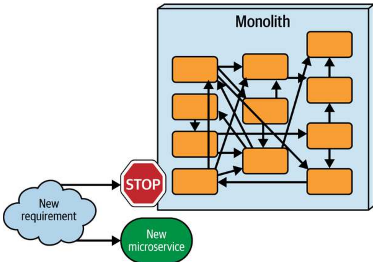
Figure 10-5. Microservices-first directive to promote New Features as Microservices
