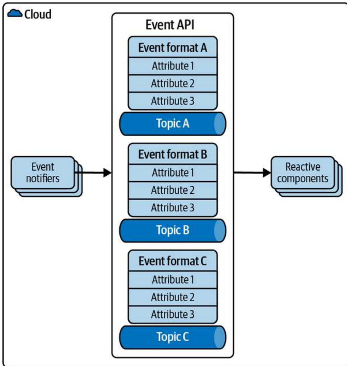
Figure 6-16. Event API
