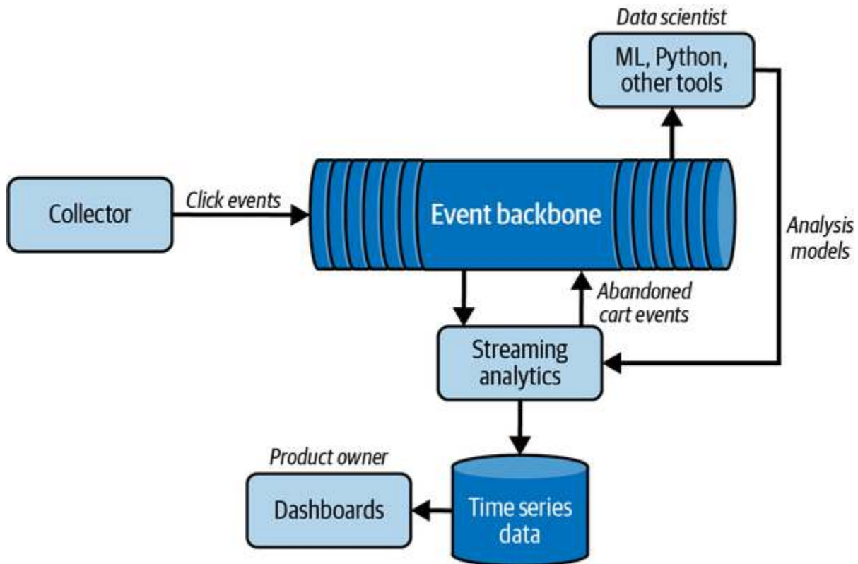
Figure 6-8. Clickstream analytics
