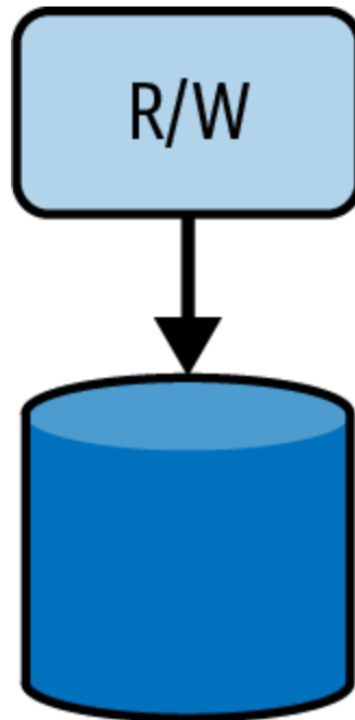
Figure 7-2. Single-server topology
