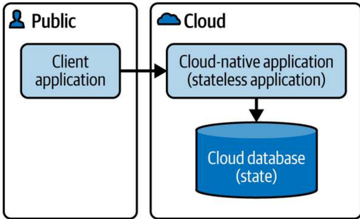
Figure 7-7. Cloud Database
