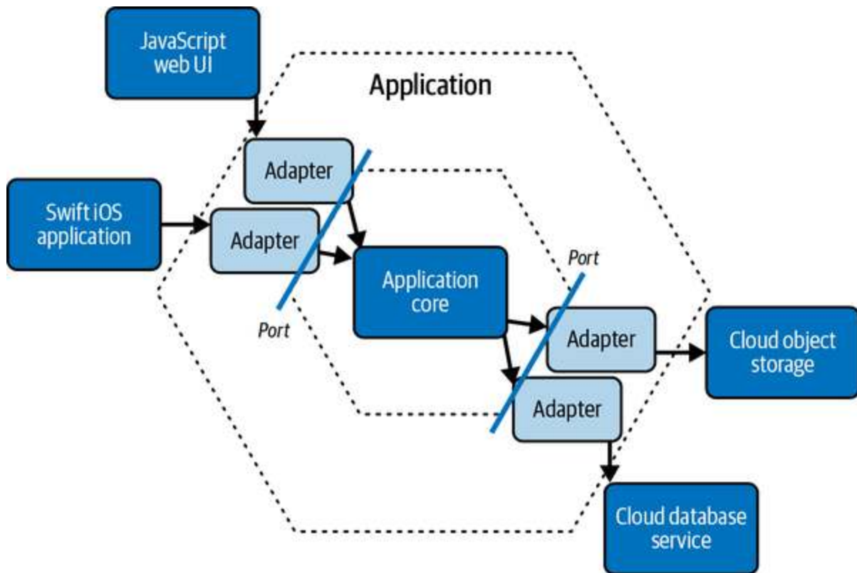
Figure 8-4. Hexagonal architecture
