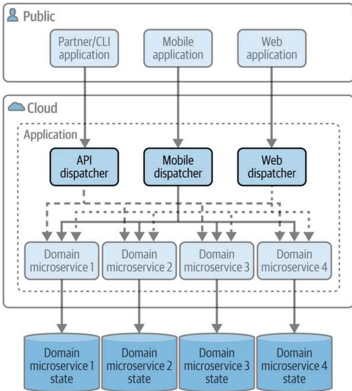
Figure 4-15. Dispatchers in Microservices Architecture
