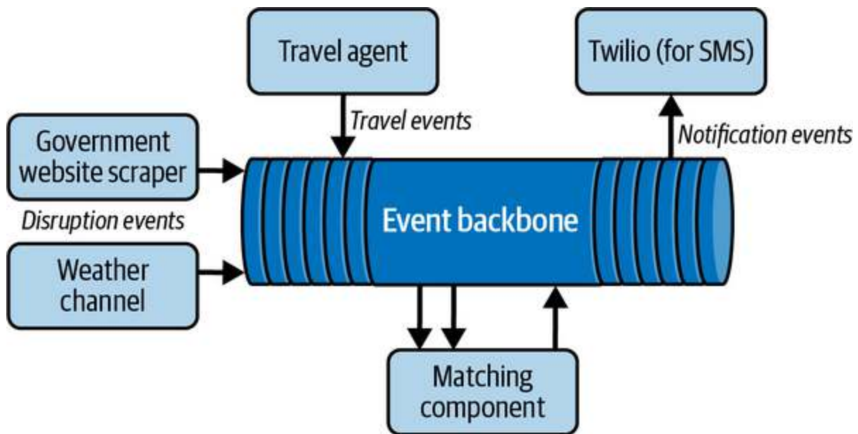
Figure 6-6. Design for employee safety notifications
