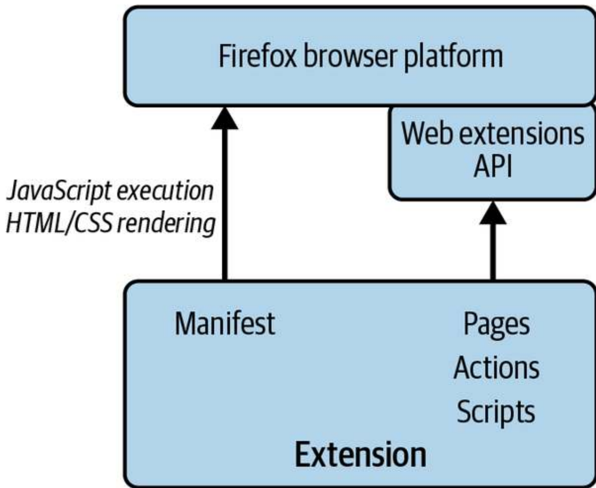
Figure 2-9. Post-2016 Firefox architecture
