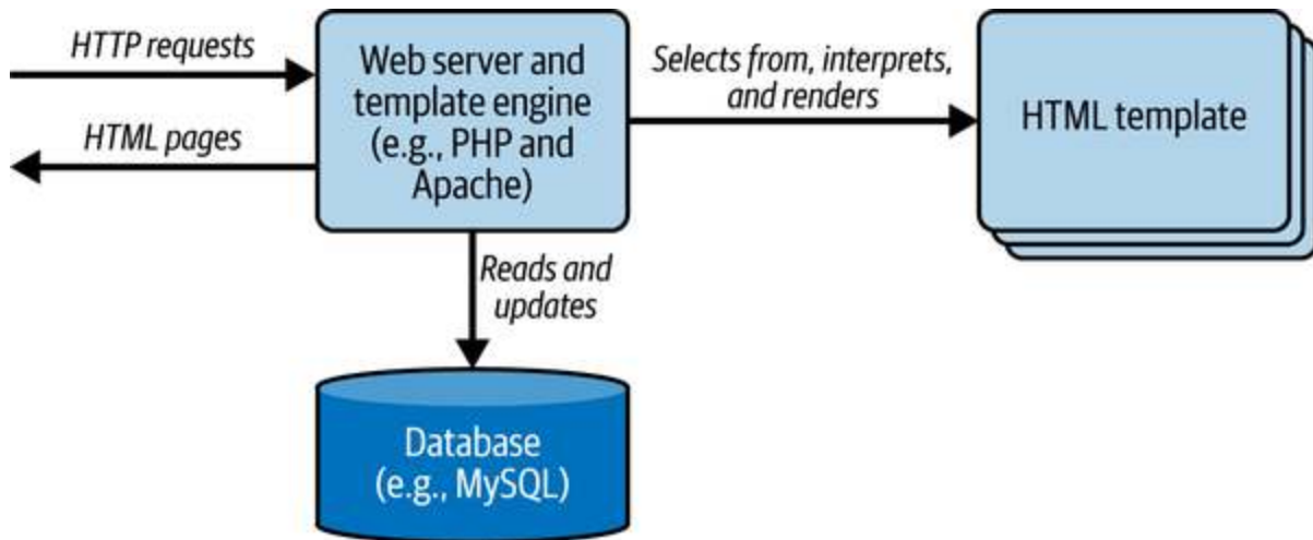
Figure 8-9. Simple templating system
