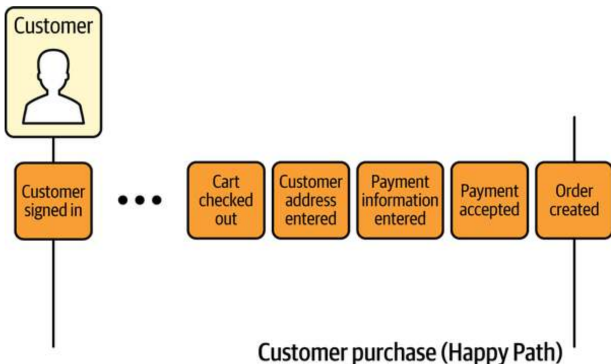
Figure 5-11. Events on a timeline with pivotal events
