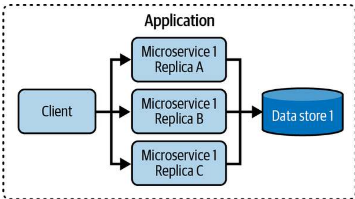
Figure 4-22. Microservice replicas share a data store
