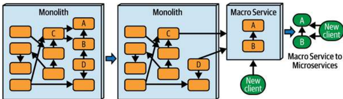
Figure 10-13. Extracting Macro Service to Refactor to Microservices
