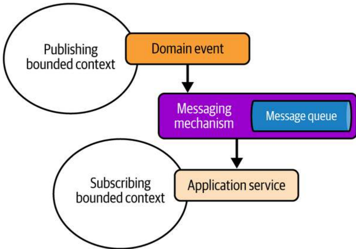
Figure 5-6. Domain Events interacting between subdomains
