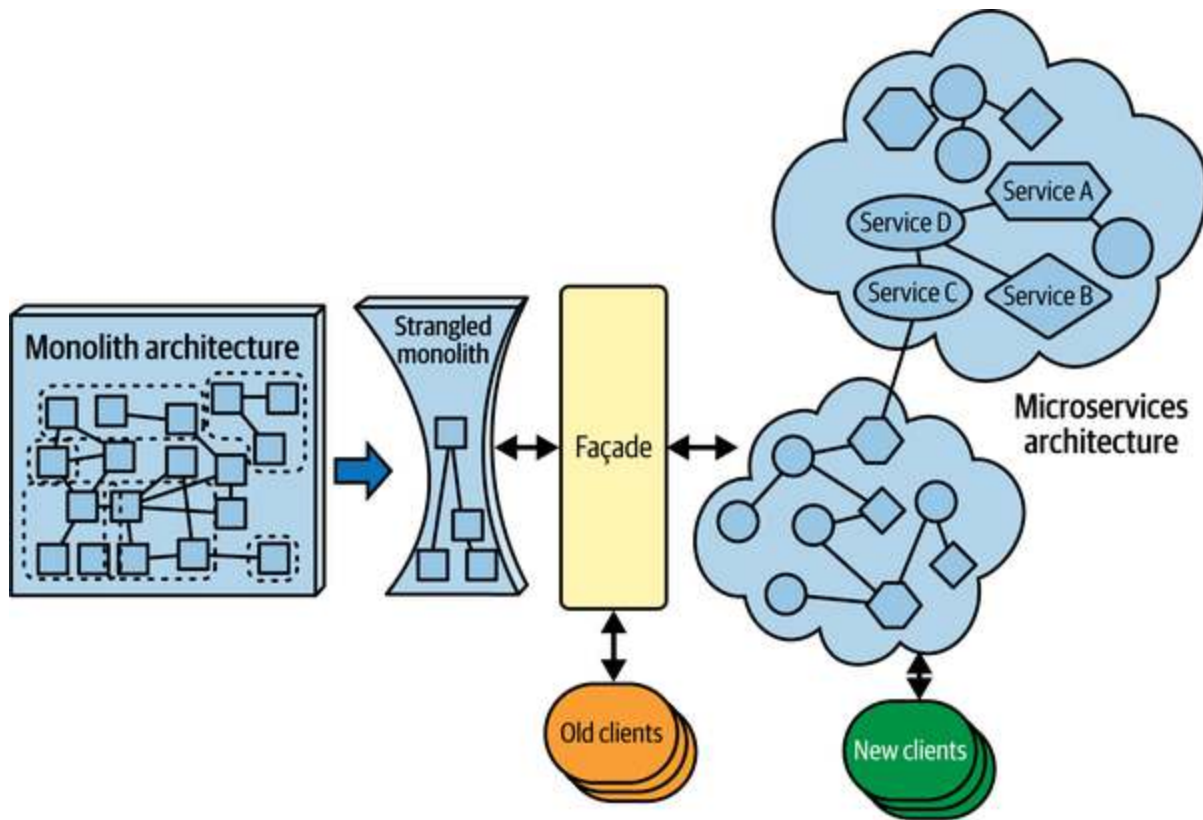
Figure 10-27. Strangled Monolith
