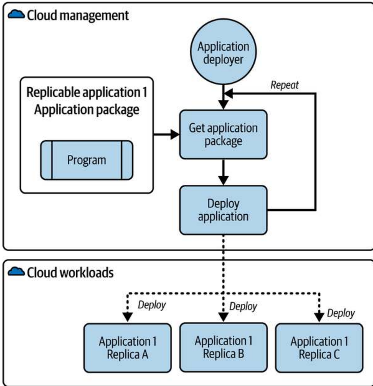
Figure 3-10. Replicable Application
