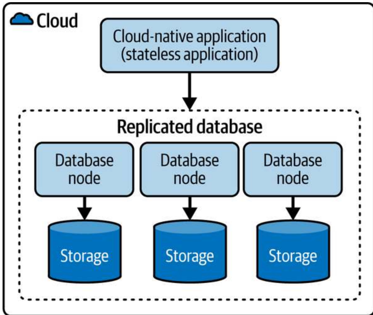
Figure 7-8. Replicated Database
