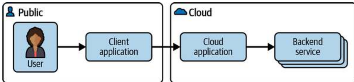
Figure 8-6. Client Application
