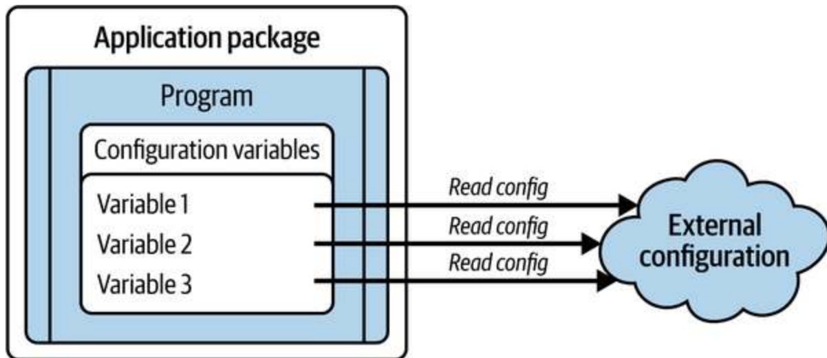
Figure 3-12. External Configuration
