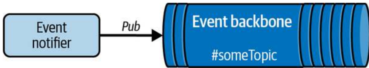
Figure 6-14. Event Notifier
