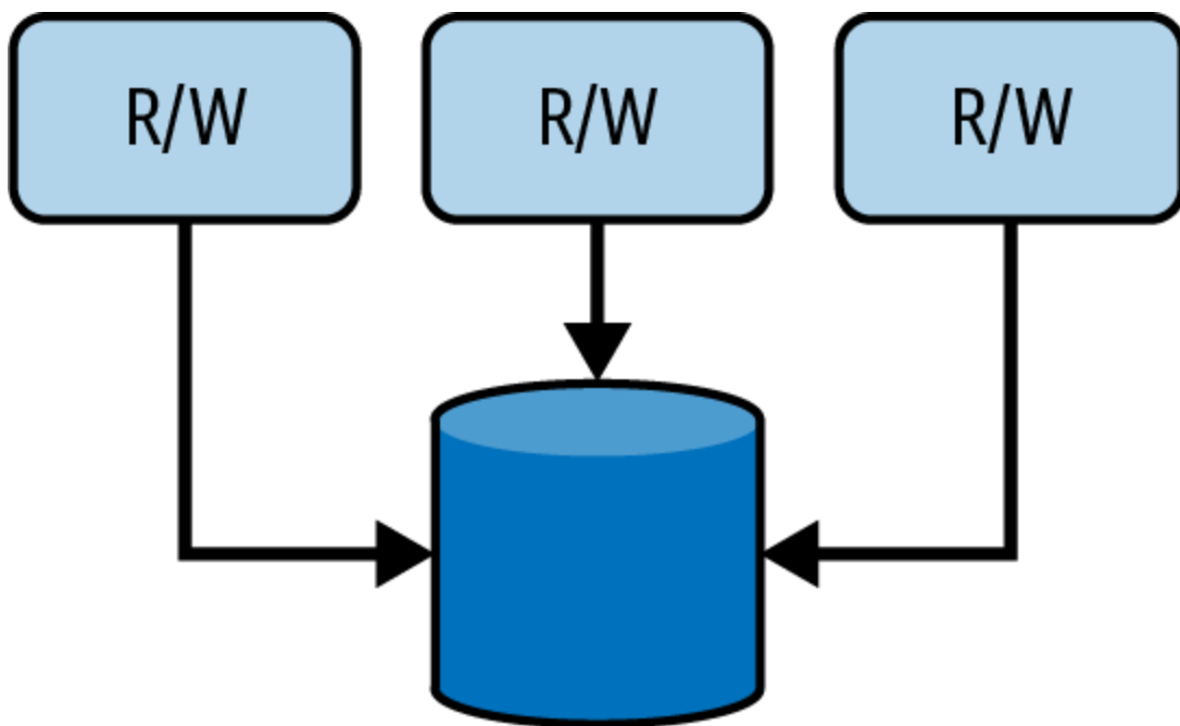
Figure 7-5. Shared-storage topology
