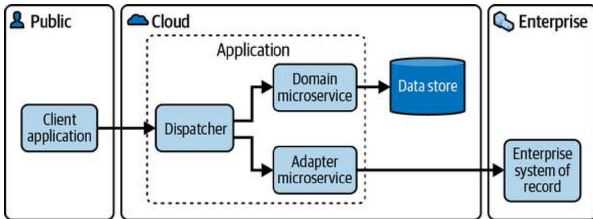
Figure 4-5. Microservices application
