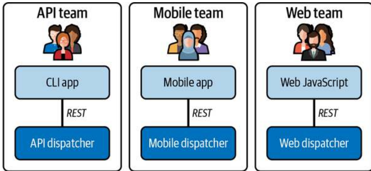
Figure 4-16. Dispatcher teams
