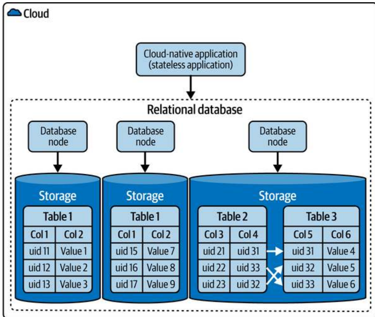
Figure 7-14. Relational Database
