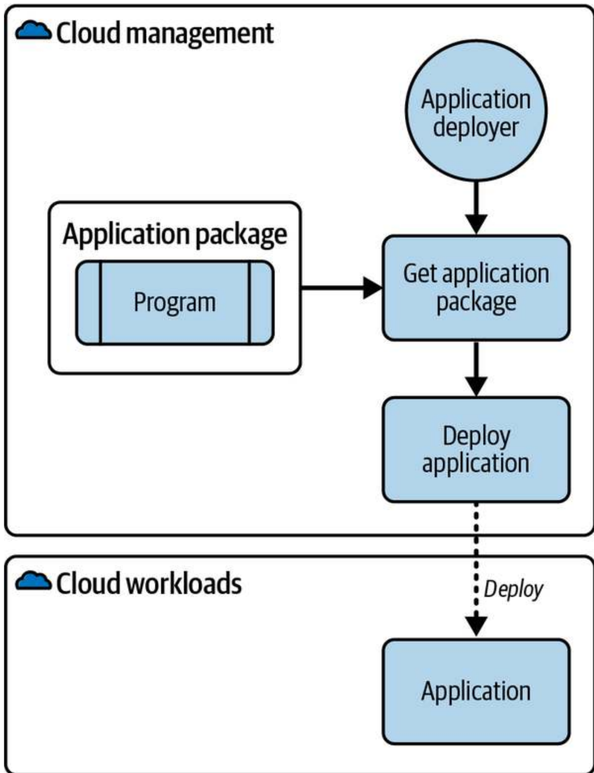
Figure 3-5. Service API
