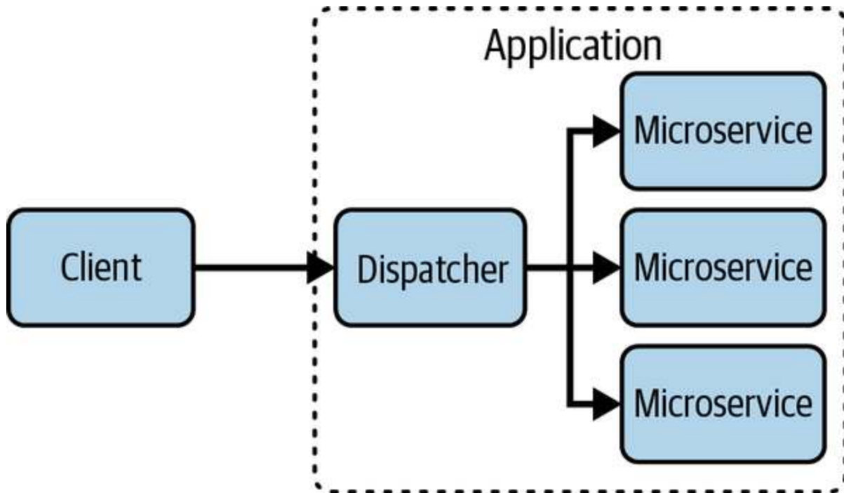
Figure 4-14. Dispatcher
