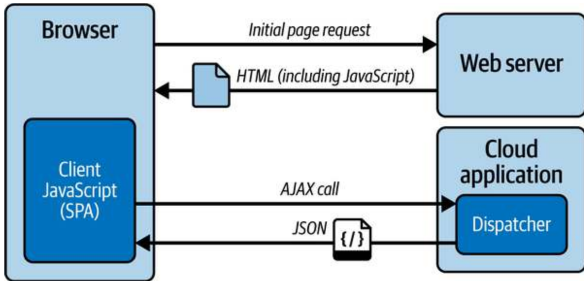
Figure 8-14. AJAX interactions
