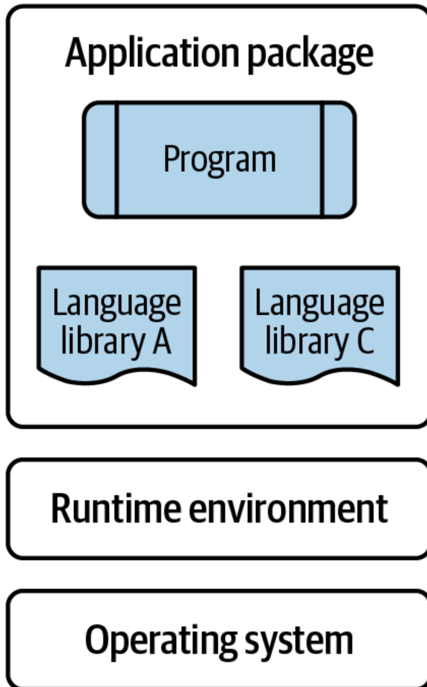
Figure 3-6. Running program
