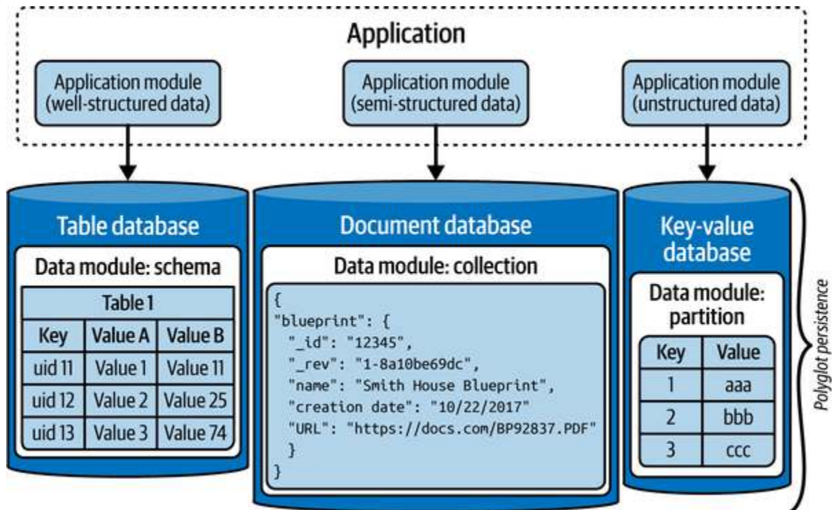
Figure 7-30. Polyglot Persistence
