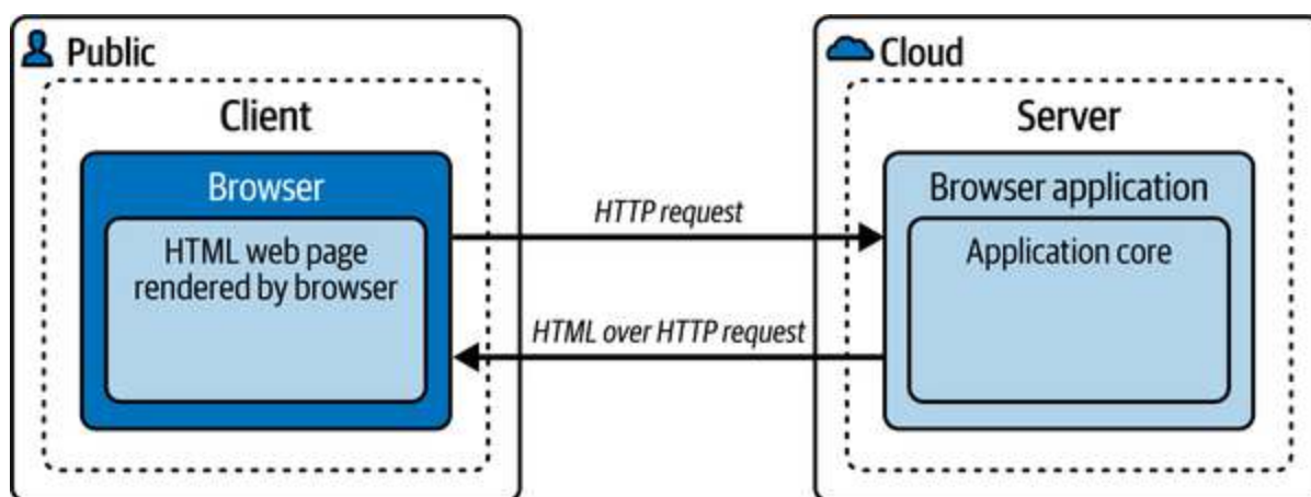
Figure 8-7. Browser Application
