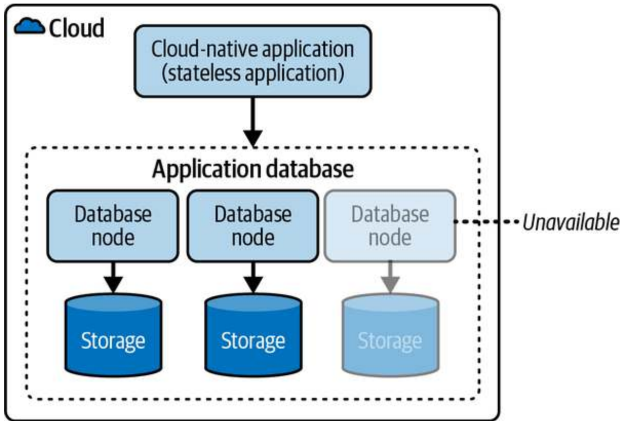
Figure 7-13. Application Database
