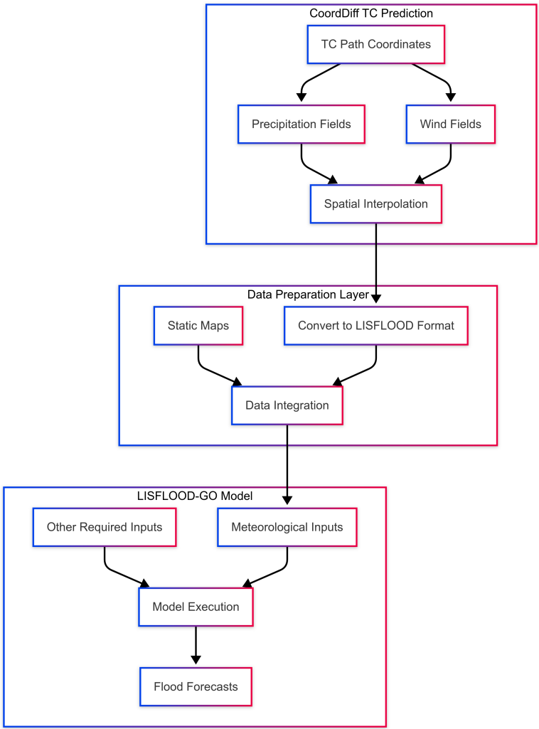
Figure 12: Connection of CorrDiff to LisFlood
