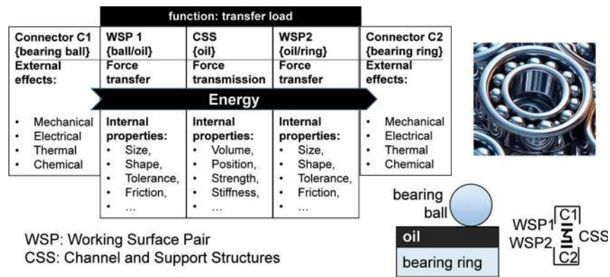
Figure 7. Entities of the interface-oriented perspective.
