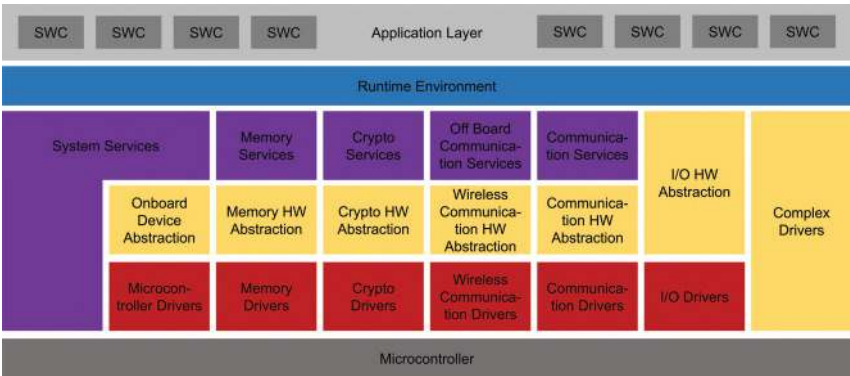
Figure 5. AUTOSAR Classic Platform software structure [22].
