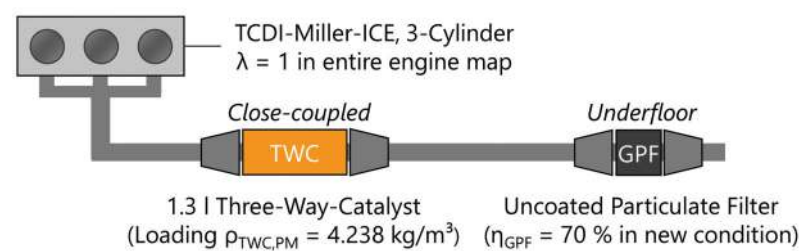
Figure 6. Setup of EU6 base exhaust aftertreatment system used for the simulation study.
