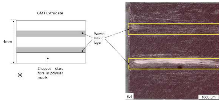
Figure 7. (a) PP-X121 F42 GMT schematic layout; (b) microscopic scan picture of PP-X121 F42 GMT.
