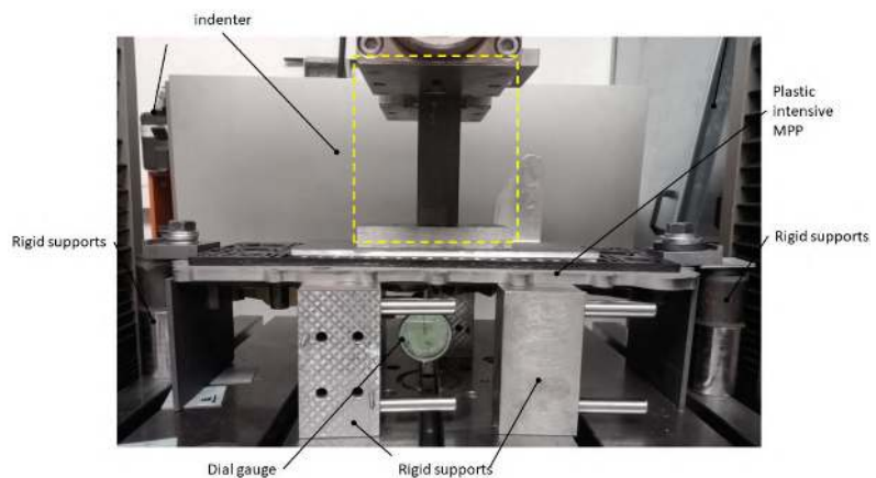
Figure 22. Test Setup for FEM verification.
