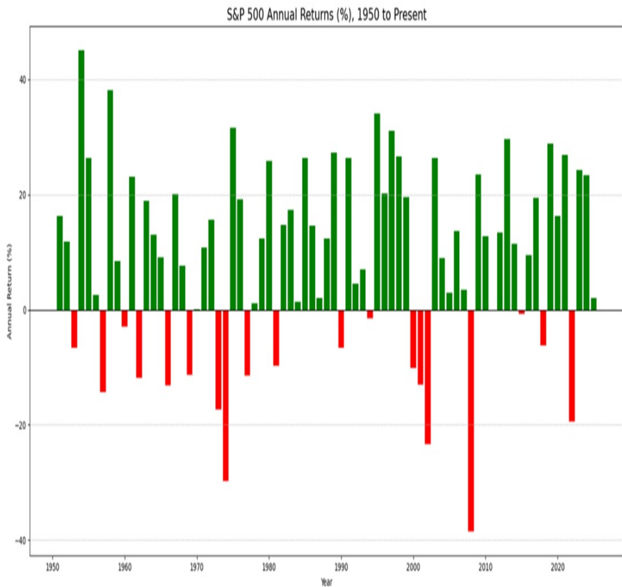
Figure 7.8 Market returns from 2050 until the present day.
