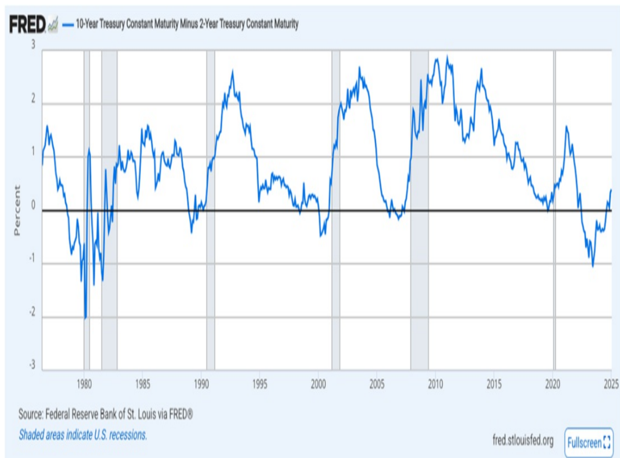
Figure 7.6 10-Year Treasury Constant Maturity Minus 2-Year Treasury Constant Maturity
