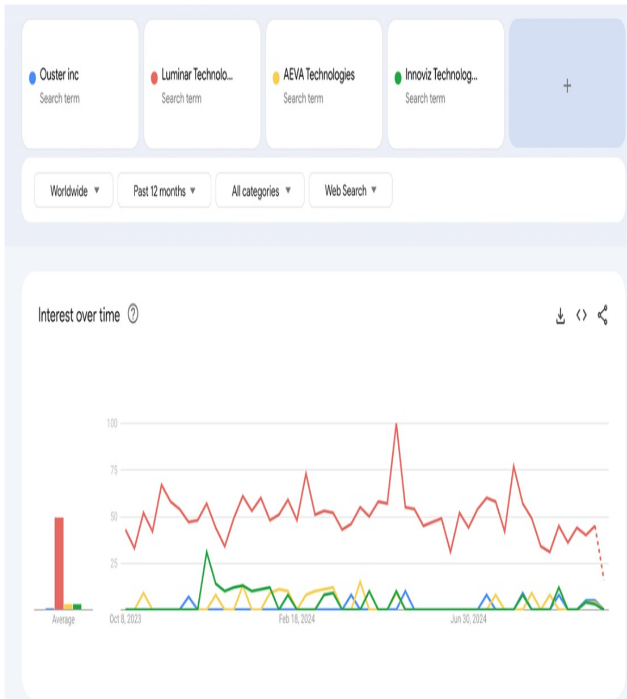
Figure 4.7 Google Trends on OUST, LAZR, AEVA, INVZ
