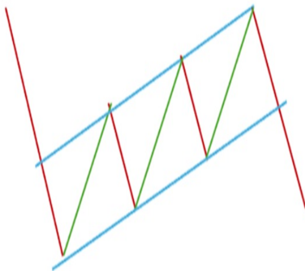
Bearish Flag Pattern
