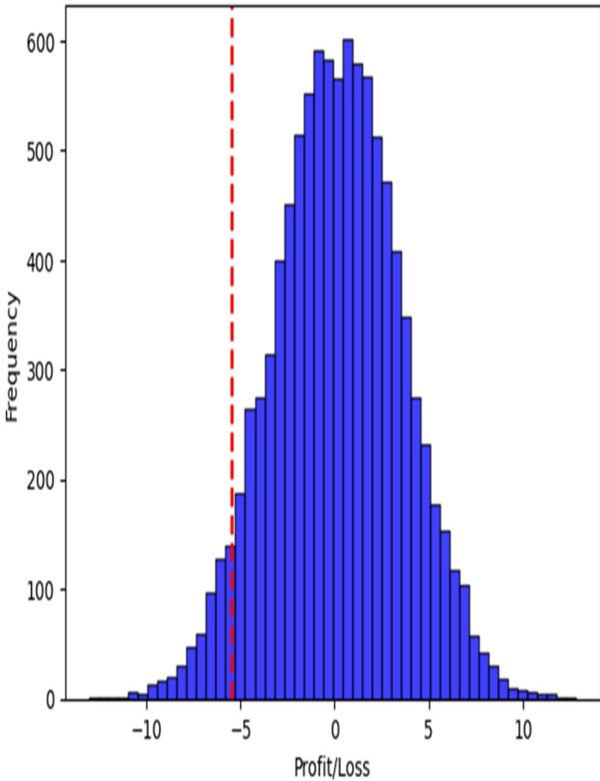
Monte Carlo Simulated P&L Distribution for AAPL
