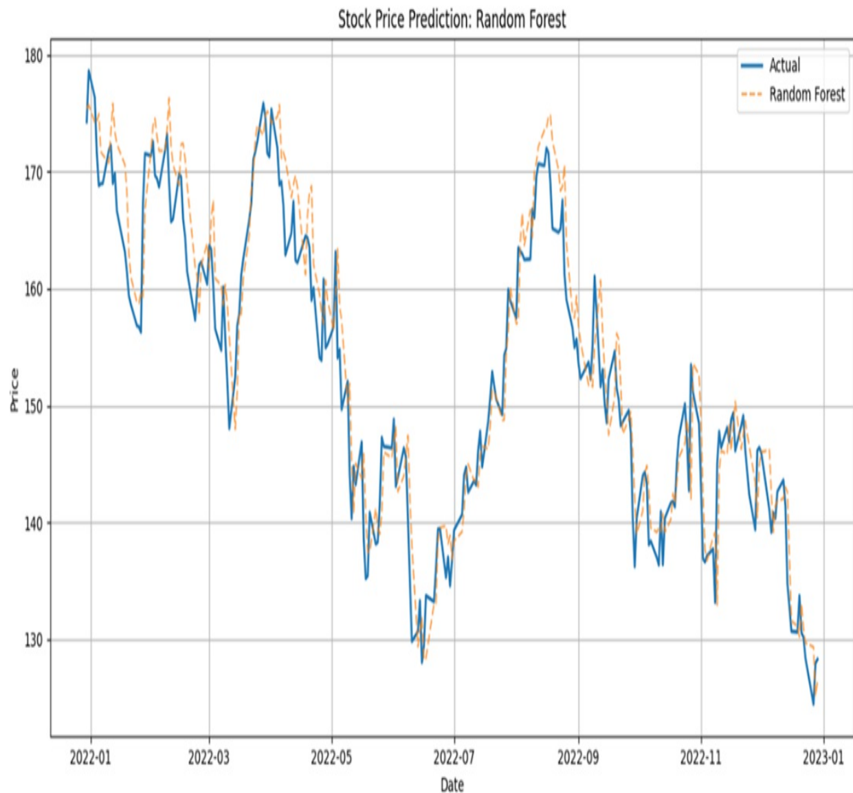
Figure 8.5 Illustrates the difference between actual and forecasted prices, showing that in some cases, the predictions are more accurate than others.
