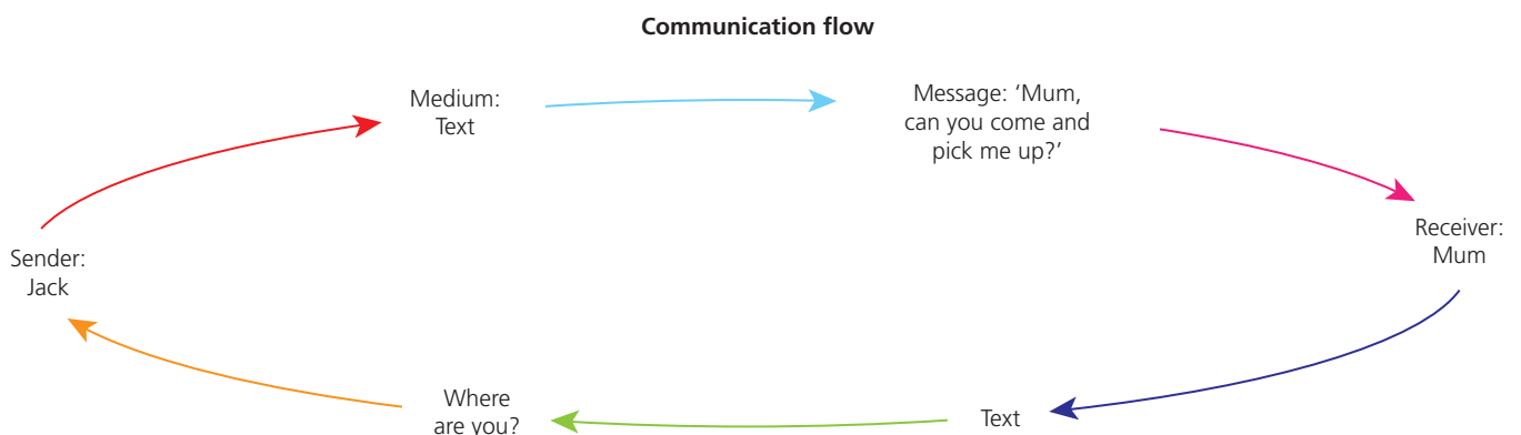
Figure 50.1 Communication model
