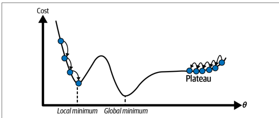
Figure 4-6. Gradient descent pitfalls
