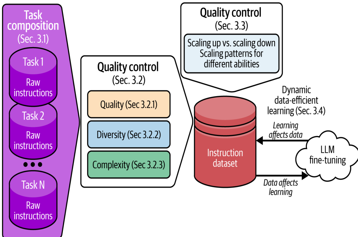
(b) Data management pipeline in the supervised fine-tuning stage of LLMs
