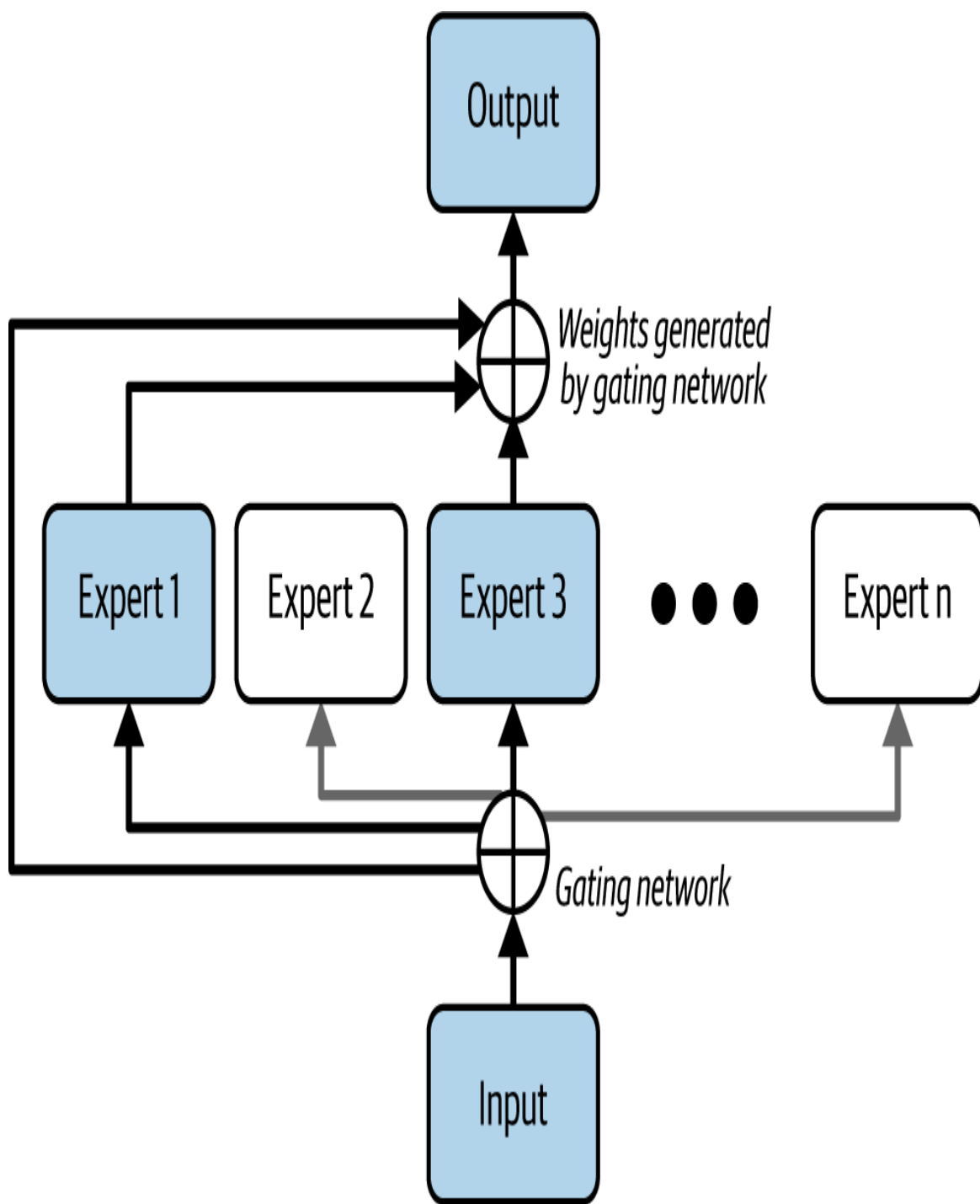
Figure 5-3. A visualization of how MoE works (source: "Mixture of Experts" )
