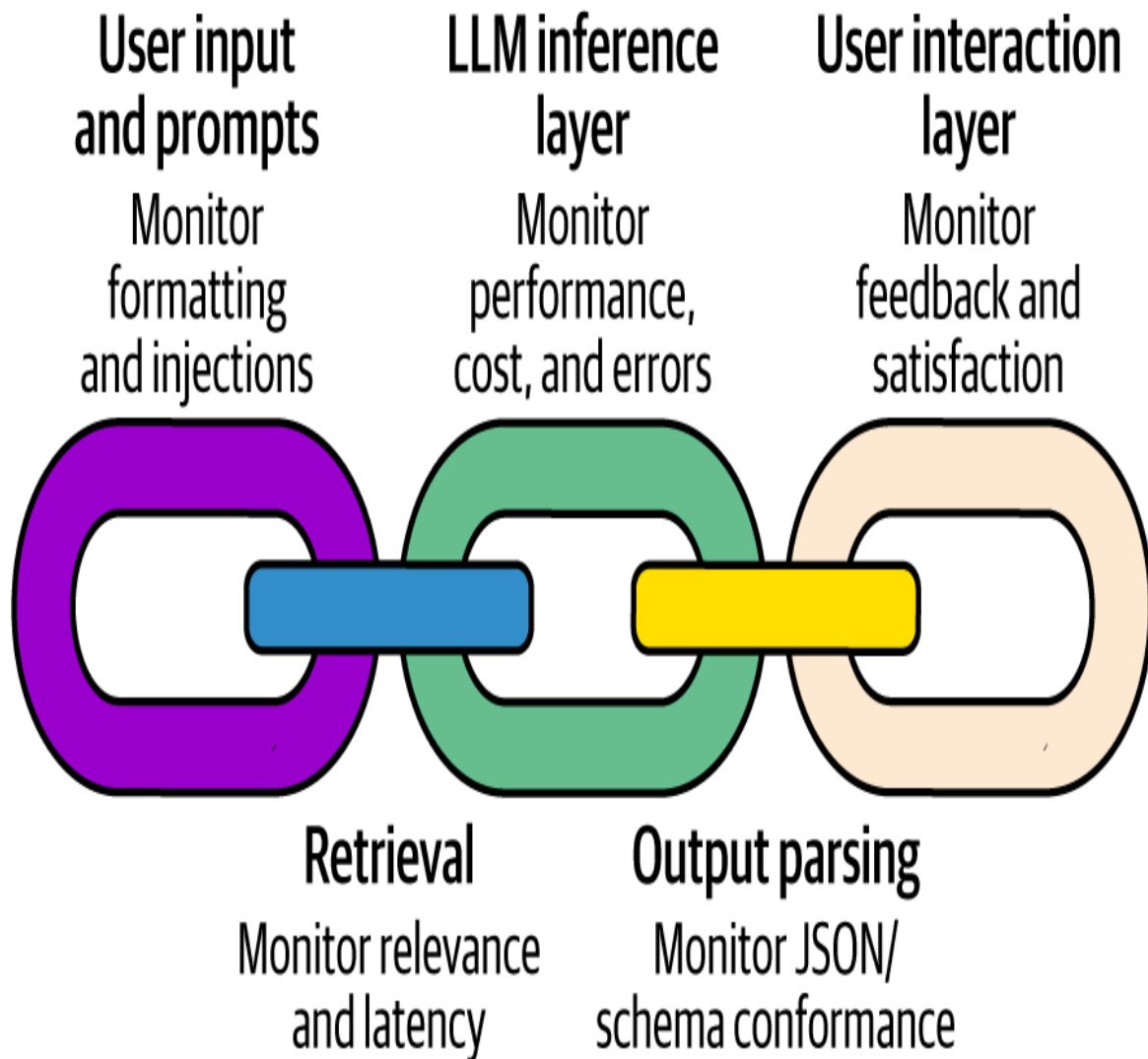
Figure 7-4. Observability pipeline for LLMs
