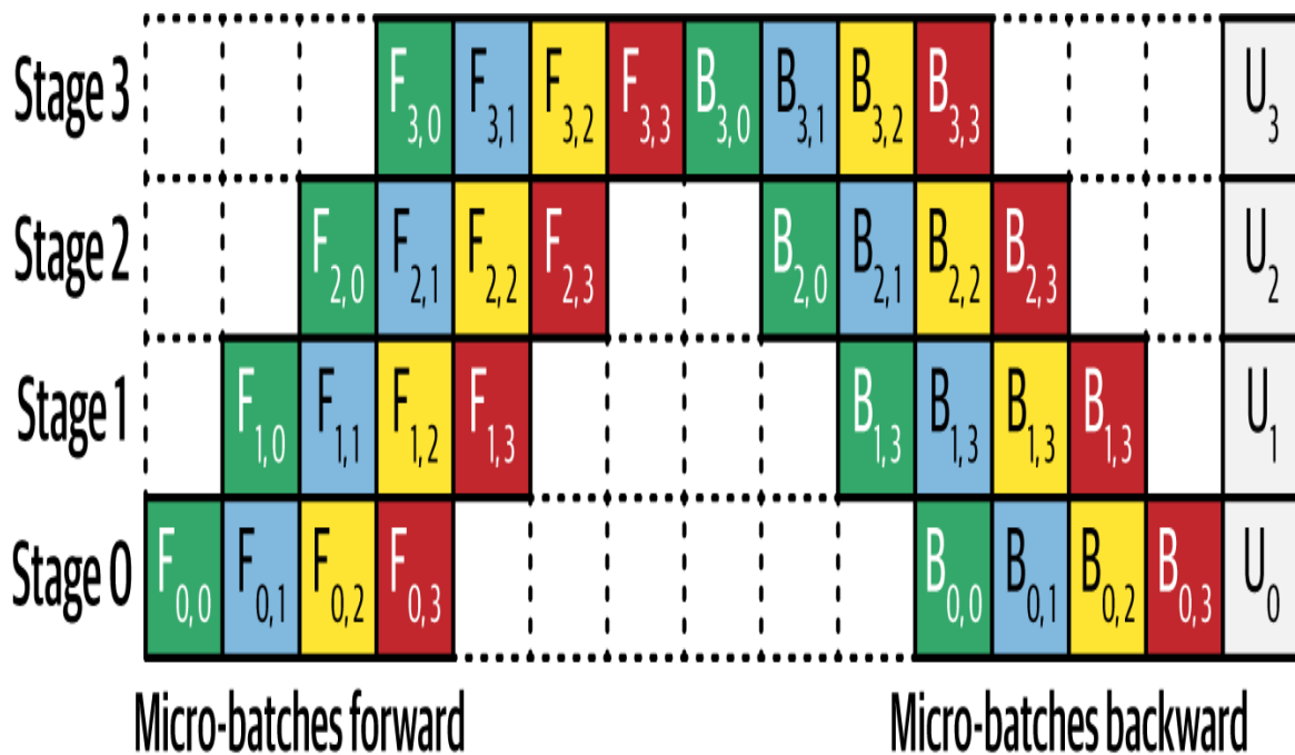
Figure 9-1. Implementing pipeline parallelism
