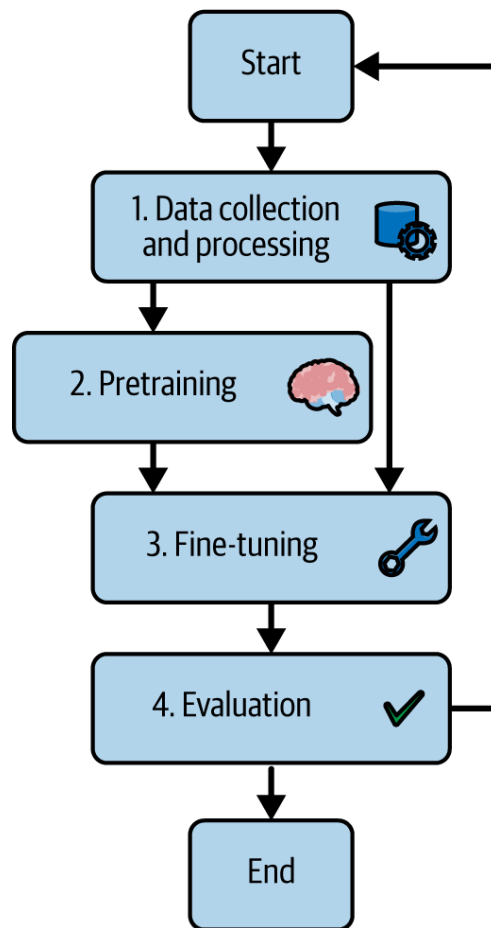
Figure 4-2. Example of an LLM training pipeline
