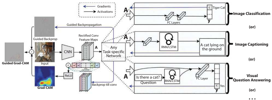
Figure 9.2 Grad-CAM (gradient-weighted class activation mapping).
