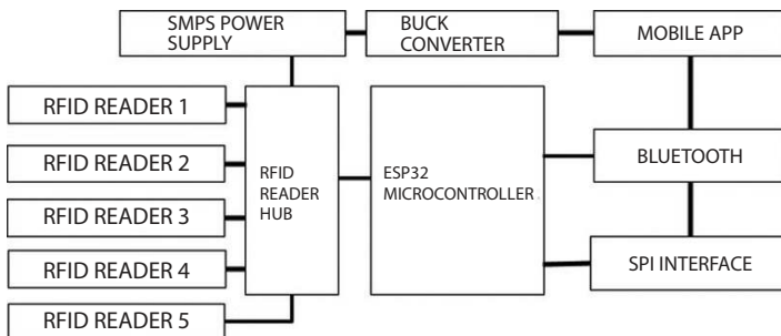
Figure 7.1 Block diagram.
