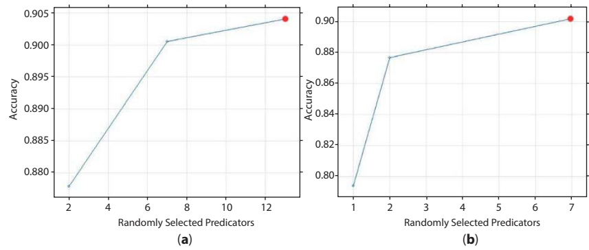
Figure 10.6 (a) mtry value by Grid search (b) mtry value by Random Search.
