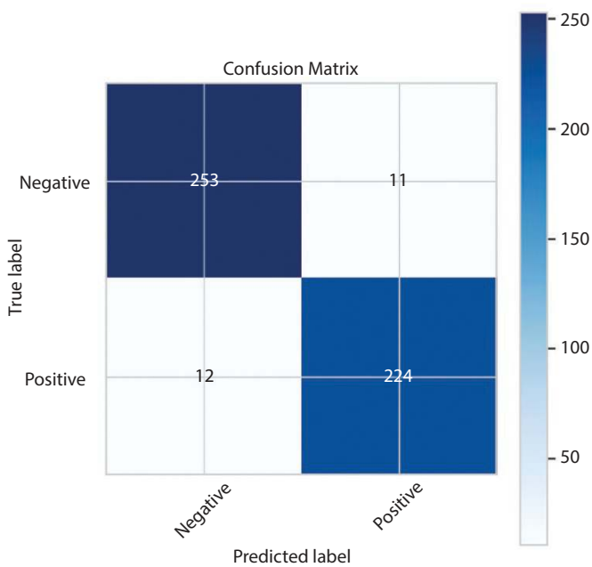
Figure 5.3 Confusion matrix.
