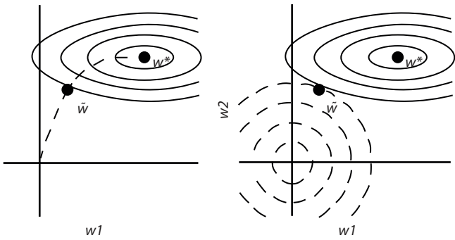
Figure 21.9 L1 regularization [19].
