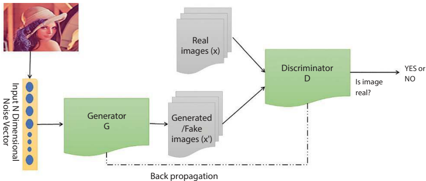
Figure 2.3 GAN architecture.
