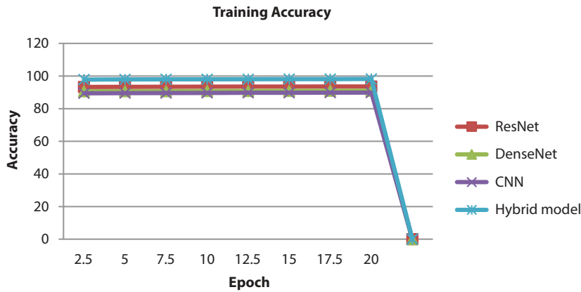
Figure 3.9 Training accuracy.
