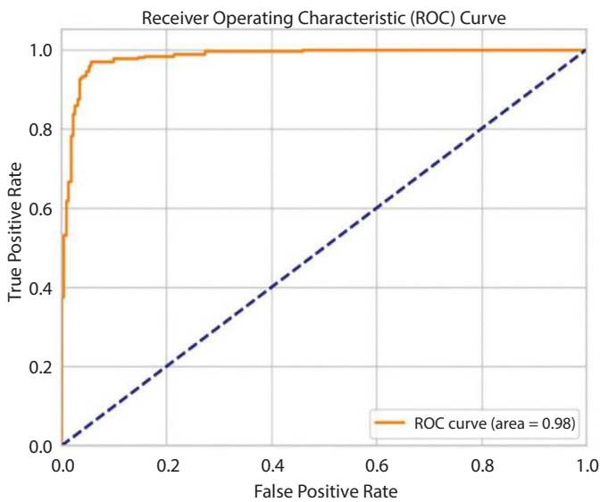
Figure 5.4 ROC curve.
