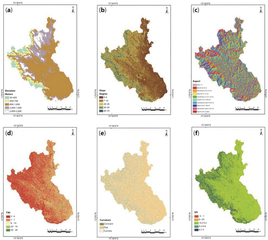
Figure 10.2 Thematic layers of (a) elevation, (b) slope, (c) aspect, (d) TWI, (e) curvature (f) SPI.
