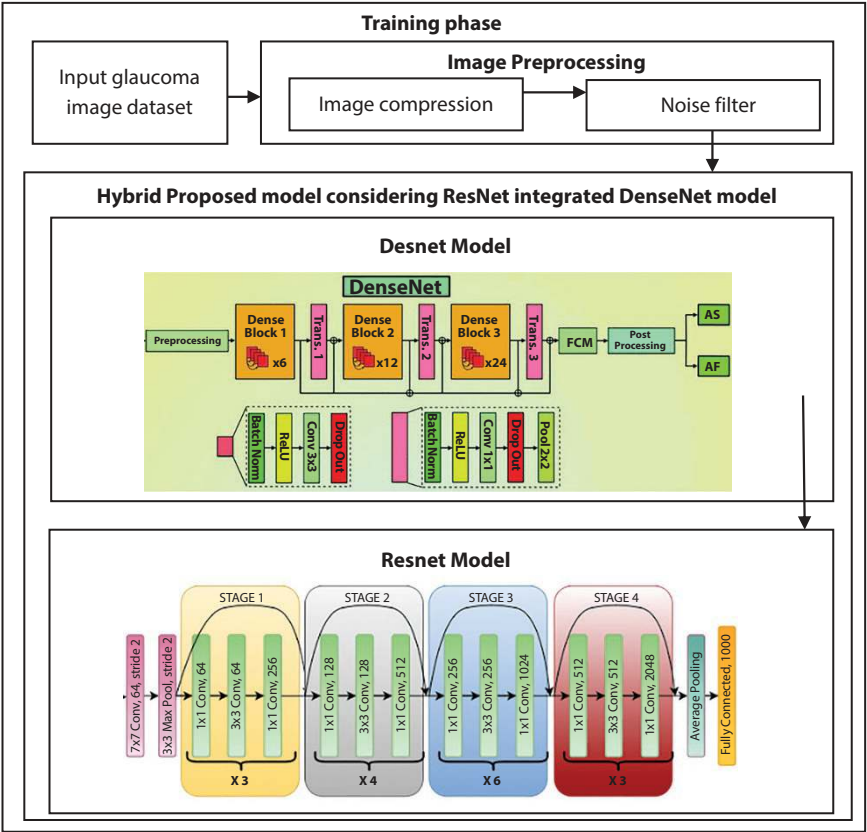
Figure 3.5 Proposed work model.
