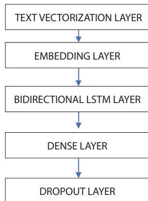
Figure 5.2 Implementation of deep learning model.
