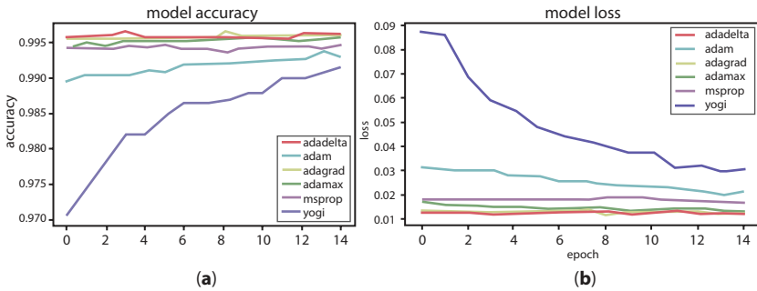
Figure 21.7 (a) Optimizers models accuracy. (b) Optimizers models loss.
