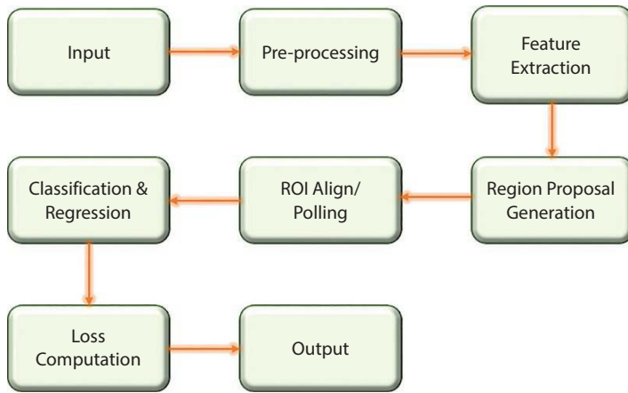
Figure 15.3 Basic architecture and training process of object detection.
