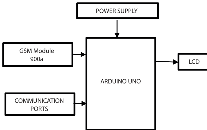
Figure 4.1 (a) Functional pattern of hardware unit.
