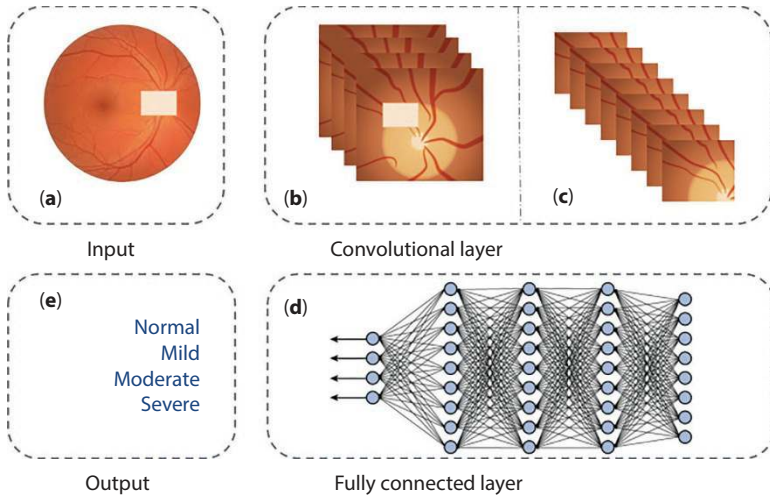
Figure 3.3 Glaucoma detection using deep learning.
