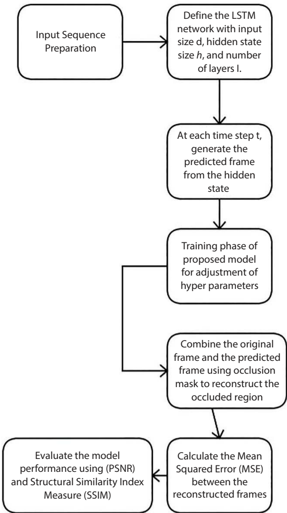
Figure 17.1 Proposed system flow diagram.
