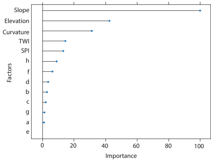
Figure 10.7 Importance of each factor that influencing the landslide event in Kodagu.
