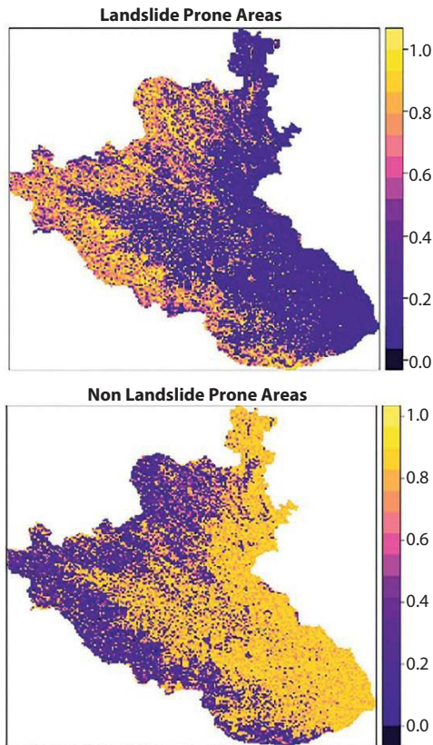
Figure 10.10 (a) Landslide-prone areas and (b) non-landslide-prone areas of Kodagu.
