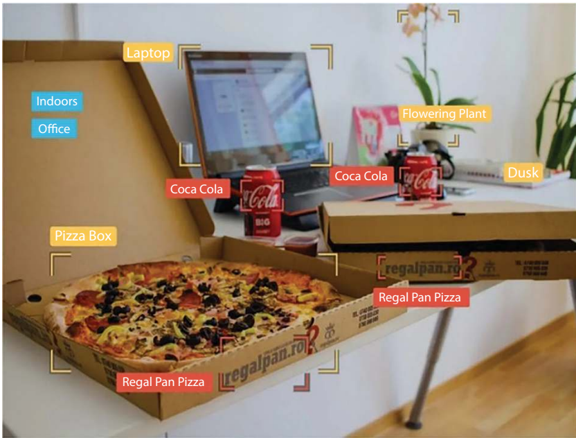
Figure 19.6 Visual intelligence.
