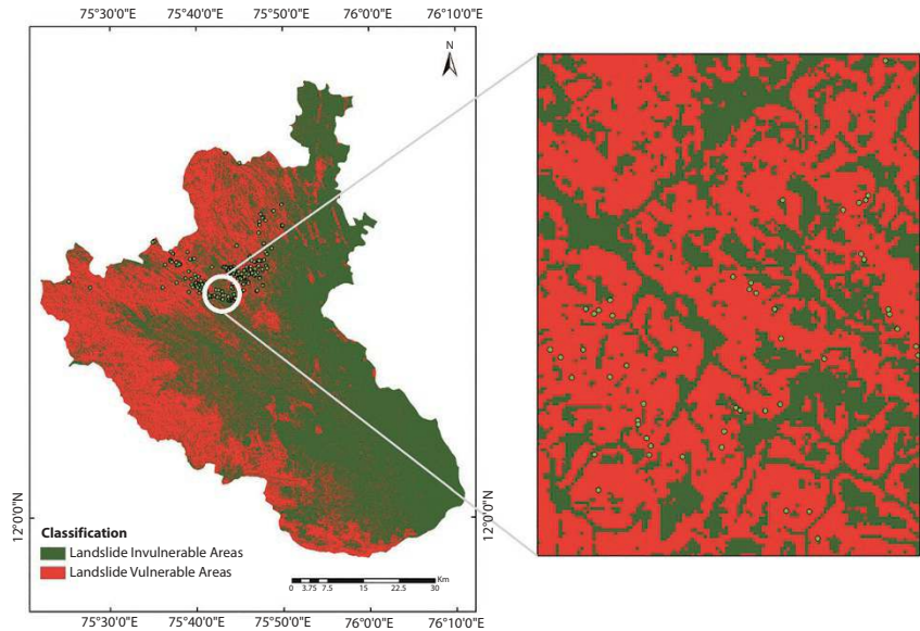
Figure 10.11 Landslide and non-landslide-vulnerable area of Kodagu region.
