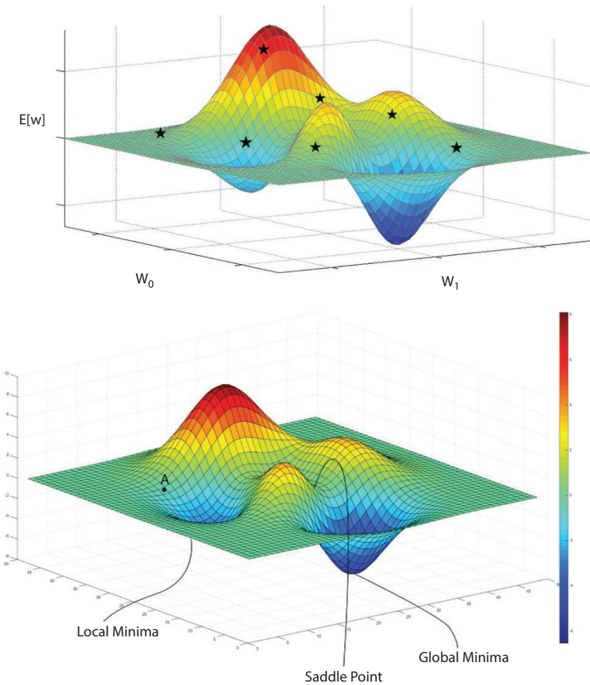
Figure 21.8 Stochastic gradient descent with momentum-local and global minima [7].
