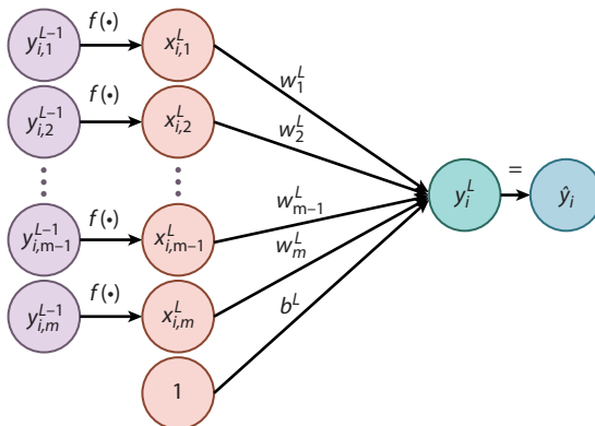
Figure 21.14 Last layer of the assumed neural network for a training sample [22].
