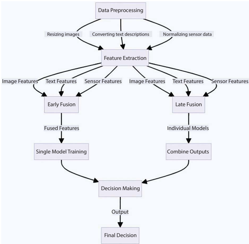
Figure 14.3 Multimodal fusion strategy for computer vision process.
