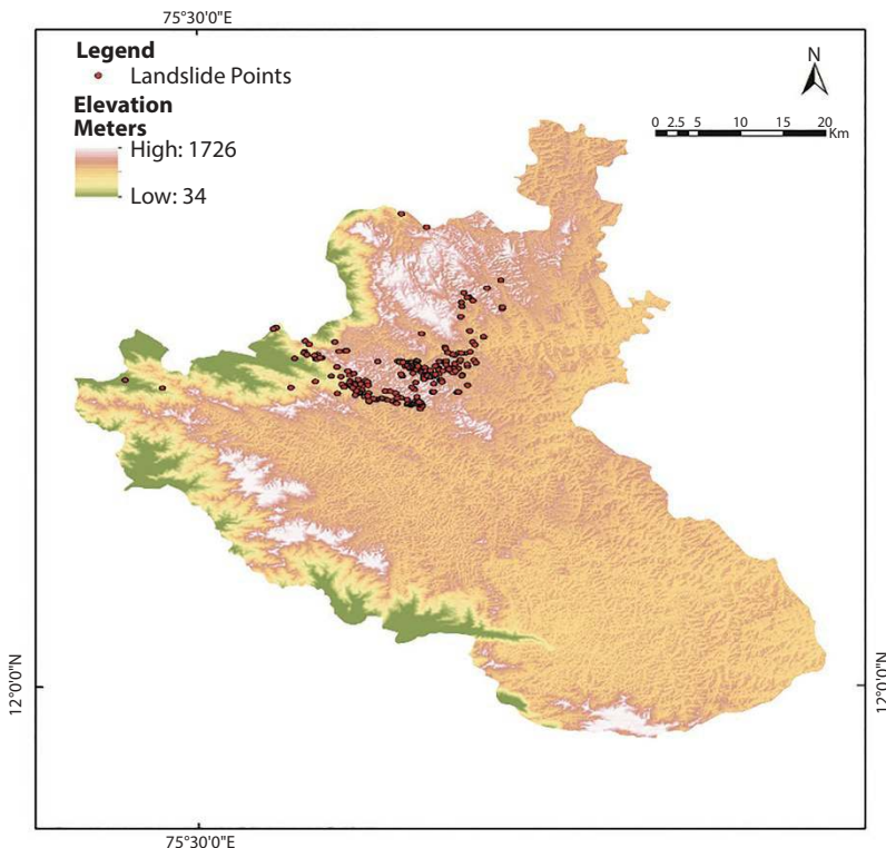
Figure 10.1 Historical landslide distribution of Kodagu, Karnataka State, India.
