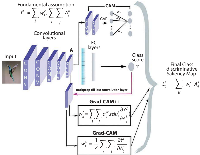
Figure 9.3 Grad-CAM++.
