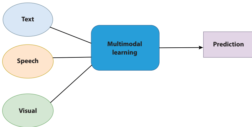
Figure 14.2 Multimodal learning.
