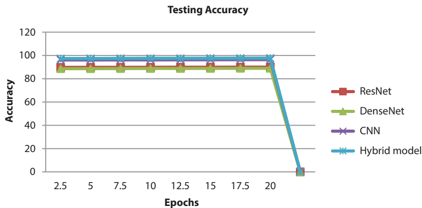
Figure 3.8 Testing accuracy.
