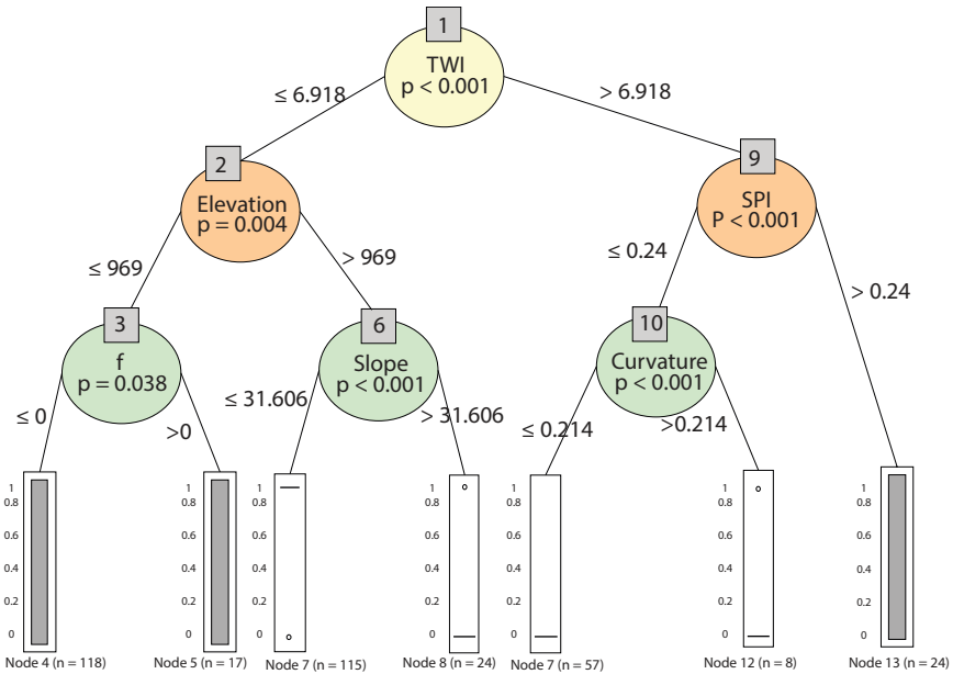
Figure 10.5 Tree generated by binary random forest classifier.
