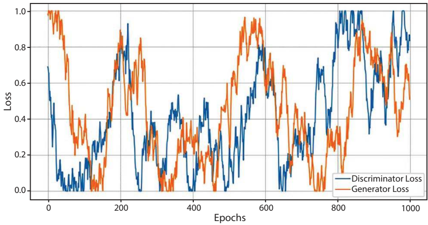
Figure 20.2 Loss curves for discriminator and generator over epochs.
