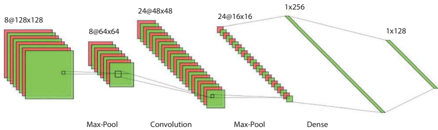
Figure 21.3 Convolution of images in layer architecture [18].
