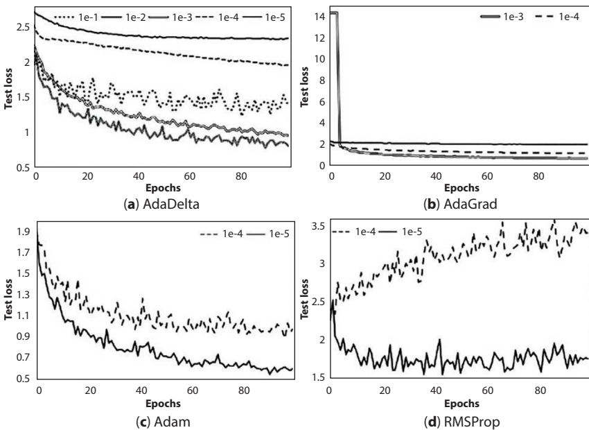
Figure 21.6 Tuning of learning rate for adaptive optimizers. (a–d) Validation loss evolution [16].
