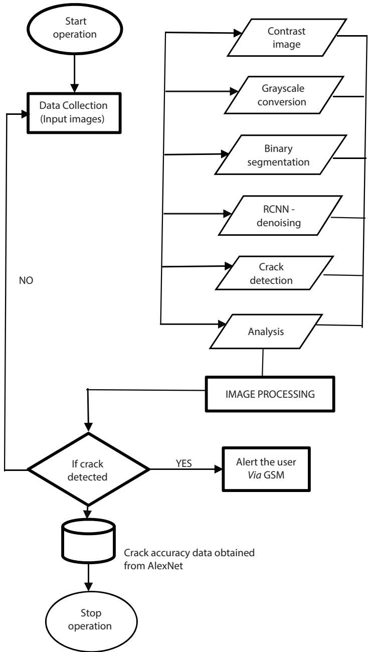
Figure 4.1 (b) Flowchart of damage detection of road surface.
