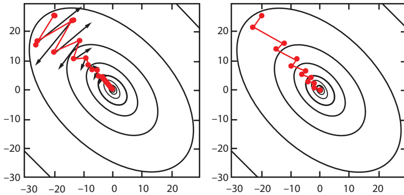
Figure 21.4 From good fellow. SGD (left) vs SGD with momentum (right) [15].
