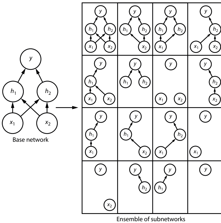
Figure 21.11 Structural decomposition of example neural network [20].
