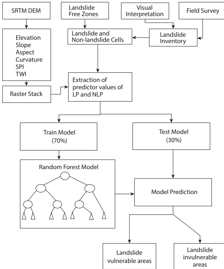
Figure 10.3 Workflow of random forest algorithm to generate LSM.
