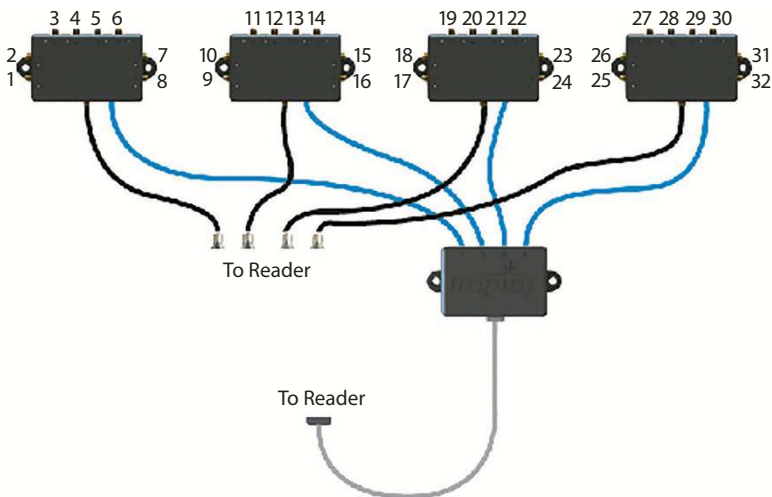
Figure 7.4 RFID reader hub.
