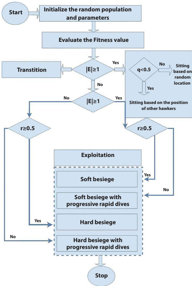
Figure 1.5 Flowchart of HHO.
