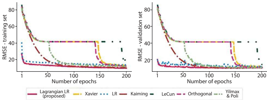
Figure 21.15 Training and validation set after each epoch [22].
