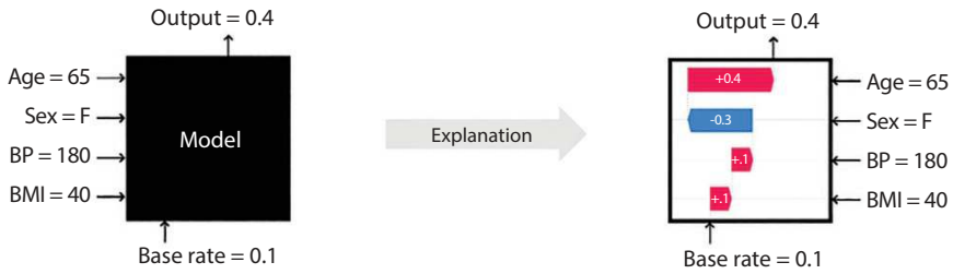
Figure 9.6 SHapley additive explained (SHAP).
