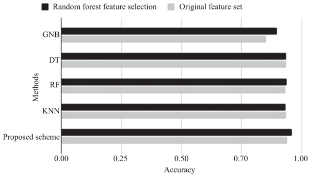
Figure 13.8 Compare deep stacked ensemble accuracy to machine learning methods
