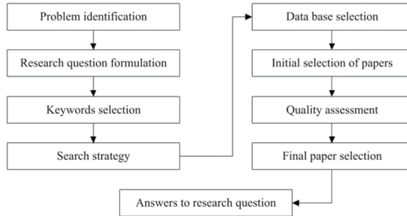
Figure 8.1 SLR methodology
