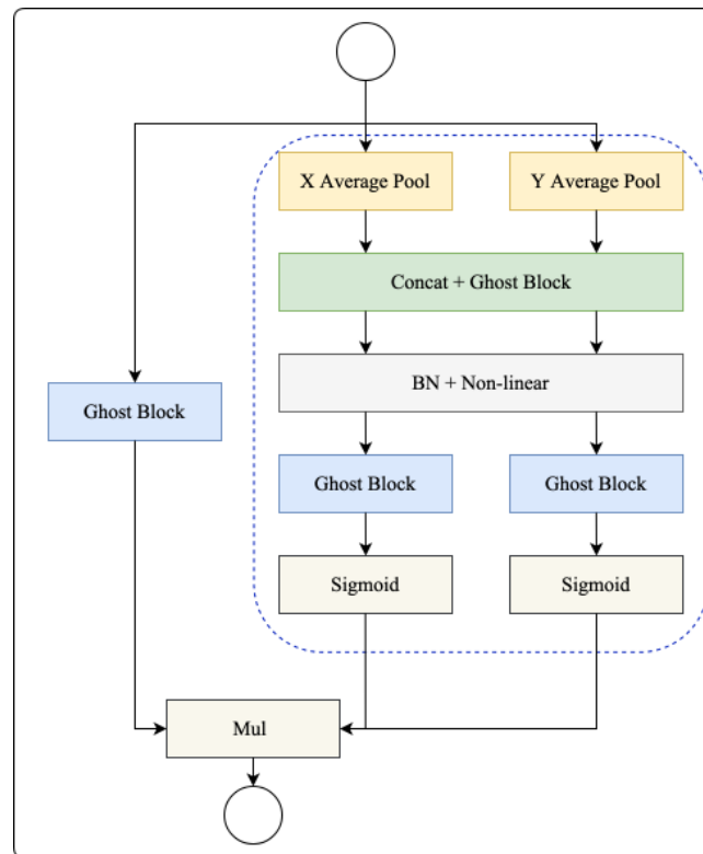
Figure 4. The diagram of GGC block. The blue dash square denotes the ghost coordinate attention (GCA).
