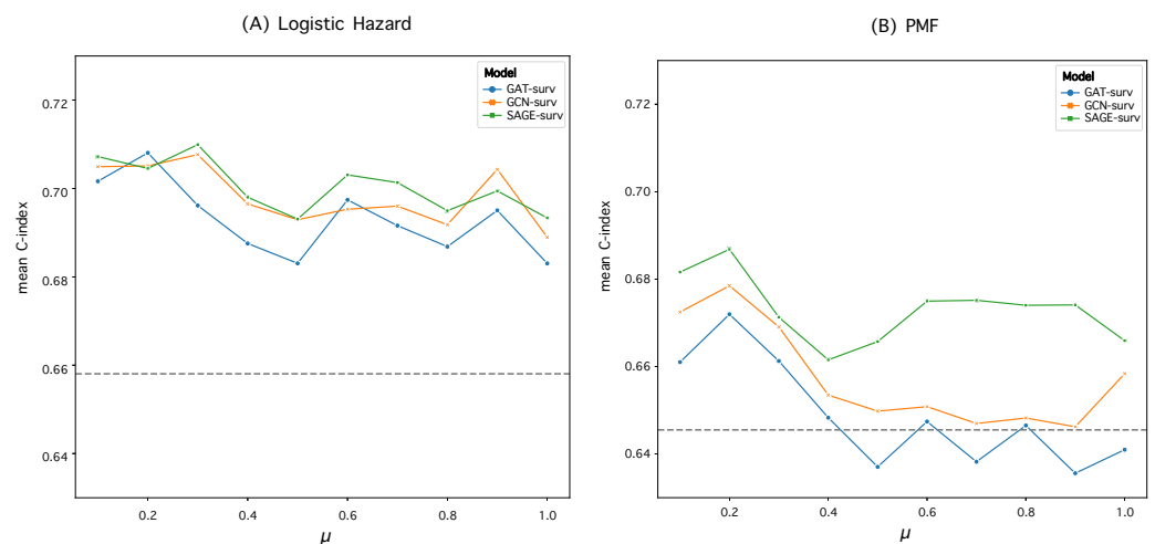
Figure 2. Performance variation of GNN-surv models in the KIRC dataset for different hyperparameter \mu values. The discrete-time survival models are (A) Logistic Hazard and (B) PMF. The performance metrics are mean C^{td} values obtained from 50 random data splits. The gray dotted line represents the mean C^{td} of the MLP model, used as a baseline.
