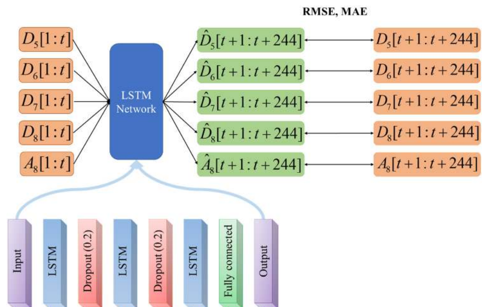
Figure 4. Diagram of the proposed time-series prediction based on MODWT-LSTM.
