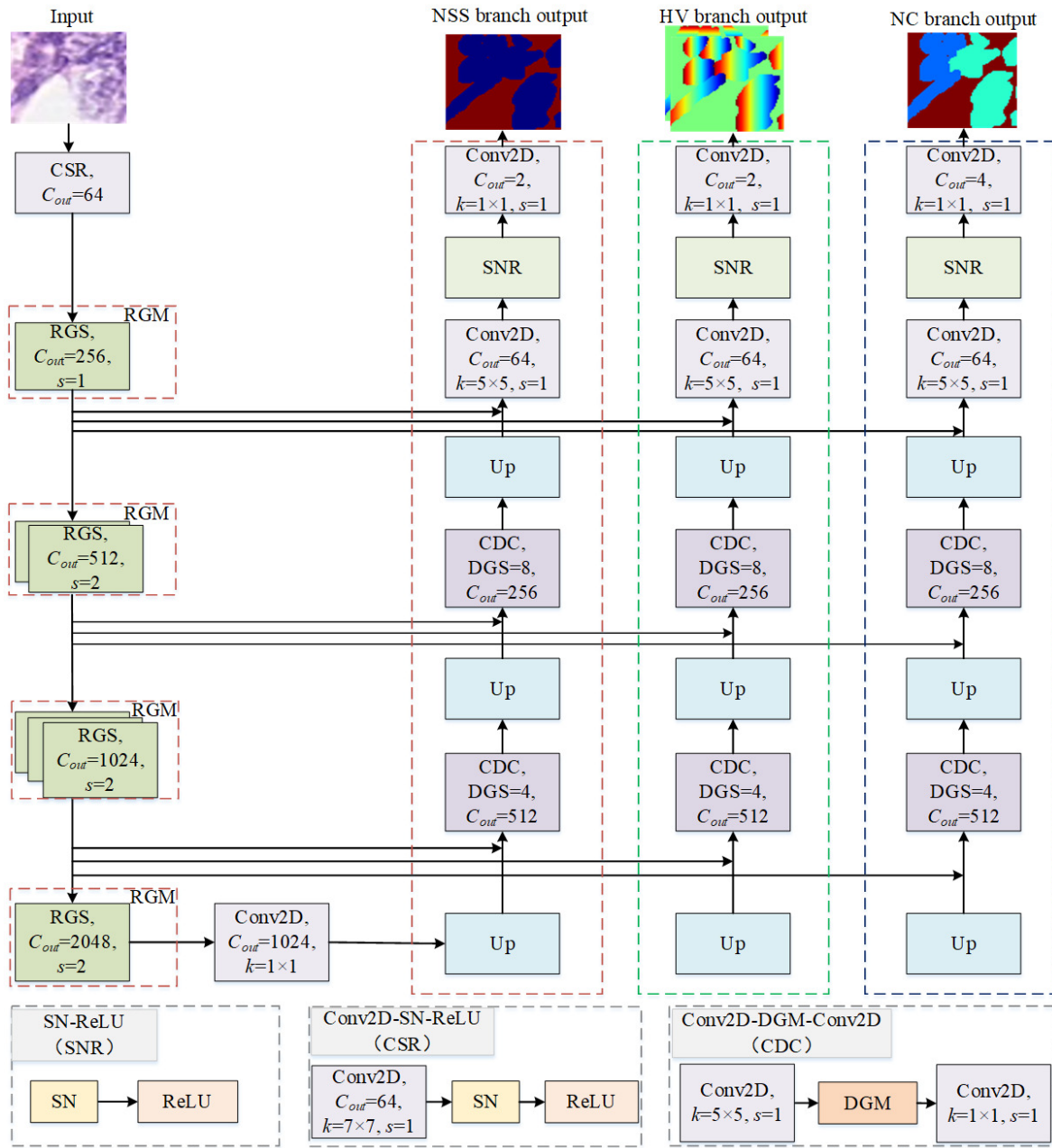
Figure 2. The structure of GSN-HVNET. Our proposed network contains an encoder and a decoder. The encoder, which extracts an effective set of features, is composed of a CSR block, four RGMs, and a Conv2D. The decoder is composed of three branches to achieve accurate nuclei instance segmentation and classification simultaneously.
