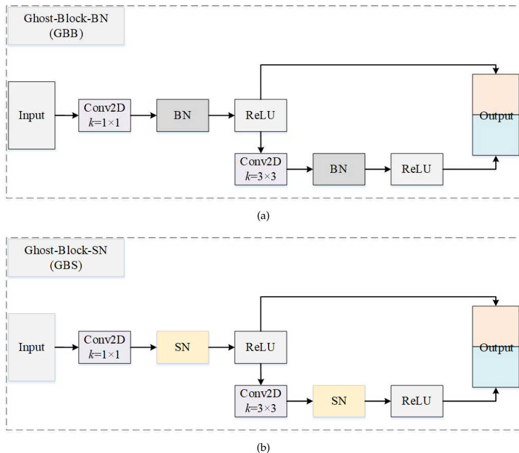
Figure 3. An illustration of the ghost block and the improved ghost block with switchable normalization. (a) Ghost block with batch normalization. (b) Ghost block with switchable normalization.
