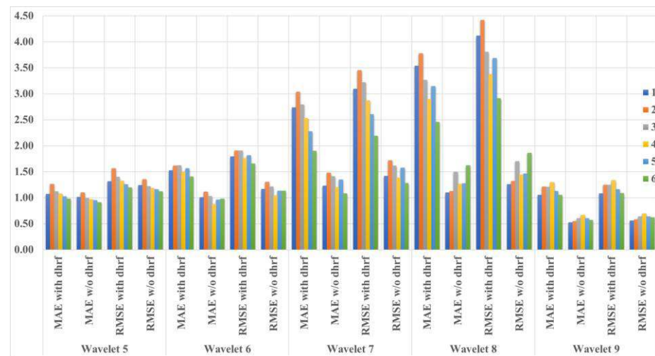
Figure 8. Comparison of MAE and RMSE for all data segmentations: (1) MODWT 600 s and LSTM training 300 s, (2) MODWT 600 s and LSTM training 600 s, (3) MODWT 300 s and LSTM training 300 s, (4) MODWT 150 s and LSTM training 150 s, (5) MODWT 90 s and LSTM training 90 s, and (6) MODWT 60 s and LSTM training 60 s.
