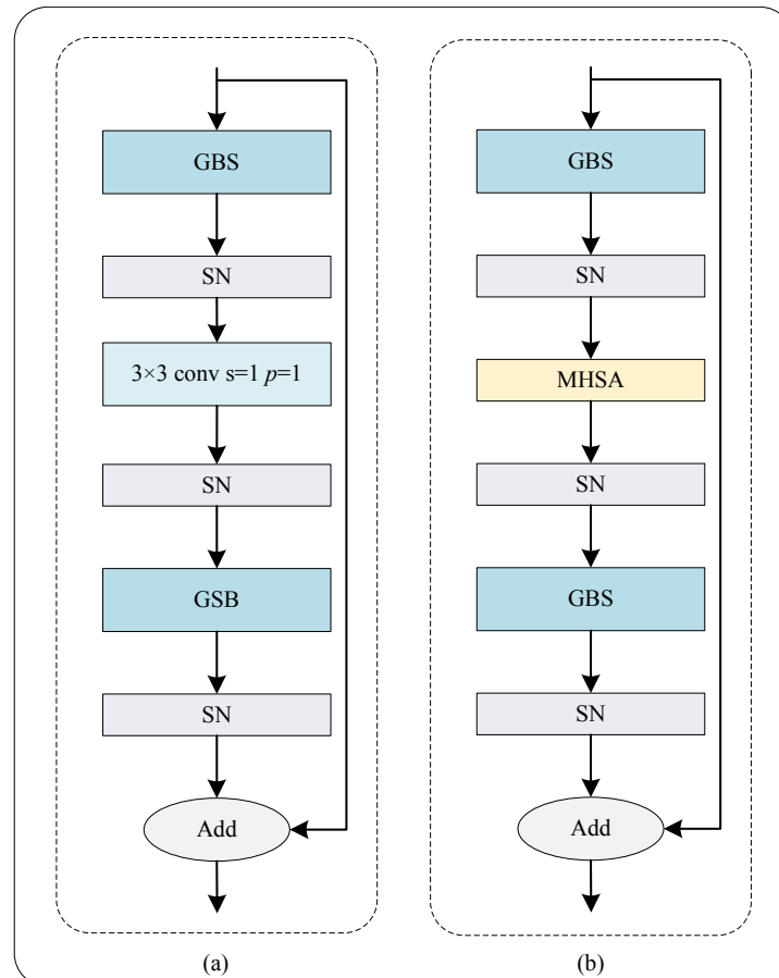
Figure 4. Schematic diagram of the proposed bottleneck. (a) RGS Bottleneck. (b) Bottleneck transformer. GBS and SN denote the ghost block with switchable normalization and switchable normalization, respectively. MHSA denotes multi-head self-attention.
