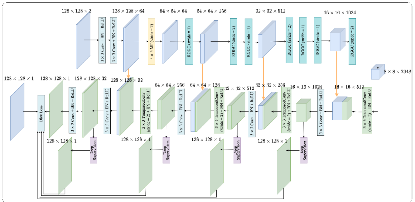
Figure 2. Detailed architecture of RGGC-UNet.
