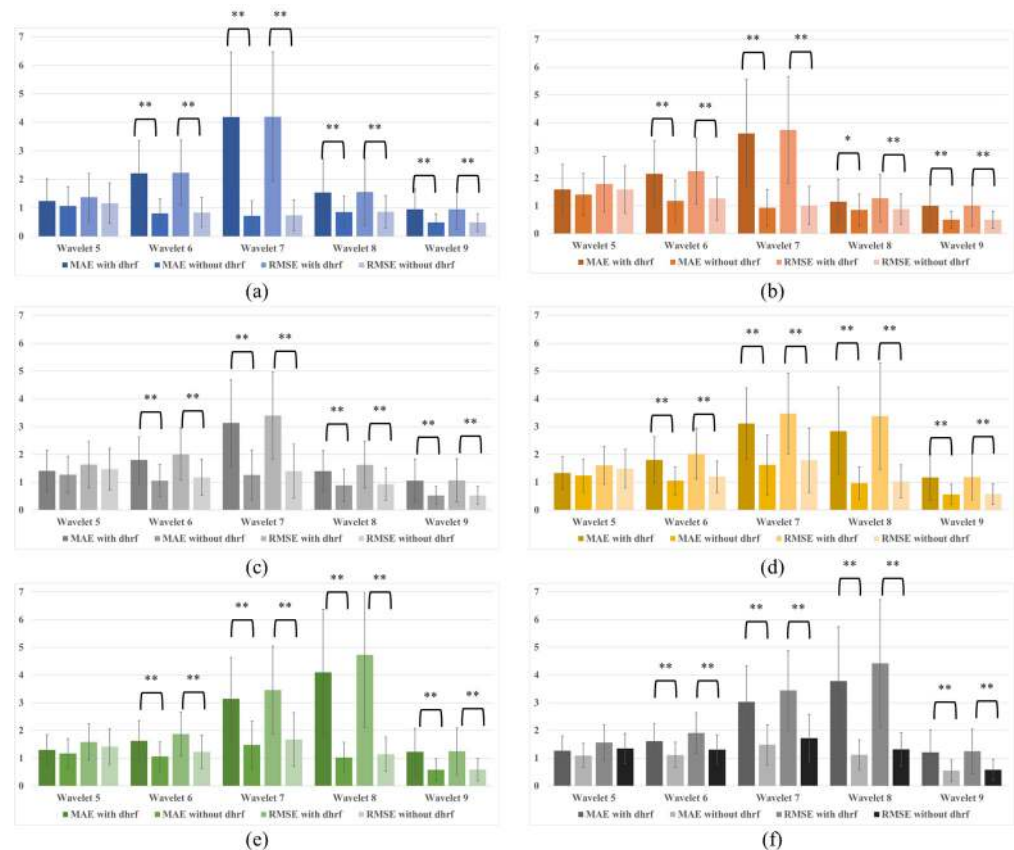
Figure 9. MAEs and RMSEs of 600 s data MODWT-LSTM for each wavelet: (a) 1 s, (b) 3 s, (c) 5 s, (d) 10 s, (e) 15 s, and (f) 30 s (* p < 0.05 , ** p < 0.01 ).
