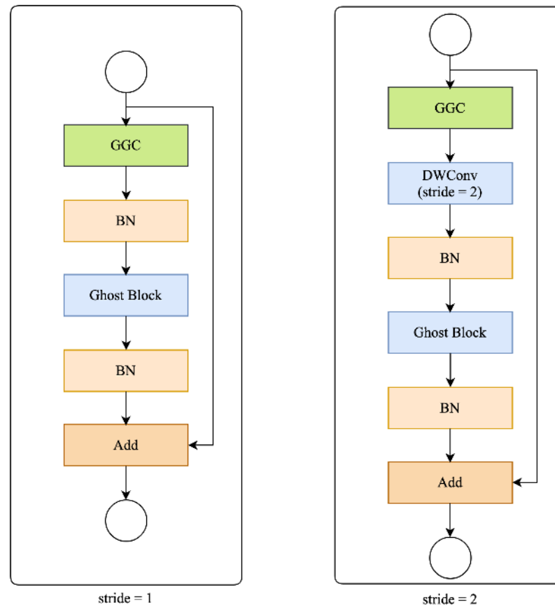
Figure 5. Diagram of an RGGC block.
