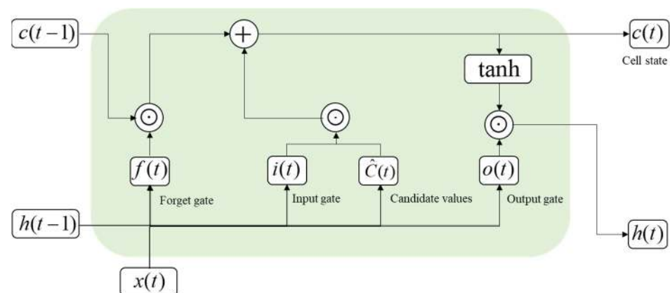
Figure 3. A structure of LSTM layers.
