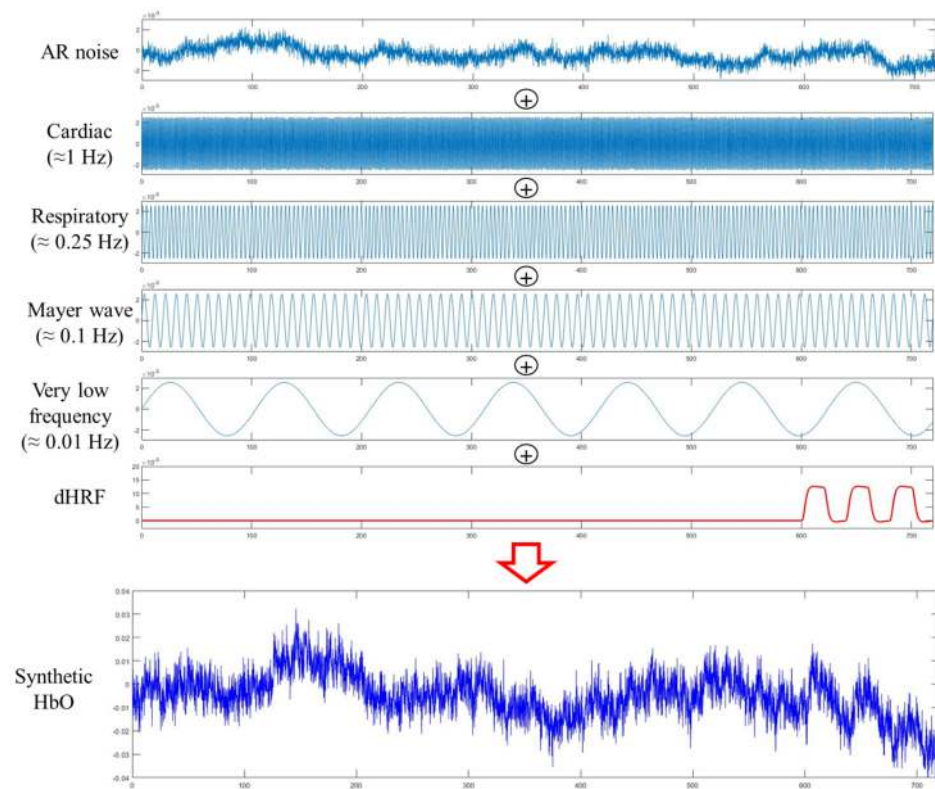
Figure 1. A synthetic HbO signal is made of six components.
