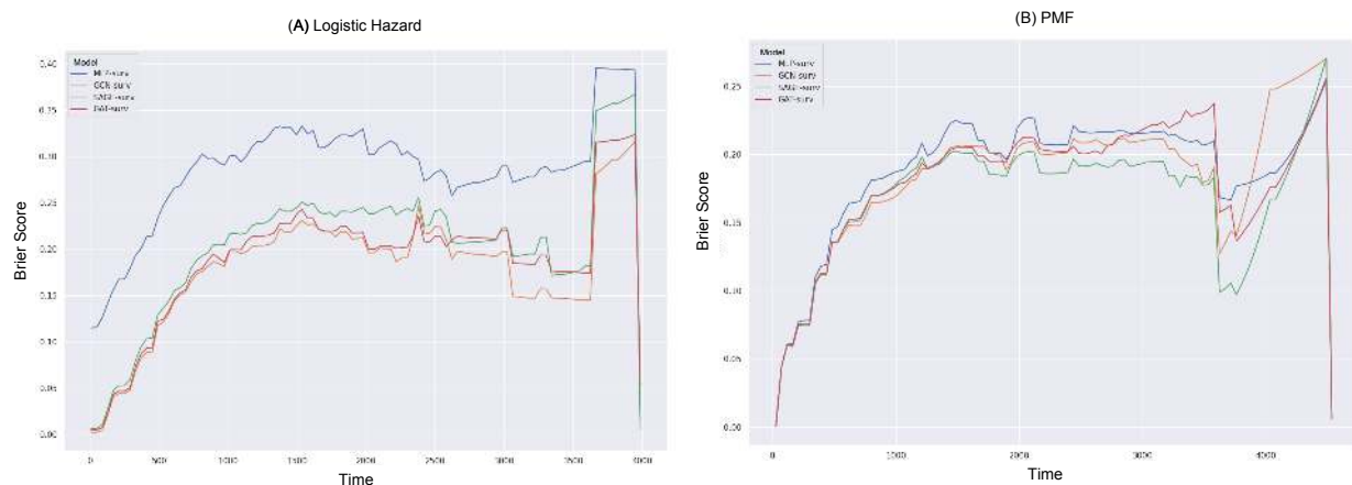
Figure 4. Brier scores over survival time (in days) for different GNN-surv models and MLP model in the KIRC dataset. Discrete-time survival models considered are (A) Logistic Hazard and (B) PMF.
