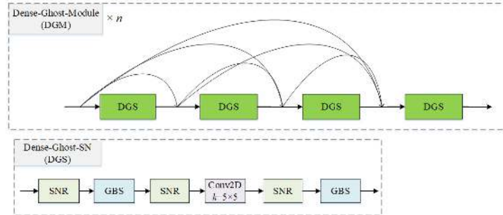
Figure 6. Dense ghost module with switchable normalization. The GBS and SNR denote the ghost block with switchable normalization and switchable normalization with ReLU, respectively.
