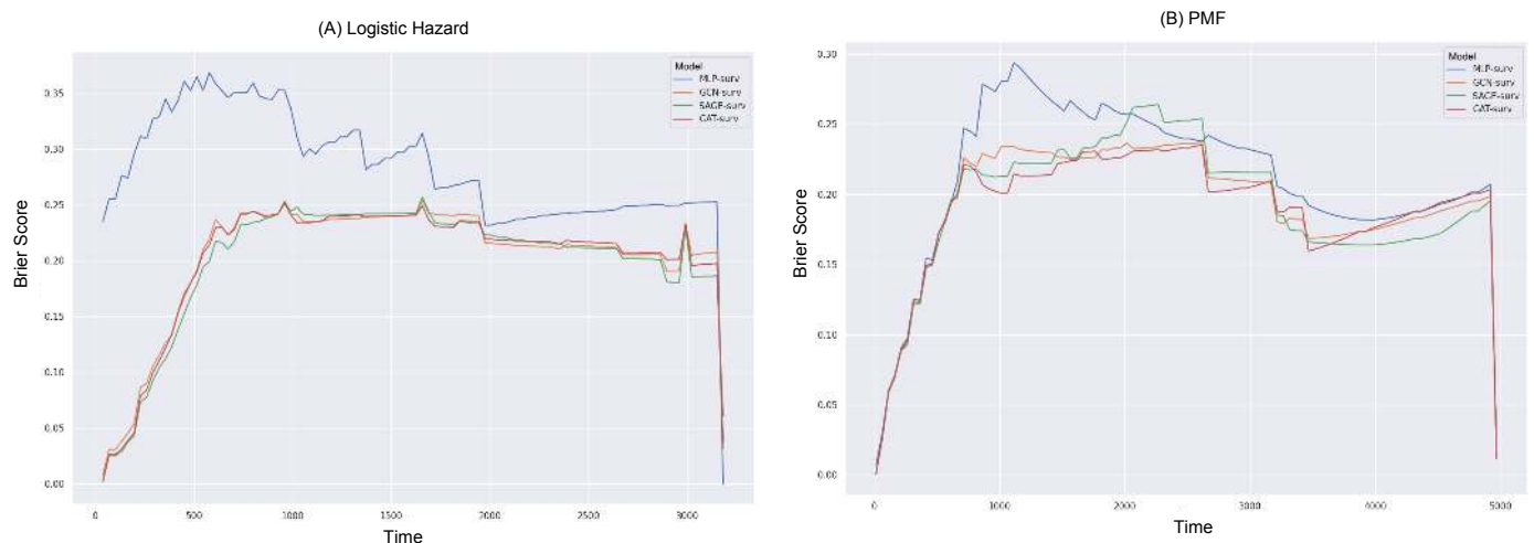
Figure 3. Brier scores over survival time (in days) for different GNN-surv models and MLP model in the BLCA dataset. Discrete-time survival models considered are (A) Logistic Hazard and (B) PMF.
