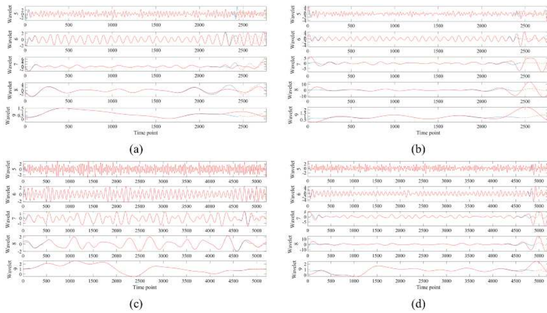
Figure 6. Prediction results from synthetic data: (a) Without dHRF (MODWT 300 s, LSTM 300 s), (b) with dHRF (MODWT 300 s, LSTM 300 s), (c) without dHRF (MODWT 600 s, LSTM 600 s), and (d) with dHRF (MODWT 600 s, LSTM 600 s) (blue line: training data, red line: MODWT results including test time, orange dotted line: predicted result).
