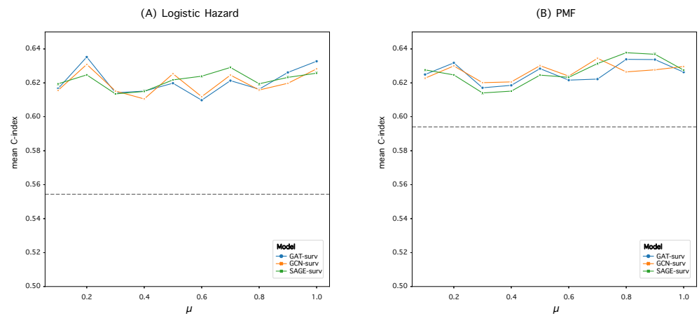
Figure 1. Performance variation of GNN-surv models in the BLCA dataset for different hyperparameter \mu values. The discrete-time survival models are (A) Logistic Hazard and (B) PMF. The performance metrics are mean C^{td} values obtained from 50 random data splits. The gray dotted line represents the mean C^{td} of the MLP model, used as a baseline.
