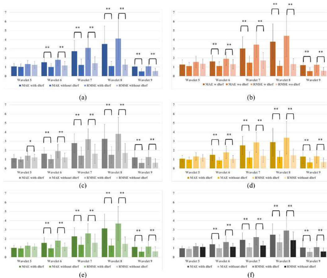
Figure 7. MAEs and RMSEs for wavelets 5–9: (a) MODWT 600 s and LSTM training 300 s, (b) MODWT 600 s and LSTM training 600 s, (c) MODWT 300 s and LSTM training 300 s, (d) MODWT 150 s and LSTM training 150 s, (e) MODWT 90 s and LSTM training 90 s, and (f) MODWT 60 s and LSTM training 60 s (* p < 0.05 , ** p < 0.01 ).
