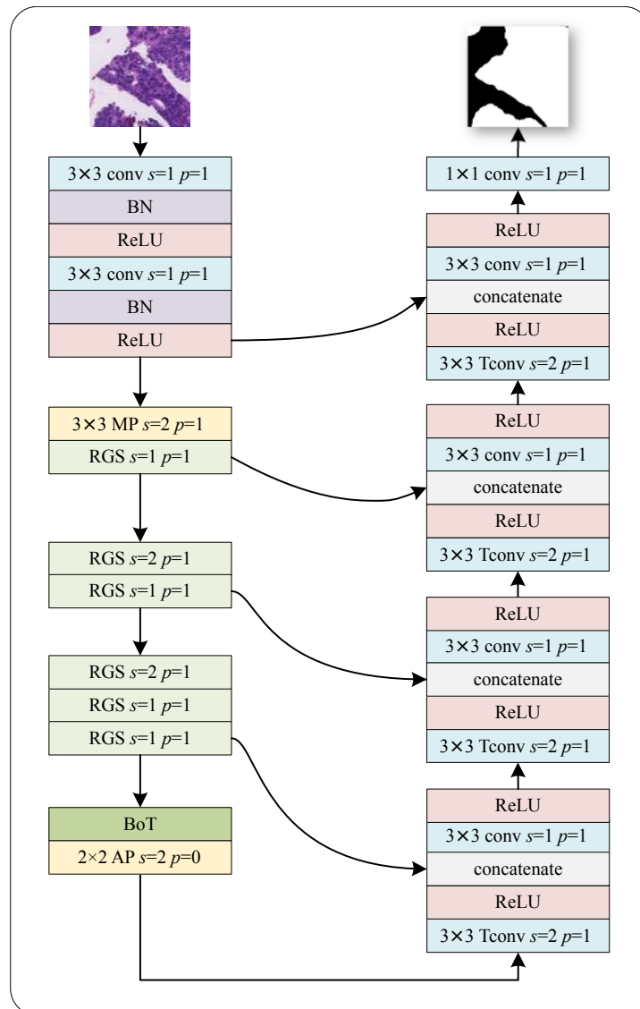
Figure 2. Schematic diagram of RGSB-UNet. RGS denotes the proposed residual ghost block with switchable normalization, and BoT denotes the bottleneck transformer. MP and AP denote the max and average pooling, respectively. Tconv denotes the transposed convolution used for upsampling.
