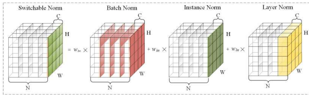
Figure 4. Switchable normalization. It learns to select different normalizers for different normalization layers of a deep neural network.
