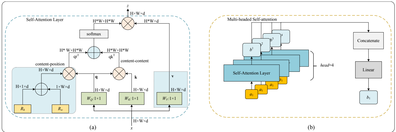
Figure 5. Schematic diagram of (a) self-attention [26] and (b) multi-head self-attention.
