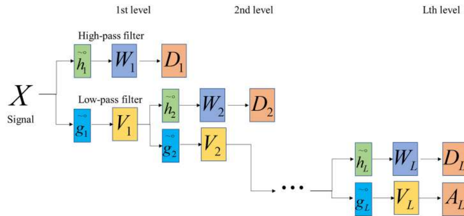
Figure 2. Schematic of the MODWT decomposition.
