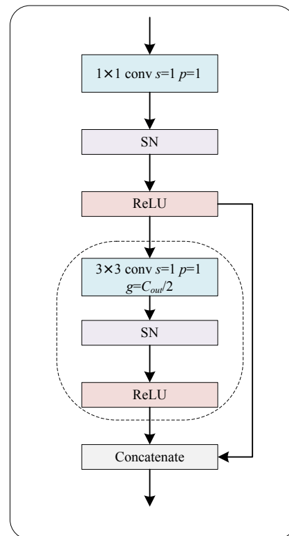
Figure 3. Schematic diagram of Ghost block with switchable normalization. The dash box denotes the cheap operation that uses a 3 \times 3 group convolution in the ghost block.
