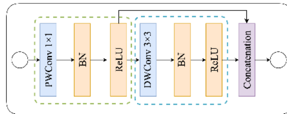
Figure 3. Diagram of ghost block. The green dash box represents identity operation. The blue dash box represents the efficiency operation [28].
