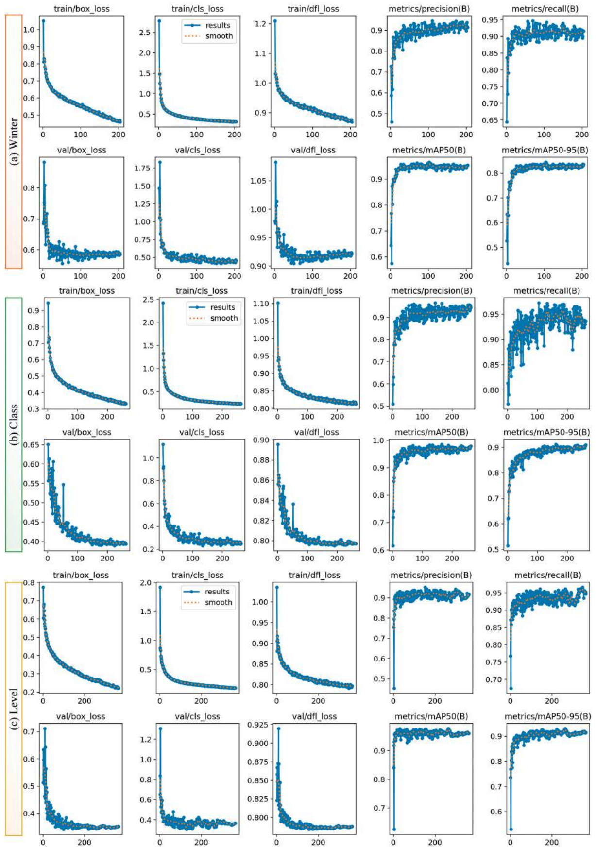
Figure 3. Graphs showing the loss values (box_loss, cls_loss, df_l_loss) and performance metrics (precision, recall, mAP50, mAP50-95) of the model during the training and validation processes across epochs: (a) Winter for YOLO11n, (b) class for YOLO11n, (c) level for YOLO11m.
