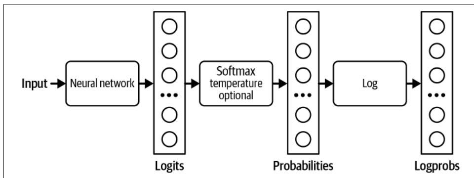
Figure 2-17. How logits, probabilities, and logprobs are computed.
