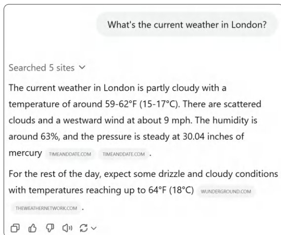
Figure 1.4 ChatGPT called a function to search the web behind the scenes and inserted the results into the user's prompt. This creates the illusion that the LLM browses the web.
