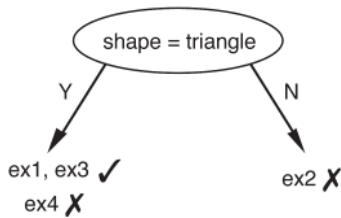
FIGURE 5.8 Starting to build a decision tree.
