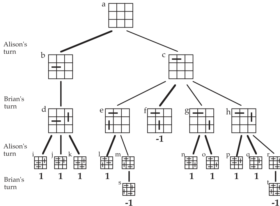
FIGURE 11.1 Game tree for “placing dominoes”.
