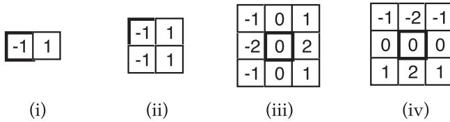
FIGURE 12.8 Different gradient filters.
