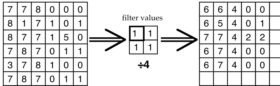
FIGURE 12.6 Applying a 2 \times 2 smoothing filter.
