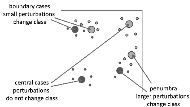
FIGURE 21.11 Identifying central and boundary examples.
