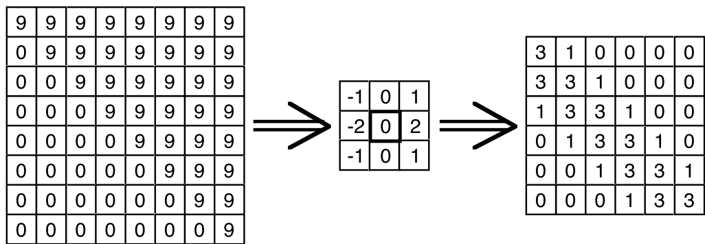
FIGURE 12.10 Gradient filter on a diagonal edge.
