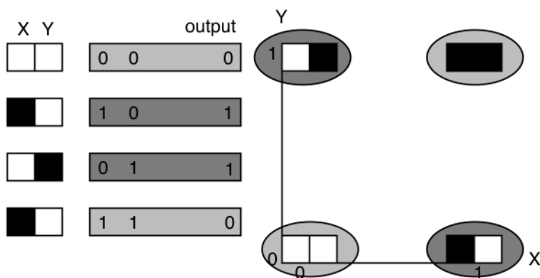
FIGURE 6.5 XOR problem (diagram after Beale &amp; Jackson (1990)).
