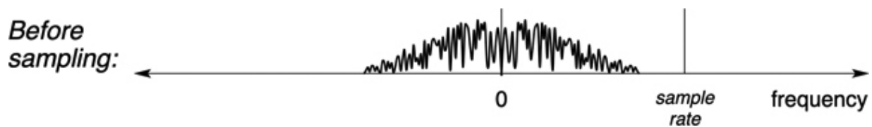
Figure 3.18: A broader spectrum (contains higher frequencies) before sampling. ↗
