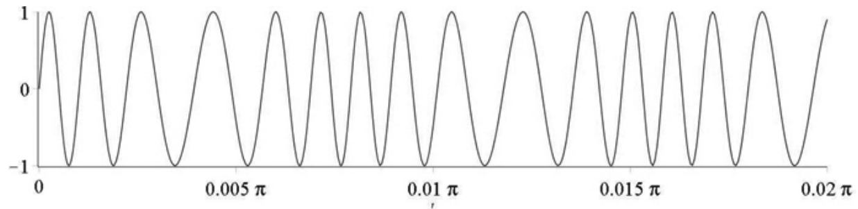
Figure 4.2: A = 1 , C = 242 Hz, D = 2 , M = 40 Hz. ↗
