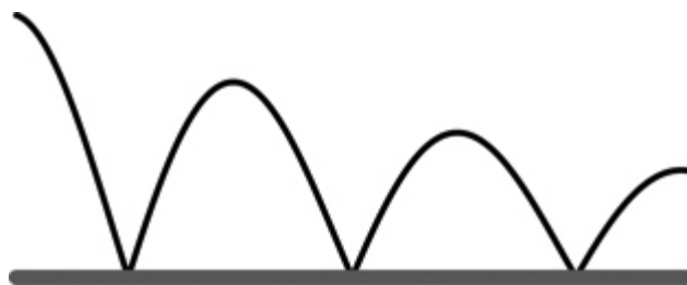
Figure 3.3: The path of a bouncing ball. ↗
