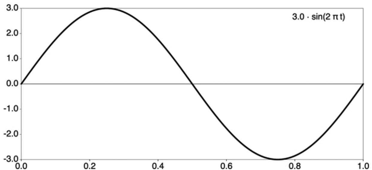
Figure 3.10: Bigger sine curve. ↗
