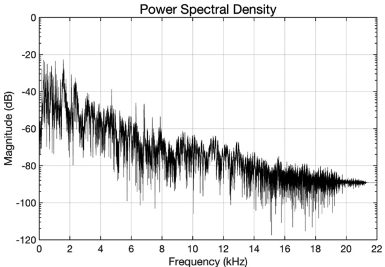
Figure 10.2: The actual spectrum shown here is not important, but the graph covers the range of audible frequencies (about 20KHz) and our range of amplitudes (about 120 dB). We are very sensitive to the shape of the spectrum. ↩
