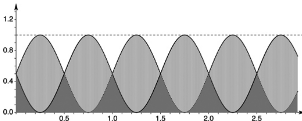
Figure 8.5: The raised cosine, Hann, or Hanning window, is named after the mathematician von Hann. This figure shows multiple Hann windows with 50% overlap, which sum to 1. But that's not enough! In practice, we multiply by a smoothing window twice: once before the FFT and once after the IFFT. See the text on how to resolve this problem ↗
