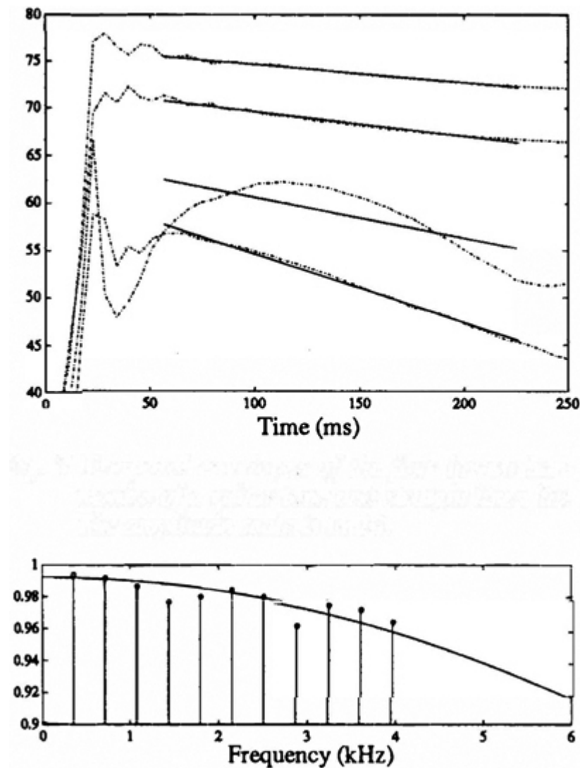
Figure 11.15: Analysis Example, from Karjalainen, Valimaki, and Janosy (47). At top, temporal envelopes of the four lowest harmonics of a guitar tone, with straight line fits. The amplitude scale is in dB. At bottom, estimated magnitude spectrum (circles) is used to fit a 1st-order IIR filter response. ↗
