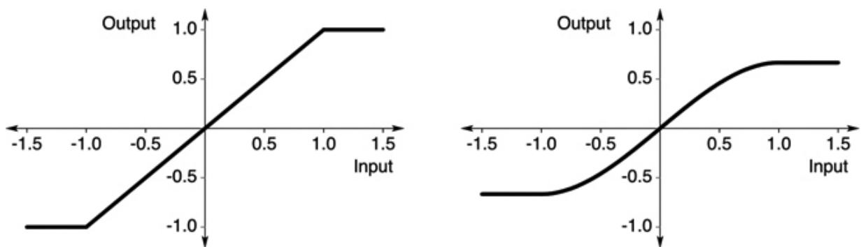
Figure 11.12: Distortion functions. At left is “hard clipping” where the signal is unaffected until it reaches limits of 1 and -1 , at which points the signal is limited to those values. At right is a “soft clipping” distortion that is more like analog amplifiers with limited output range. The amplification is very linear for small amplitudes, but diminishes as the signal approaches the limits of 1 and -1 . ↗
