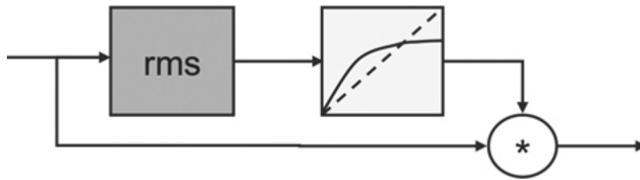
Figure 10.20: Compression/Limiting effect. The input signal is analyzed to obtain the RMS (average) amplitude. The amplitude is mapped to obtain a gain, and the signal is multiplied by the gain. The solid line shown in the mapping (at right) is typical, indicating that soft sounds are boosted, but as the input becomes increasingly loud, the gain is less, reducing the overall dynamic range (i.e., the variation in amplitude is compressed.) ↗
