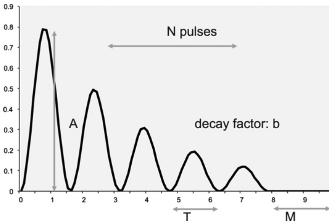
Figure 9.8: Diagram of VOSIM. ↗
