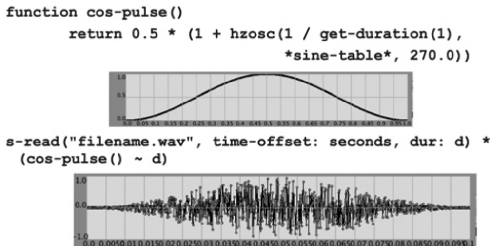
Figure 6.6: Constructing a grain in Nyquist. ↗
