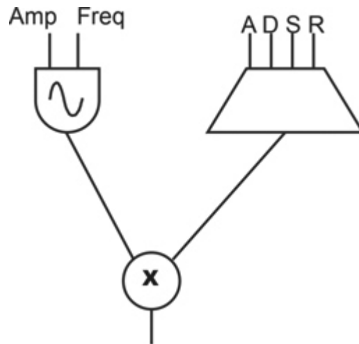
Figure 2.2: Unit generators in Nyquist. ↗
