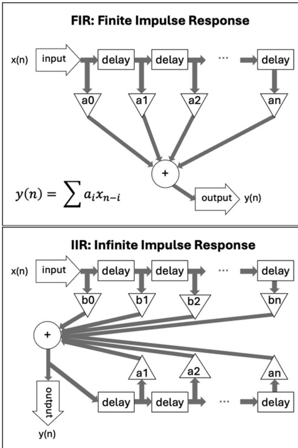
Figure 7.6: FIR and IIR filters. Filters are usually implemented in the time domain by delaying a signal and then adding weighted versions of
