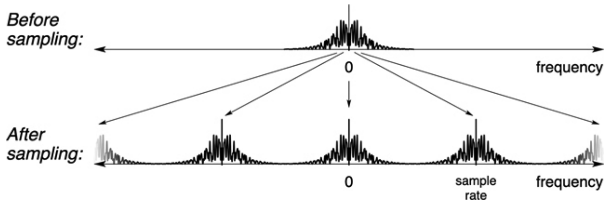
Figure 3.17: Sampling in the time domain gives rise to shifted spectral copies in the frequency domain. The spectral copies are shifted by multiples of the sample rate. ↩
