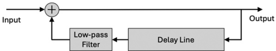
Figure 11.11: Electric Guitar Model by Charles R. Sullivan. The model is based on Karplus-Strong, but the low-pass filter is customized and the model allows continuous input through the summation node to allow for plucking while the string is still vibrating and feedback. ↩
