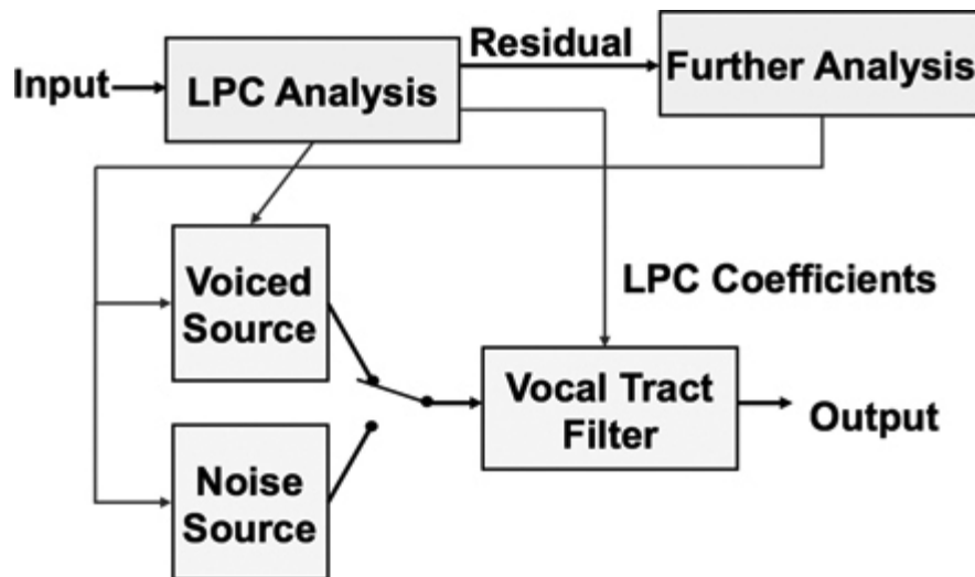
Figure 13.7: Linear Predictive Coding in Practice. 📄
