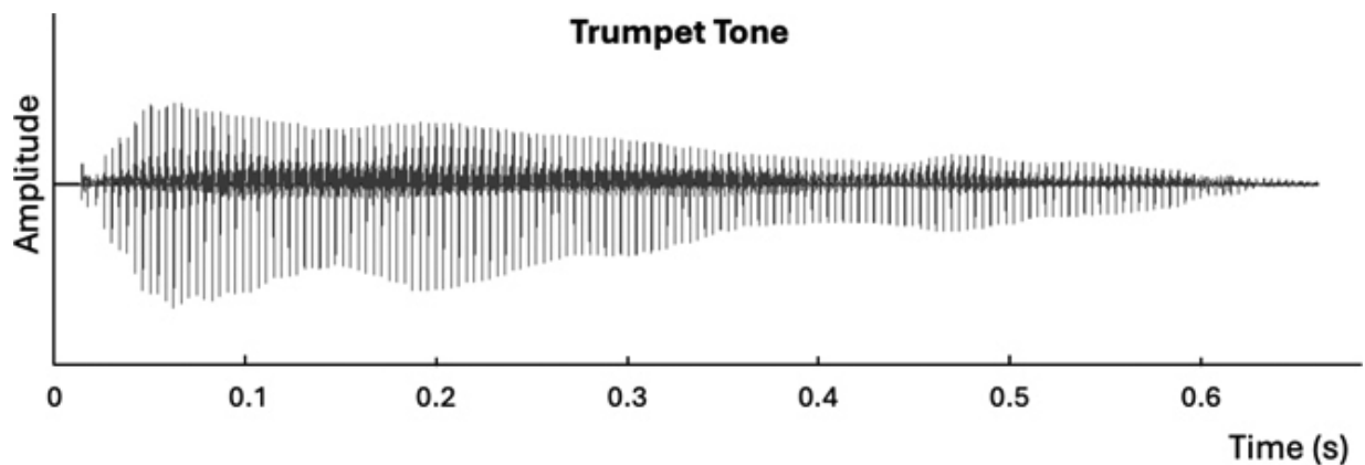
Figure 3.24: A time-domain waveform of a single trumpet tone. It is easy to see variations of amplitude in this time-domain representation. If you connected the peaks, the result would give you the amplitude envelope. More typically, the amplitude would be computed as \sqrt{x(t)^2} with some local averaging to smooth out the peaks. ↗
