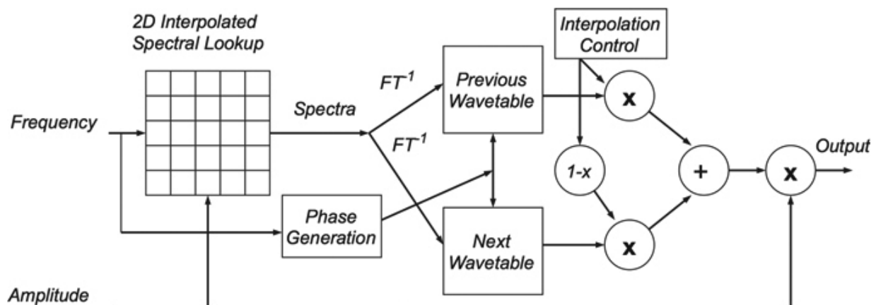
Figure 12.2: Computation for Spectral Interpolation Synthesis.
