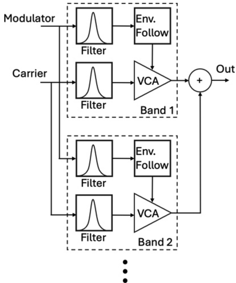
Figure 9.7: Vocoder. ↗
