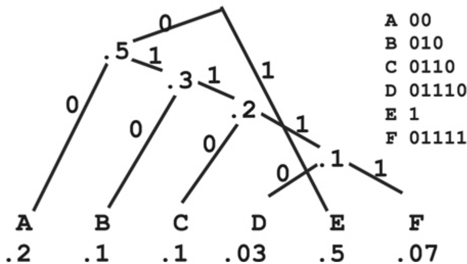
Figure 13.6: Huffman Coding Tree example. ↗
