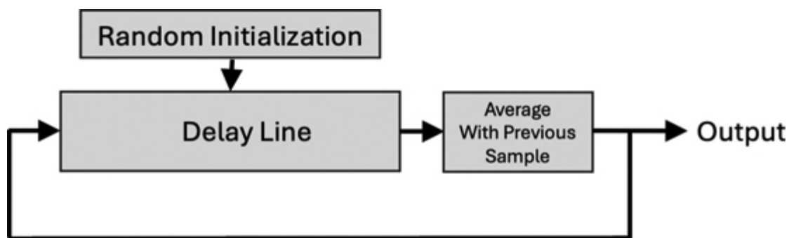
Figure 11.2: Schematic view of a computer software implementation of the basic Karplus-Strong algorithm. For each note, the computer memory buffer is filled with random values (noise). To generate a sample, values are read from the buffer and averaged. The newly calculated sample is both sent to the output stream and stored back into the buffer. When the end of the buffer is reached, we simply wrap around and continue reading at the beginning. This sort of setup is often called a circular buffer. After many iterations of this process, the buffer's contents will have been transformed from noise into a simple waveform. If you think of the random noise as a
