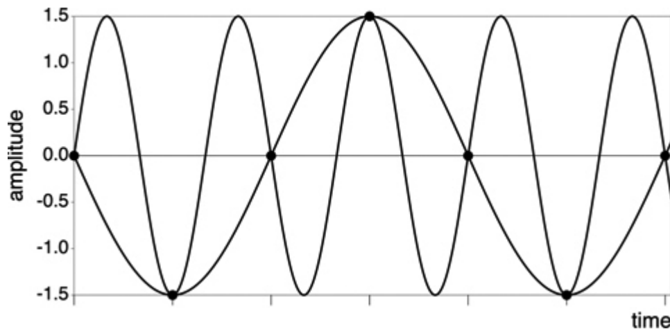
Figure 3.20: Aliasing, or foldover, happens when we sample a frequency that is more than half the sampling rate. When the frequency we want to sample is too high, we undersample and get an unwanted lower-frequency that is created by the sampling process itself. Here, samples are shown as small black circles. Samples of the higher-frequency sinusoid create an alias, the lower-frequency sinusoid, which passes through the same points
