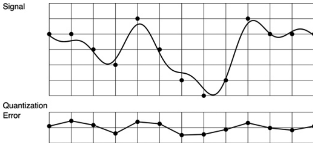
Figure 3.23: When a signal is sampled, the real-valued signal must be rounded at each sample to the nearest integer sample value. The resulting error is called quantization error ↴
