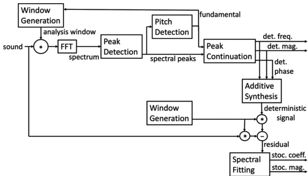
Figure 9.12: Spectral Modeling Synthesis (SMS). 🔗
