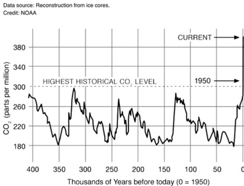
Figure 3.1: Carbon dioxide concentration data from climate.nasa.gov ↗
