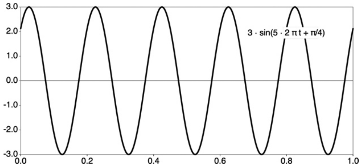
Figure 3.12: Changing the phase. 📄
