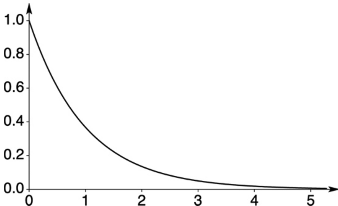
Figure 5.6: The negative exponential distribution. ↗
