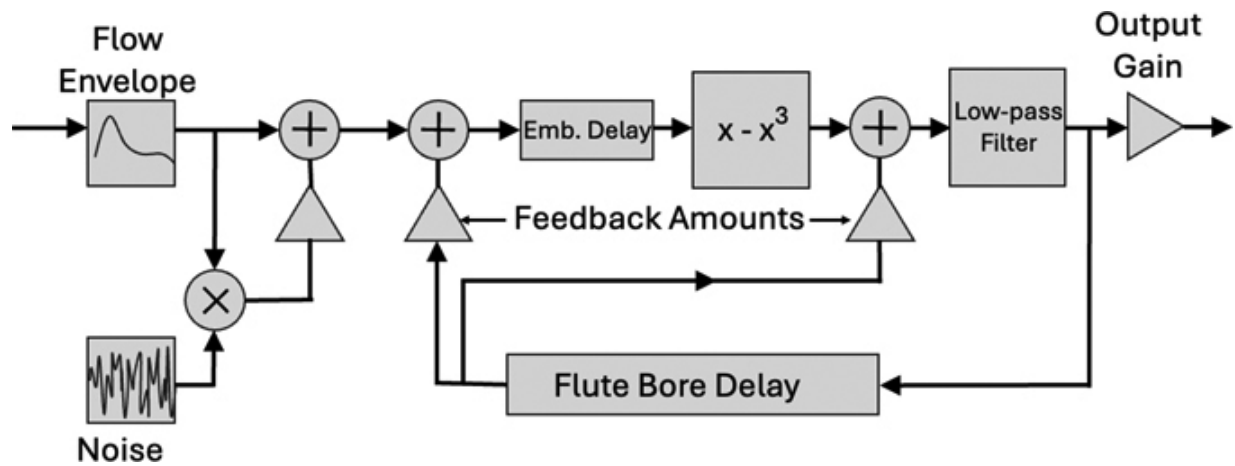
Figure 11.10: Flute Physical Model. 📄
