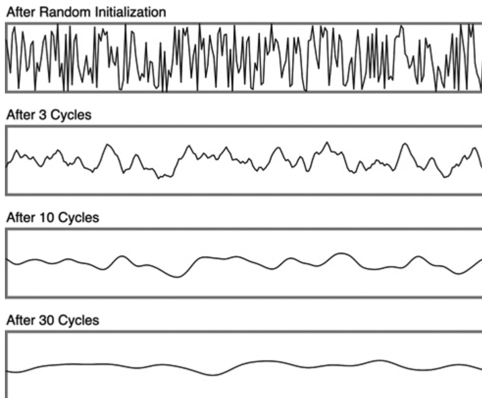
Figure 11.3: Applying the Karplus-Strong algorithm to a random waveform. After 30 passes through the filter/feedback cycle, all that’s left of the wild random noise is a gently curving wave. The result is much like what we described in a plucked string: an initially complex, periodic waveform that gradually becomes less complex over time and ultimately fades away. ↩
