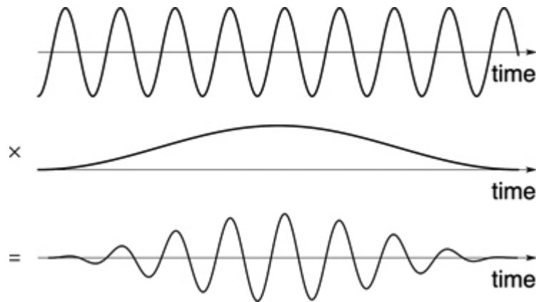
Figure 6.3: Applying a short envelope to a sound to make a grain for granular synthesis. How would a different amplitude envelope, say a square one, affect the shape of the grain? What would it do to the sound of the grain? What would happen if the sound was a recording of a natural sound instead of a sinusoid? What would be the effect of a longer or shorter envelope? 📄
