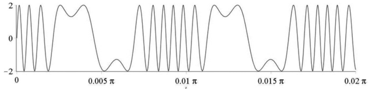
Figure 4.3: A = 2 , C = 210 Hz, D = 10 , M = 35 Hz. ↗
