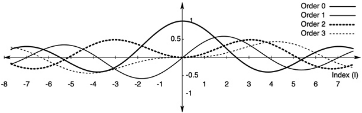
Figure 4.1: Bessel functions of the first kind, orders 0 to 3. The x axis represents the index of modulation in FM. 📄
