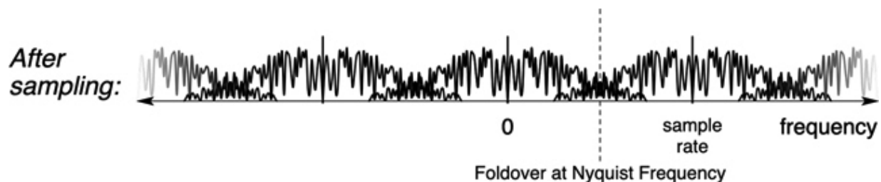
Figure 3.19: A broader spectrum (contains higher frequencies) after sampling. While shown as separate overlapping copies here, the copies are in fact summed into a single spectrum. ↗
