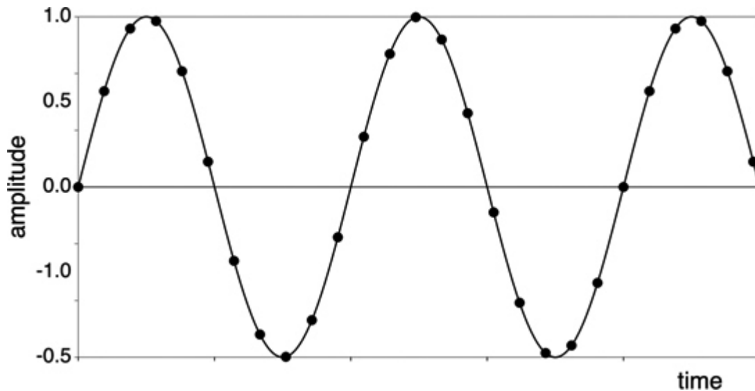
Figure 3.5: An analog waveform and its digital cousin: the analog waveform has smooth and continuous changes, and the digital version of the same waveform consists only of points along the curve. The black circles are the actual samples taken by the computer. Note that nothing in between those points is stored in the computer. ↗
