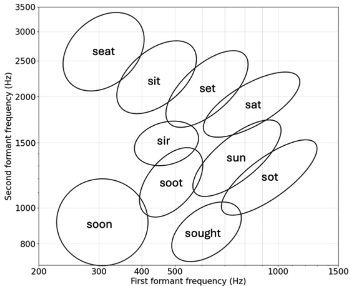
Figure 9.2: Frequency plots for vowels. ↗
