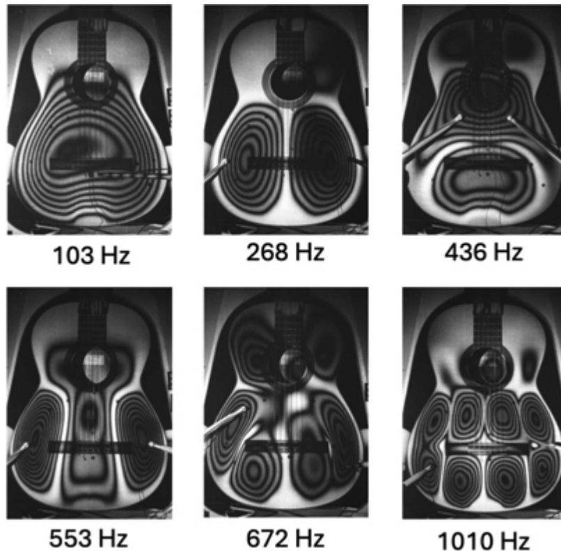
Figure 10.4: Some modes of vibration in an acoustic guitar body. Photos by Bernard Richardson, Cardiff University. 📄
