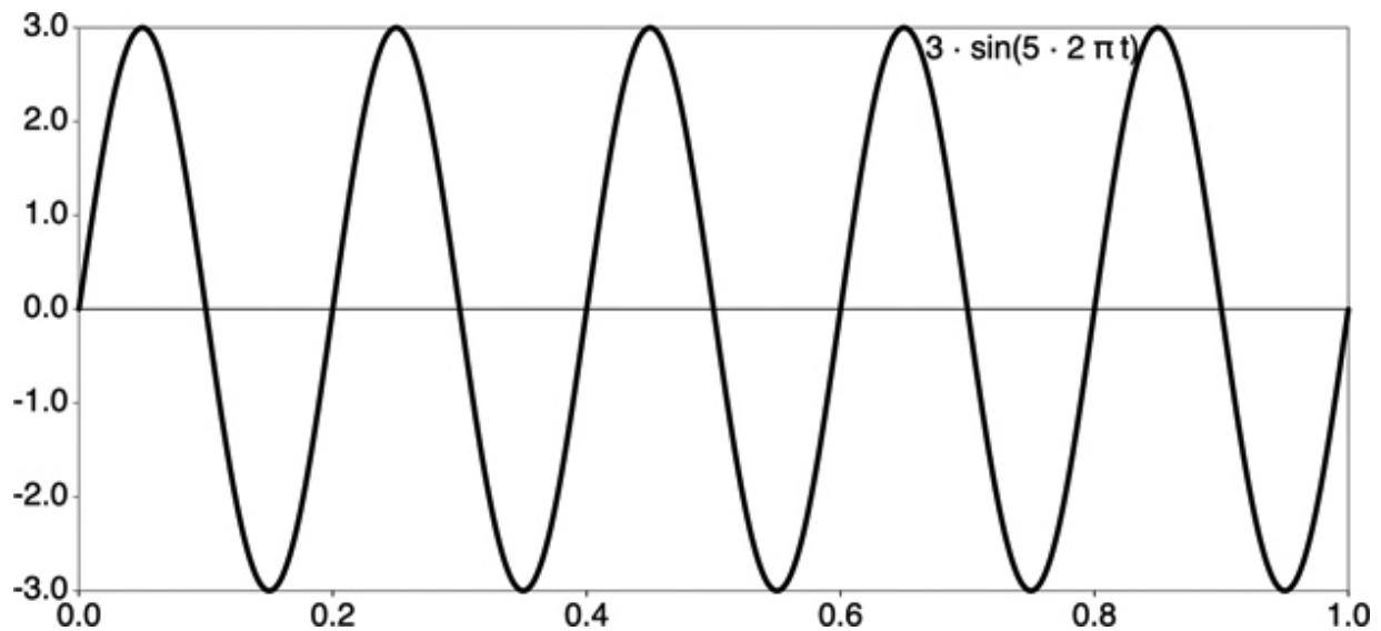
Figure 3.11: Bigger, faster sine curve. ↗
