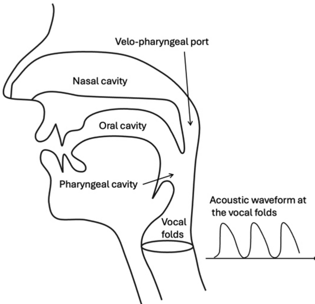
Figure 9.1: Diagram of a human head to illustrate how the voice works. The waveform at right is roughly what the “input” sound looks like coming
