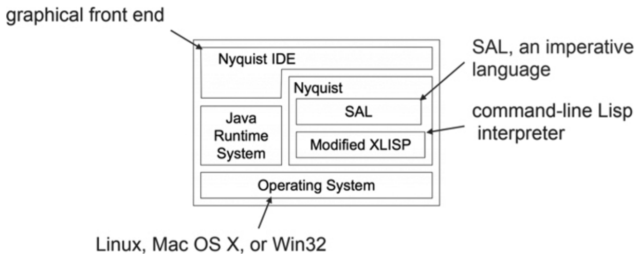
Figure 1.6: NyquistIDE System Architecture. ↗
