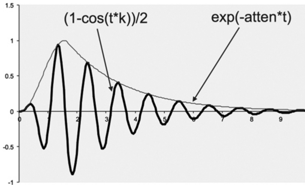
Figure 9.9: FOF. ↗
