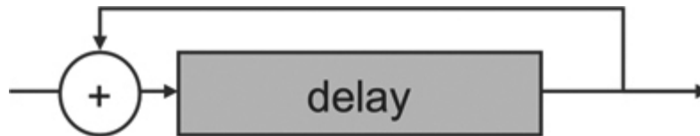
Figure 10.11: Echo algorithm in Nyquist. ↗
