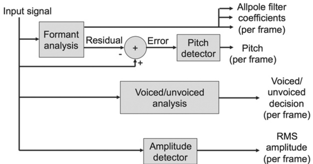
Figure 9.6: Diagram of LPC. 📄
