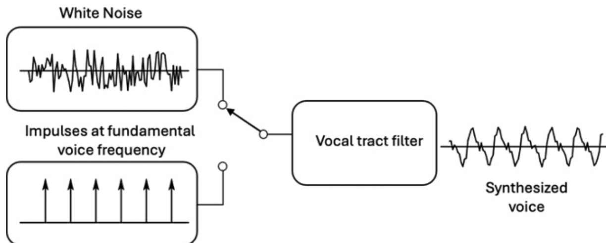
Figure 9.3: Framework of source-filter models. 📄
