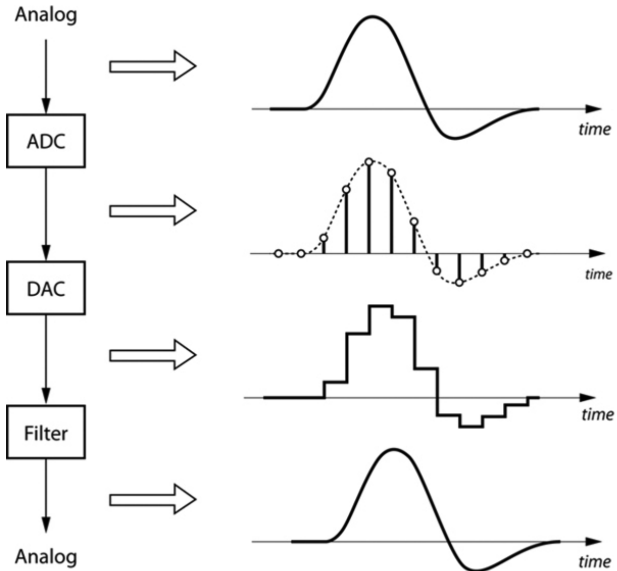
Figure 1.4: An analog waveform is converted by an ADC to digital form. Conversion back to analog is shown in two steps. First, each digital sample is converted to a voltage. Second, the signal is smoothed by a filter. (Sometimes, the filter step is assumed and the two-step process is referred to as DAC. 📄 )
