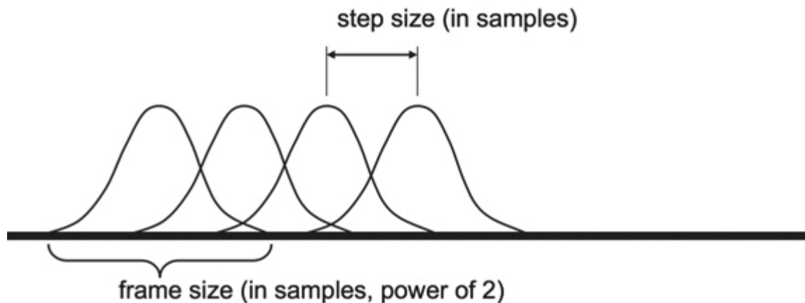
Figure 8.4: Multiple overlapping Windows. The distance between windows is the step size. ↩
