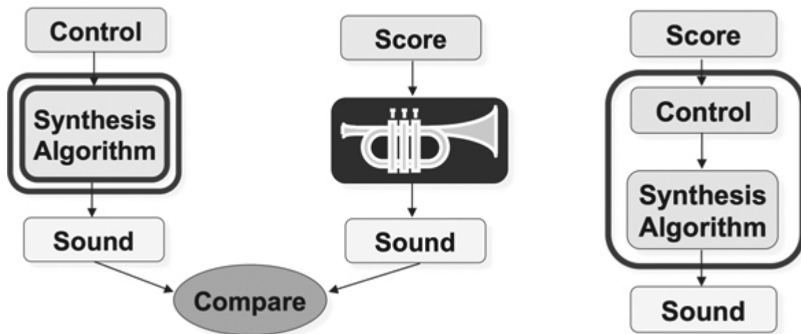
Figure 12.3: Left: Traditional approach to synthesis algorithm research and development. It is assumed that control functions are not critical and not part of the synthesis algorithm. Right: The SIS approach. Control and synthesis are considered to be related and must be developed and optimized together. Both control and synthesis are critical to good, realistic, and musical output. ↩
