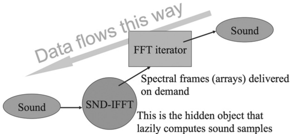
Figure 8.6: Spectral processing in Nyquist. Dependencies of sounds, unit generators, and objects are indicated by arrows. Computation is demand driven, and demand flows left-to-right following pointers to signal sources. Signal data flows right-to-left from signal sources to output signals after processing. 📄
