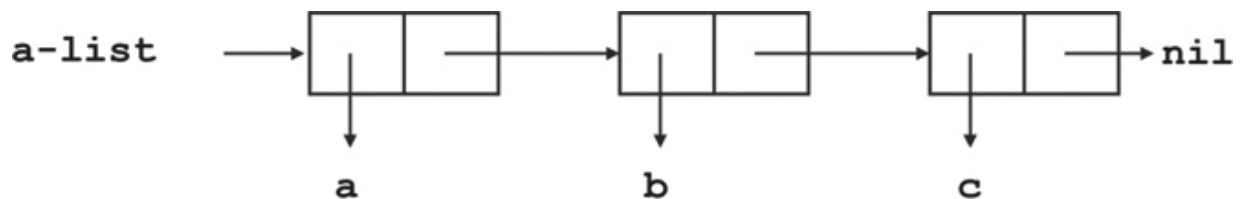
Figure 2.5: A list in Nyquist.
