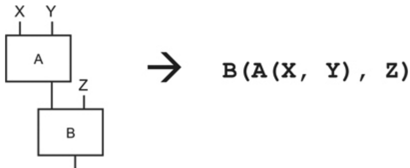
Figure 2.3: Unit generators in Nyquist. ↗
