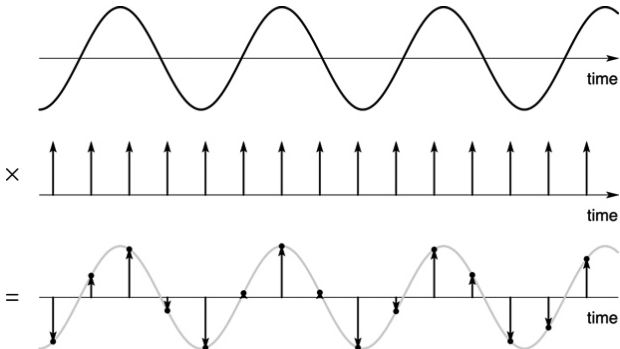
Figure 3.16: Sampling is effectively multiplication in the time domain: We multiply by 1 (or more properly an instantaneous but infinite impulse whose integral is 1) wherever we capture samples, and we remove the rest of the signal by multiplying by zero. ↩
