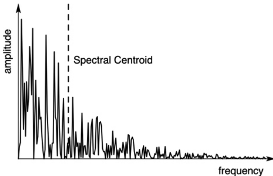
Figure 5.4: A magnitude spectrum and its spectral centroid (dashed line). If you were to cut out the spectrum shape from cardboard, it would balance on the centroid. The spectral centroid is a good measure of the overall placement of energy in a signal from low frequencies to high. ↩
