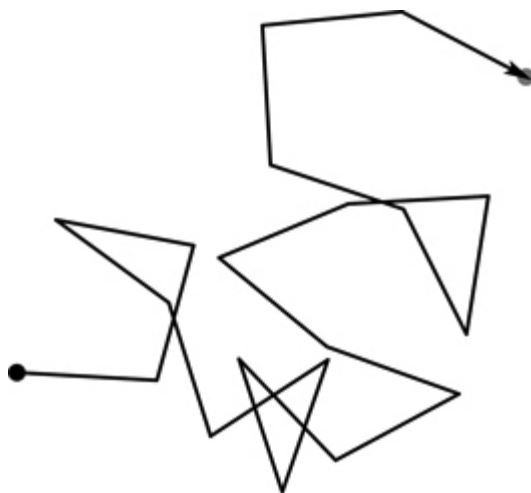
Figure 5.7: A random walk in two dimensions. Each step has the same length, but the direction is random. ↗
