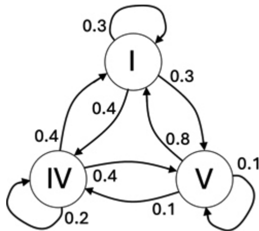
Figure 5.8: A Markov Chain for simple chord progressions with labeled transition probabilities. For example, the V chord is very likely (0.8) to transition to the I chord. 📄
