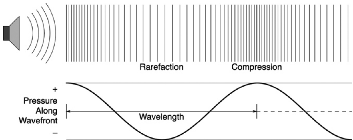
Figure 1.1: Illustration of a wave and the corresponding pressure variations in the air at an instant in time. At any given point, pressure varies with time as the wave passes through the point at the speed of sound. ↗
