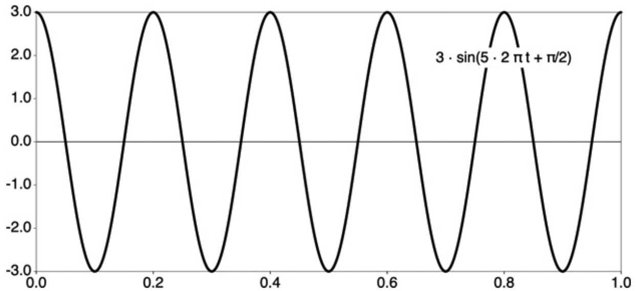
Figure 3.13: Changing the phase. 📄
