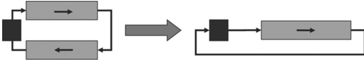
Figure 11.6: McIntyre Woodhouse model consisting of a delay representing sound traveling through the bore of a clarinet and a filter representing the losses over the round trip. The figure shows that the single delay is equivalent to a bi-directional waveguide with perfect reflection at one end. ↩
