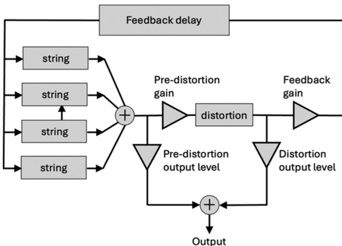
Figure 11.13: Feedback is achieved by feeding some of the output through a delay and back into each string model. ↩
