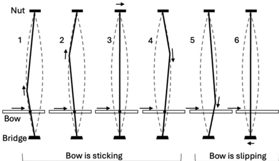
Figure 11.5: A bowed string is pulled by the bow when the bow sticks to the string (1 through 4). At some point the bow does not have enough friction to pull the string further, and the string begins to slip. The sliding reduces the friction on the string, which allows it to stretch in opposition to the bowing direction (5 and 6). Finally, the stretching slows the string and the bow sticks again, repeating the cycle. ↩
