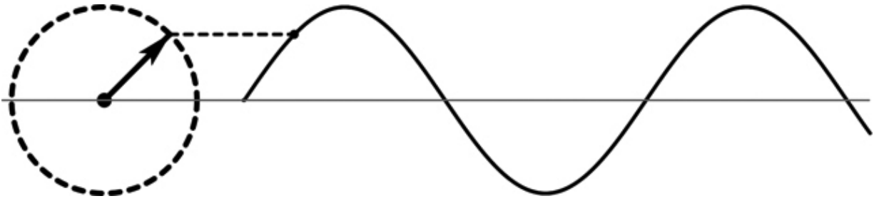
Figure 3.7: Sine waves and phasors. As the sine wave moves forward in time, the arrow goes around the circle at the same rate. The height of the arrow (that is, how far it is above or below the x-axis) as it spins around in a circle is described by the sine wave. ↱
