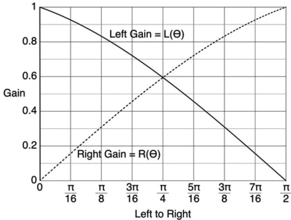
Figure 10.17: The -4.5 dB pan law. ↗
