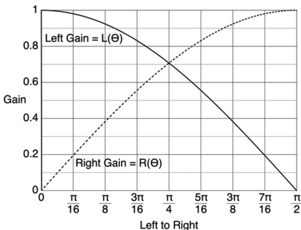
Figure 10.16: Constant power panning. ↗
