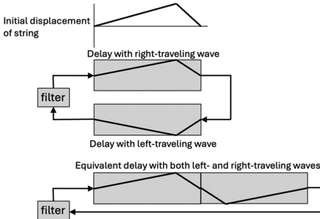
Figure 11.14: Initializing the string. The physical string shape contains both left- and rightgoing waves so we need to combine them to get a full round-trip initial waveform. ↗
