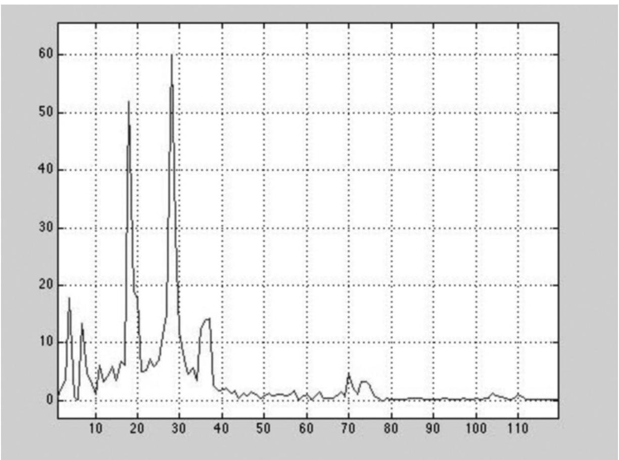
Figure 3.14: Changing the phase. ↗
