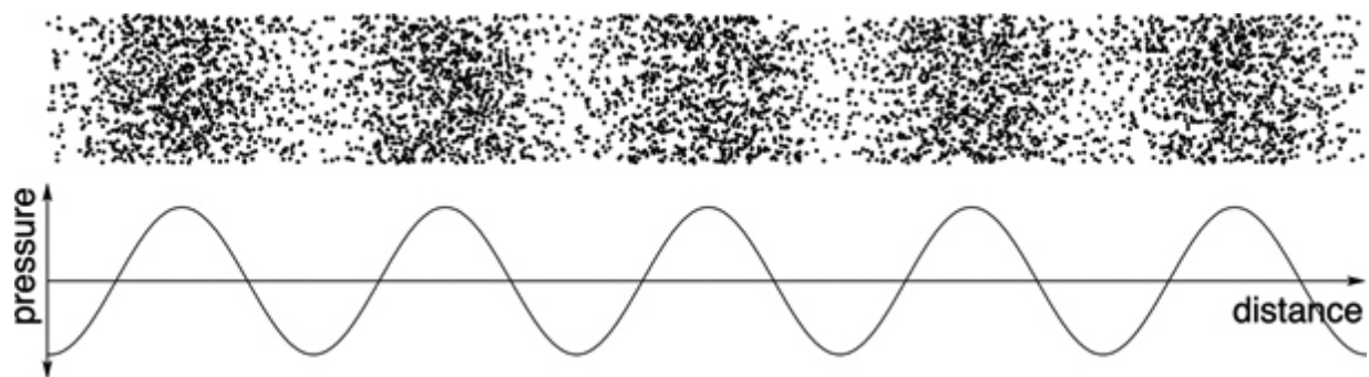
Figure 10.1: Sound is vibration or air pressure fluctuations. The top illustrates a snapshot of air molecules as a sinusoidal sound wave passes from left to right. The pressure is shown in the graph below (the “zero” axis represents local air pressure). In reality, air molecules are much more dense, and the density variation is much too small to see even if you could see air molecules! ↗
