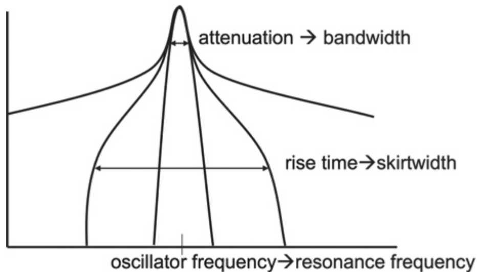
Figure 9.10: FOF in the frequency domain. ↗
