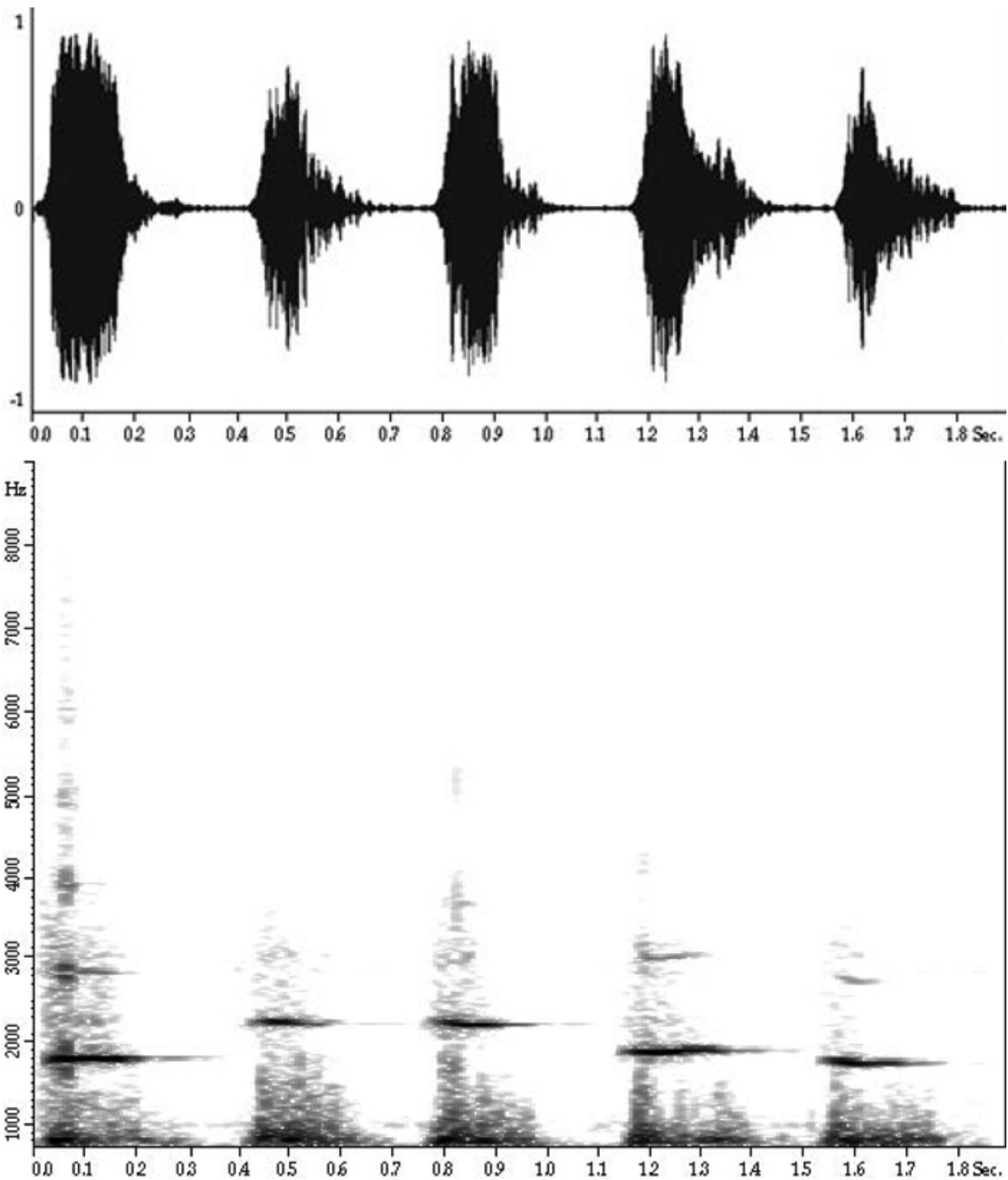
Figure 3.6: Two graphical representations of sound. ↗
