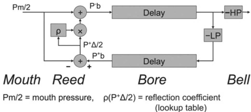
Figure 11.7: Clarinet model. ↗
