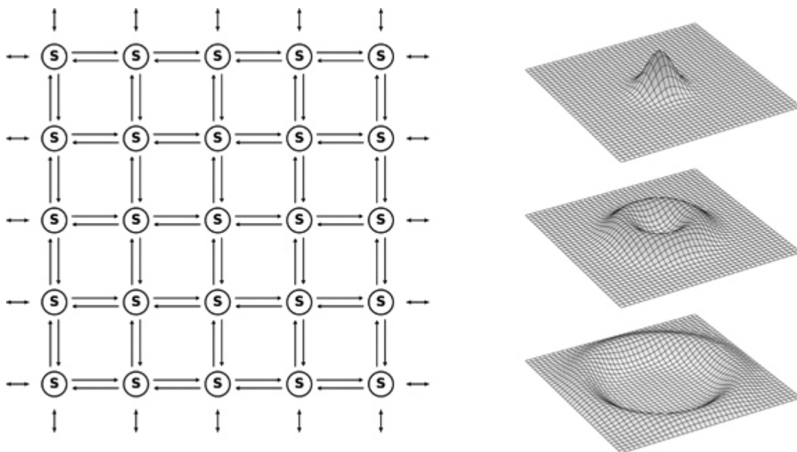
Figure 11.16: 2D Waveguide Mesh and some simulation results. 📄
