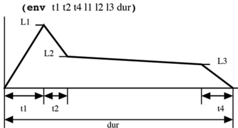
Figure 2.6: Envelope function env .
