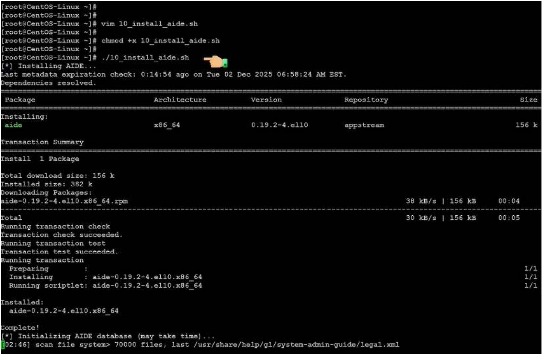
Figure 4.7: Installing AIDE and creating the initial integrity baseline
