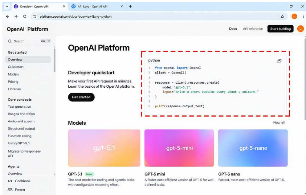
Figure 3.7: Python example and model choices in the OpenAI Platform
