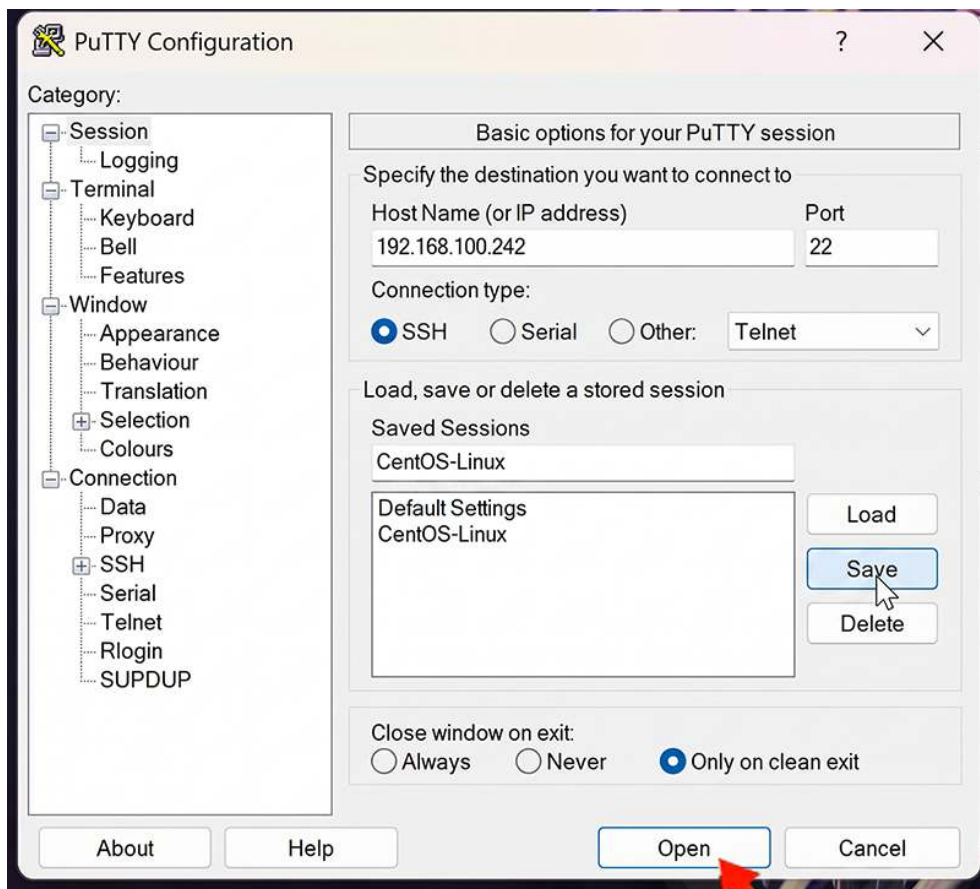
Figure 2.17: PuTTY configuration window
