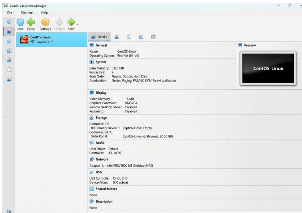
Figure 2.8: VirtualBox Manager showing the newly created CentOS Linux VM and its hardware summary
