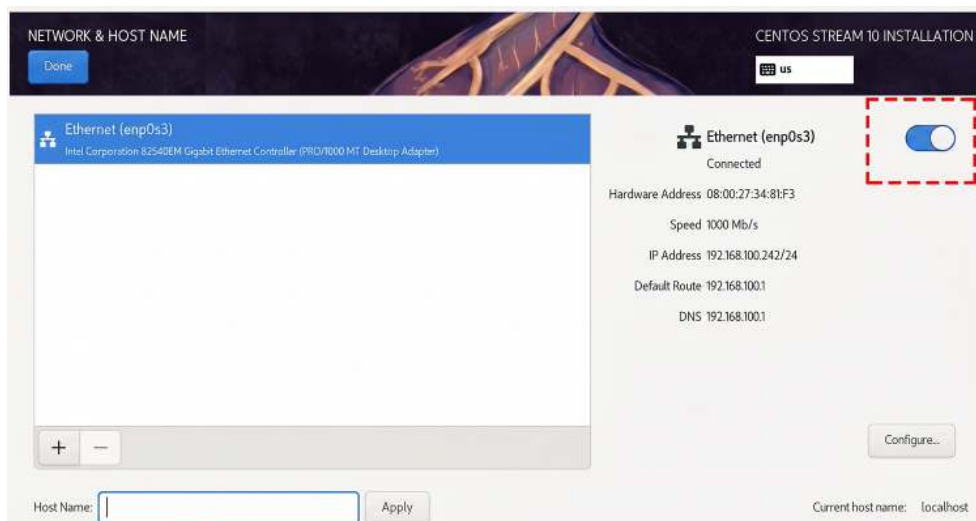
Figure 2.13: CentOS Network & Host Name screen showing Ethernet enabled
