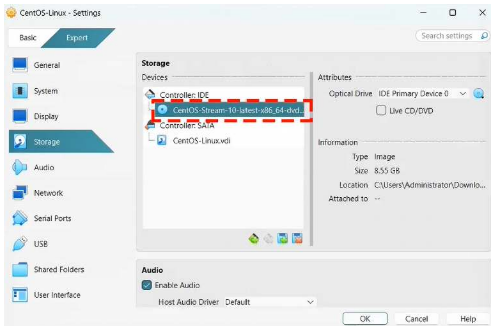
Figure 2.10: VirtualBox storage settings showing the CentOS Stream ISO attached to the virtual optical drive
