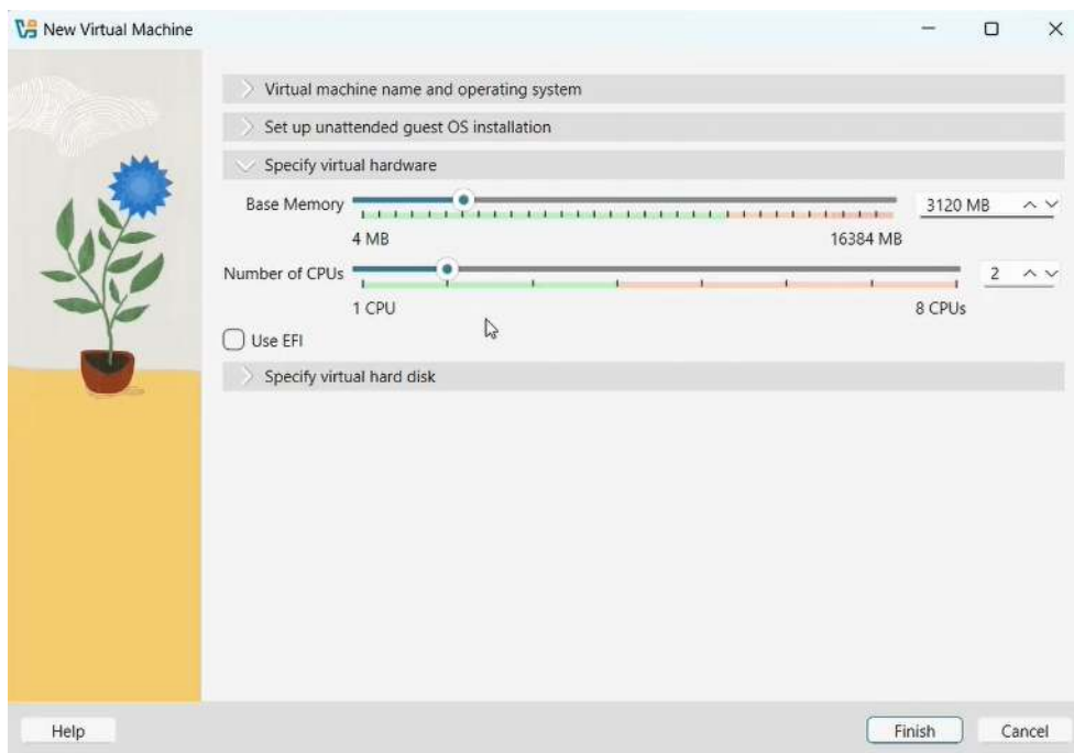
Figure 2.7: VirtualBox virtual hardware settings showing memory and CPU allocation
