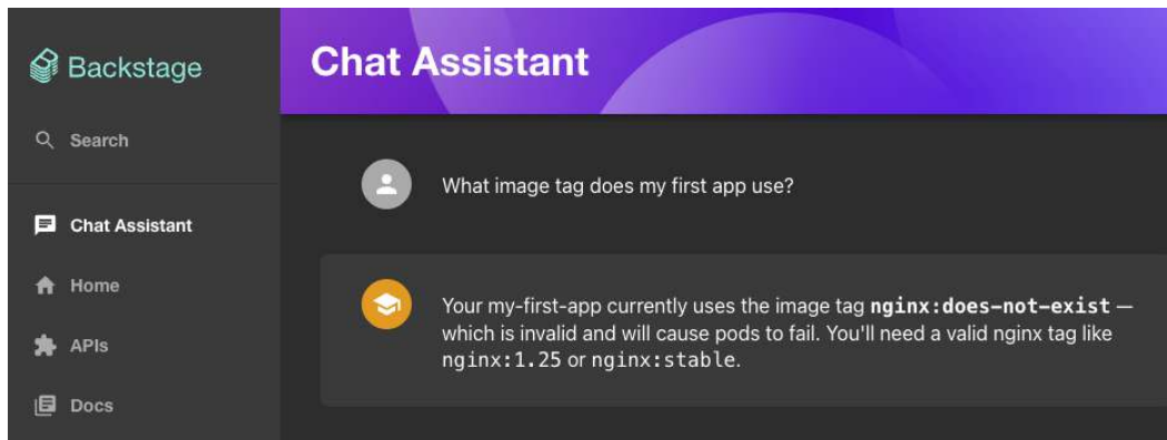
Figure 7.3: The assistant reporting my-first-app's current image tag
