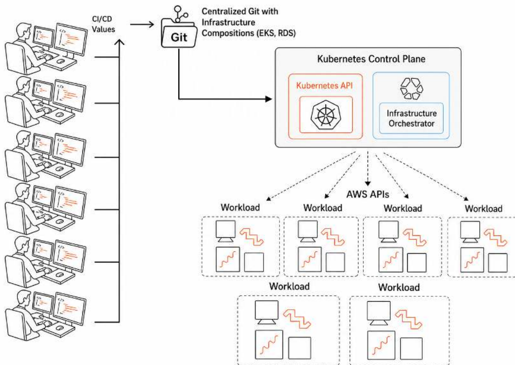
Figure 1.1: Using Kubernetes as a control plane (Kubernetes operators)
