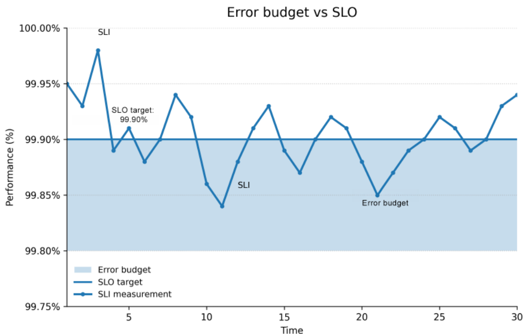
Figure 1.2: Error budget versus SLO (service level objective)
