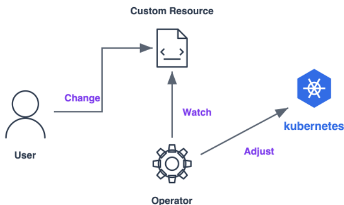
Figure 5.1: The Kubernetes Operator pattern: a user declares intent in a custom resource, and the Operator adjusts the cluster to match
