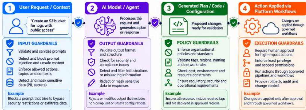
Figure 8.4: Guardrail layers across the AI interaction lifecycle
