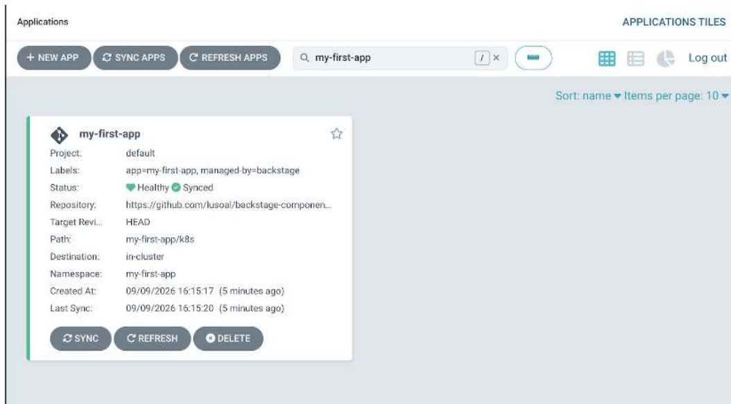
Figure 5.7: Argo CD showing my-first-app synced and healthy after the pull request is merged
