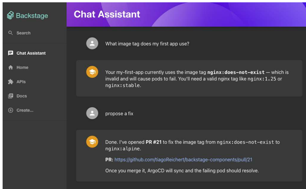
Figure 7.5: The chat assistant created a pull request
