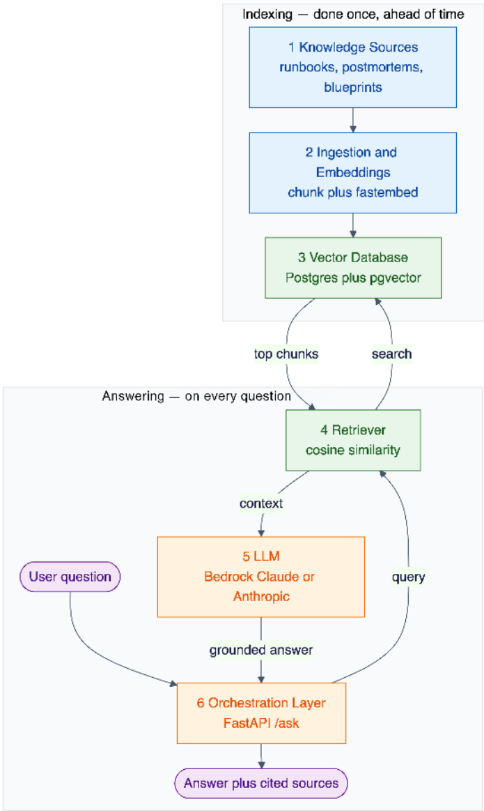
Figure 4.1: The six components of a RAG pipeline, shown as an offline indexing path and an online answering path
