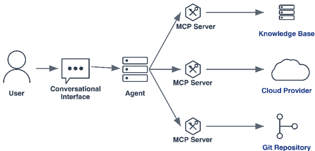
Figure 5.4: The full conversational path, with an agent reaching a knowledge base, a cloud provider, and Git through separate MCP servers
