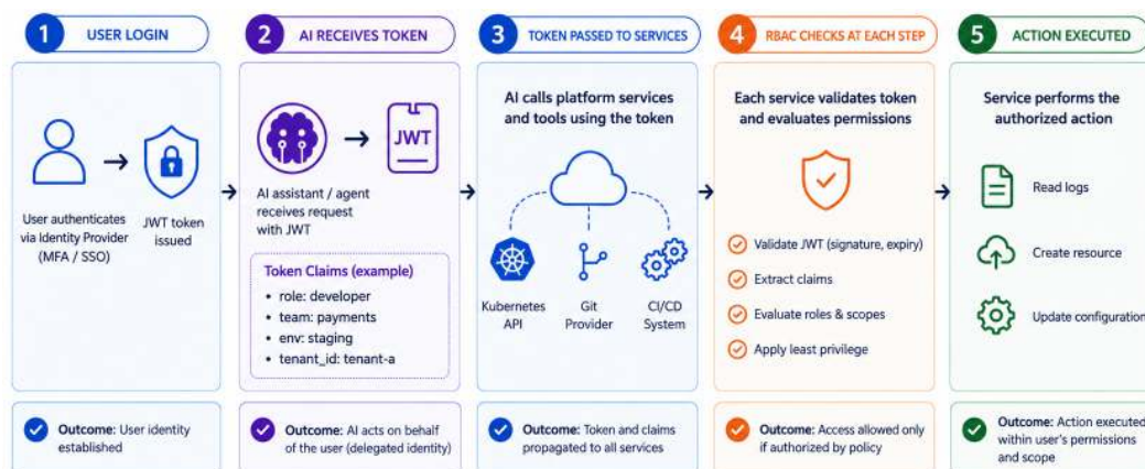
Figure 8.6: Identity propagation and authorization across AI-driven platform workflows
