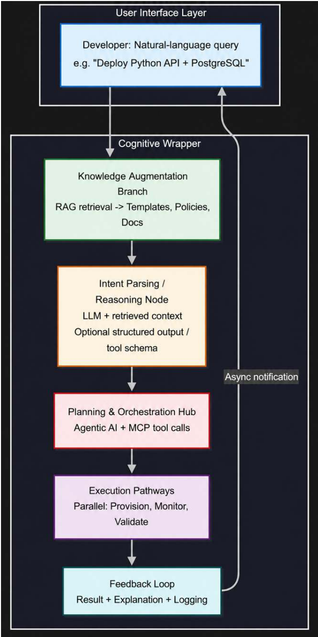
Figure 3.3: Platform engineering AI call flow
