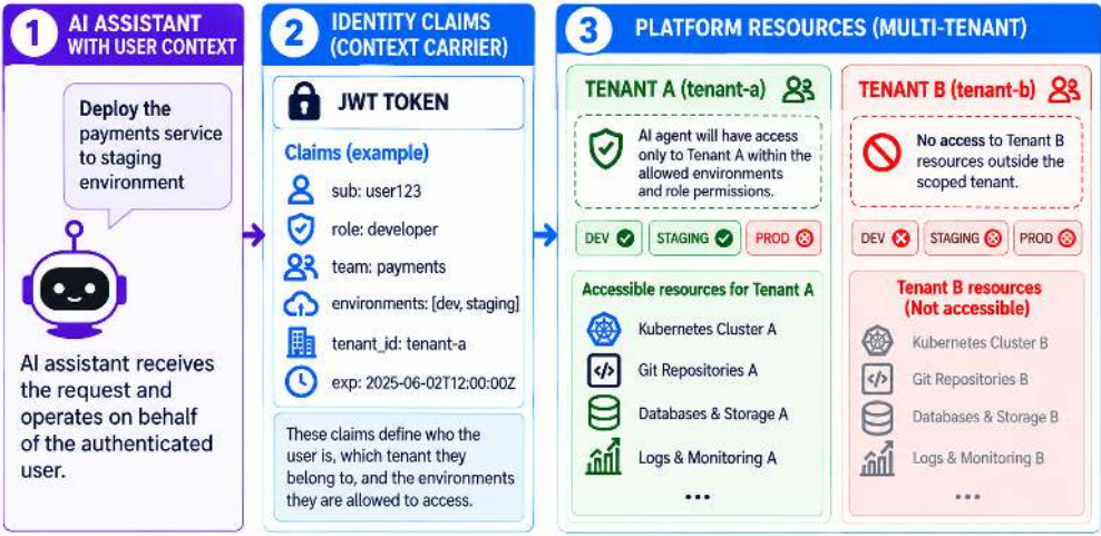
Figure 8.9: Tenant-aware authorization using identity claims and resource ownership
