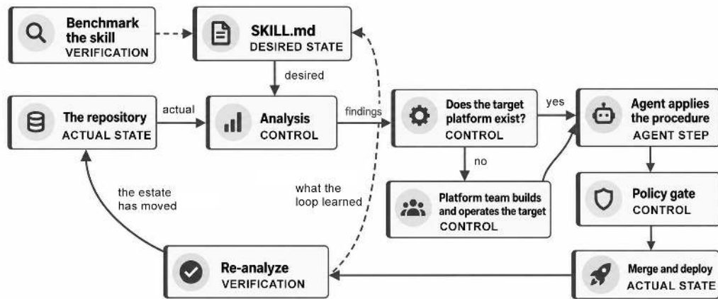
Figure 9.1: Continuous modernization as a reconciliation loop, which closes only when the platform the fix lands on already exists and somebody is operating it
