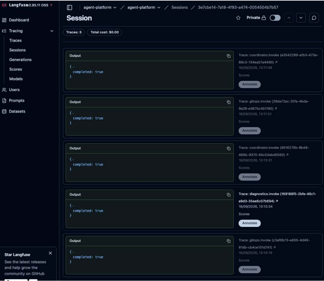
Figure 7.7: Langfuse session with multiple traces (specialist agents)
