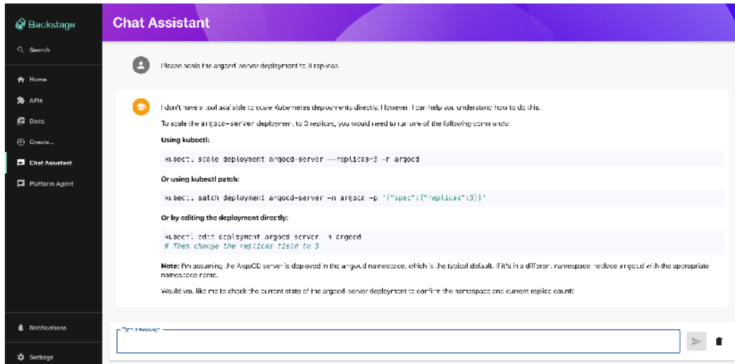
Figure 5.11: The assistant declining to modify a deployment because no write action is registered
