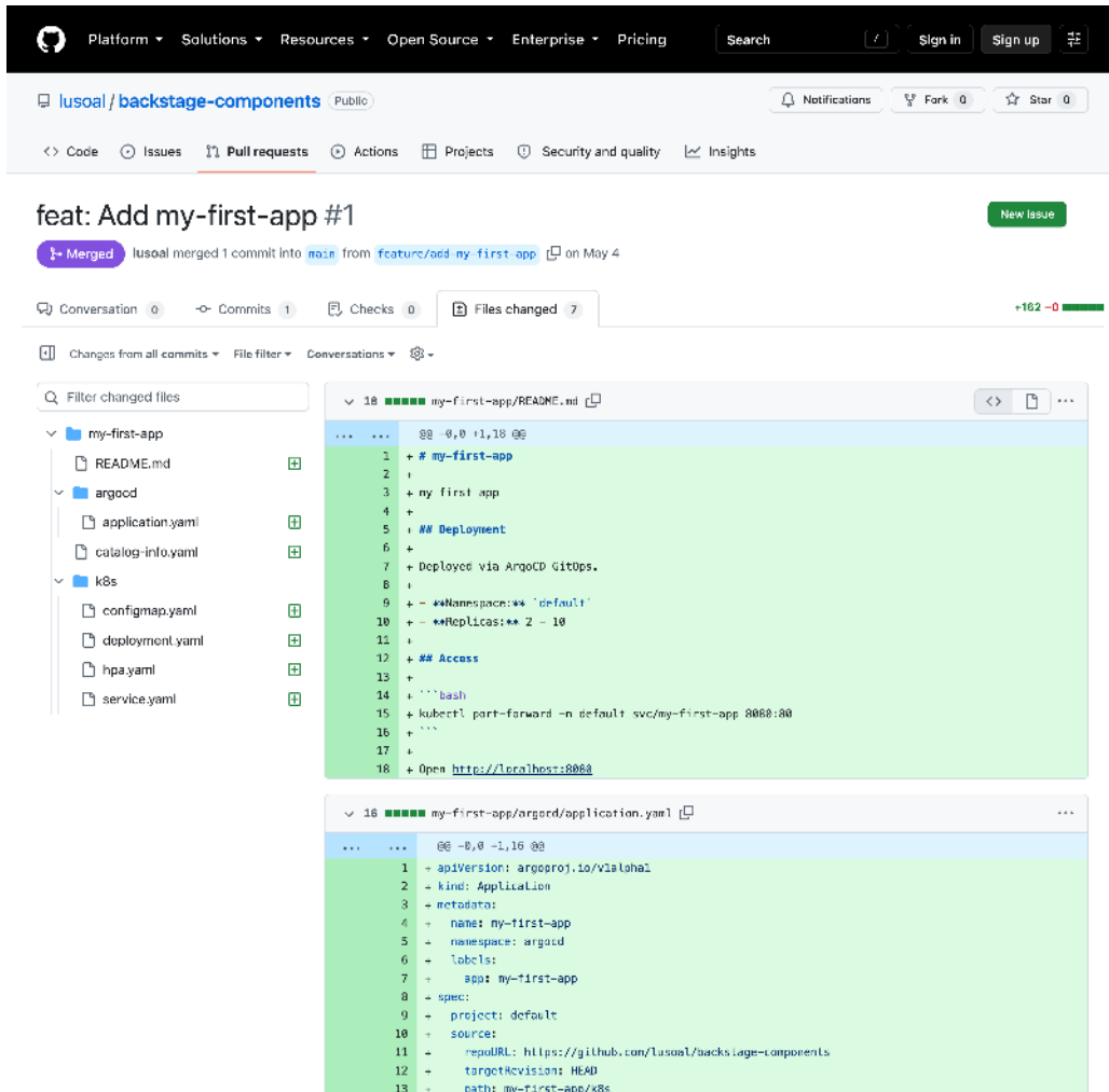
Figure 5.6: The pull request opened by the Backstage template, carrying the generated Kubernetes manifests
