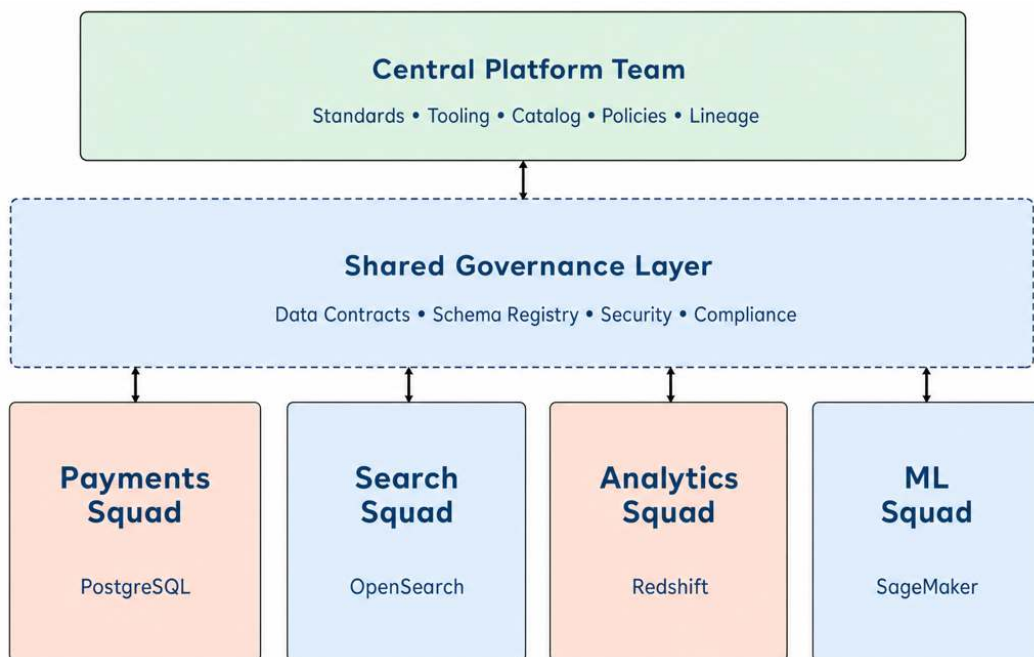
Figure 2.3: Hybrid data governance model combining central standards with domain ownership
