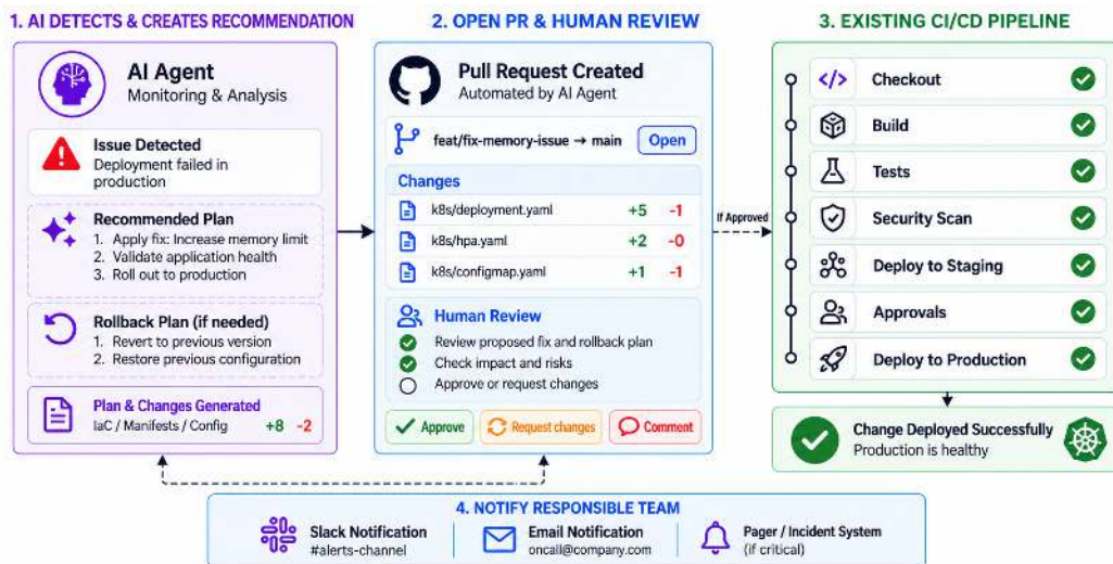
Figure 8.3: Guarded remediation workflow with human review and CI/CD validation
