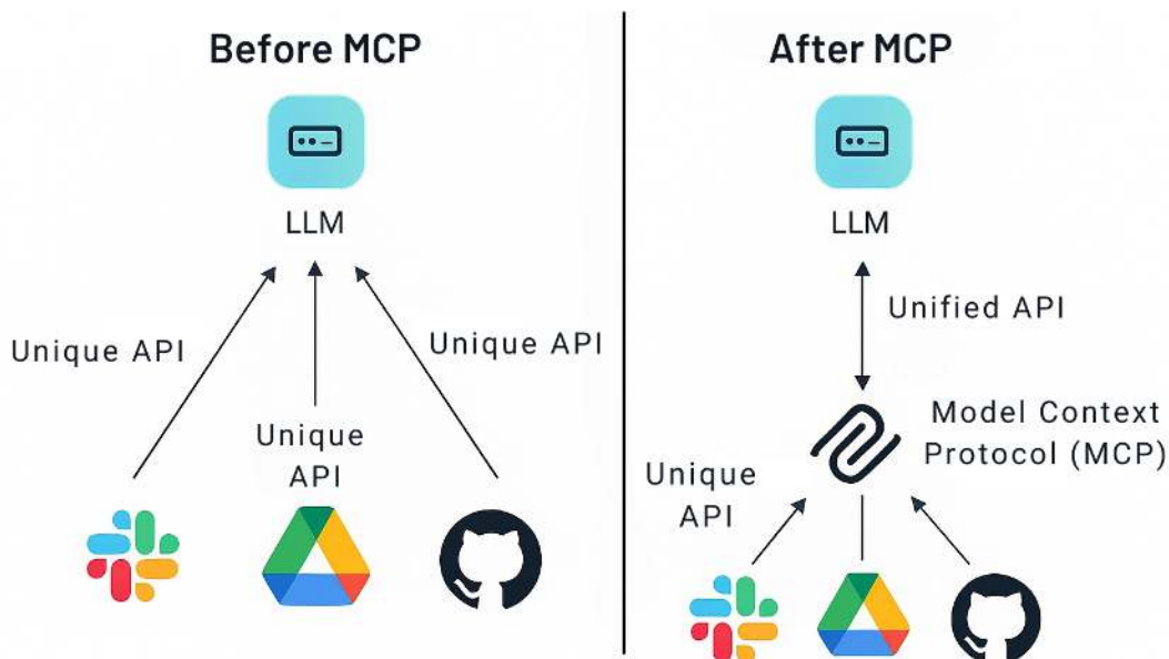
Figure 3.2: Tool integrations before and after MCP
