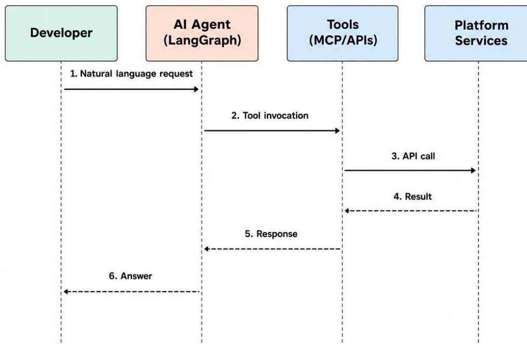
Figure 2.4: Conversational AI agent interaction flow in a developer portal
