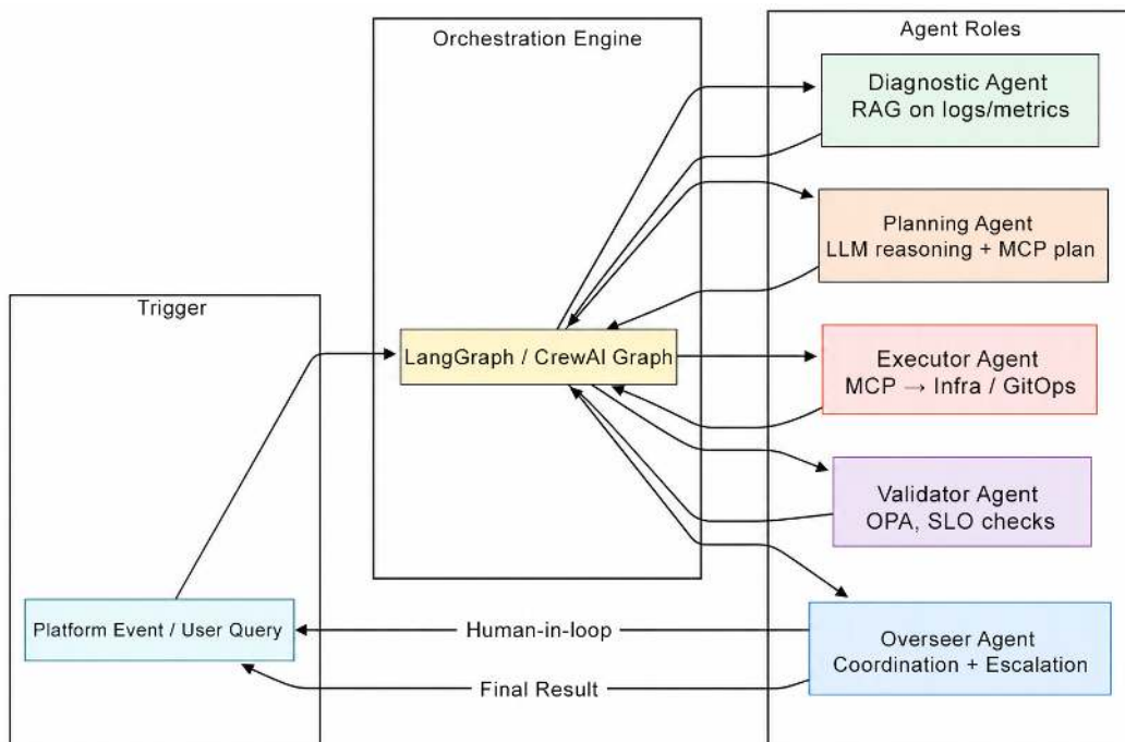
Figure 3.5: Agentic AI workflow (multi-agent orchestration)
