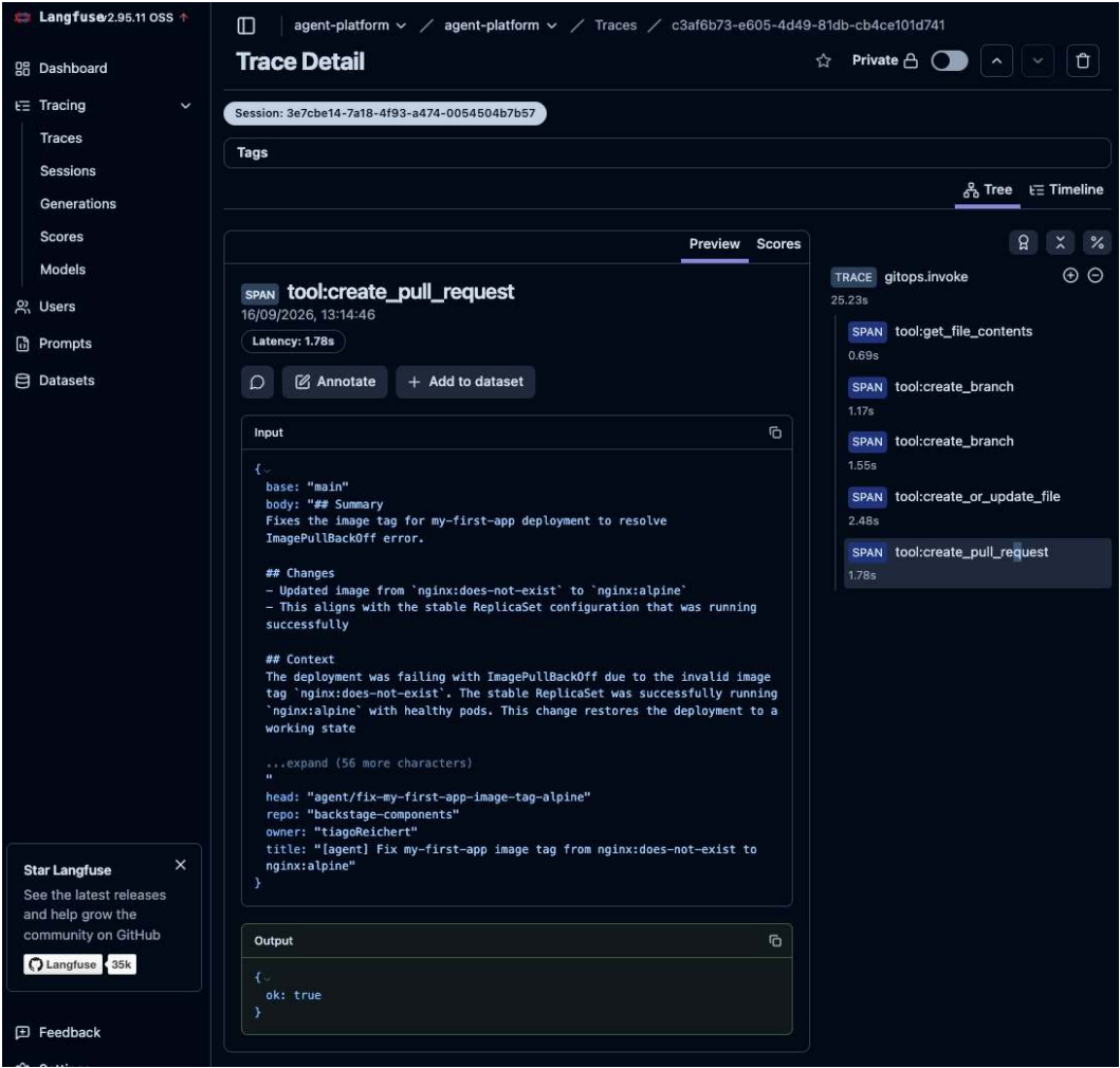
Figure 7.8: A single trace expanded (GitOps specialist agent)
