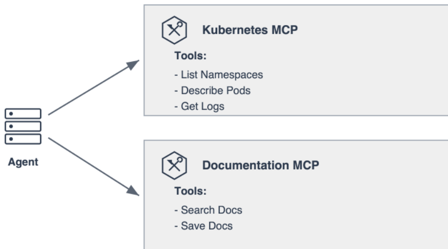
Figure 5.2: An agent reaching platform capabilities through MCP servers, each exposing a narrow, explicitly defined set of tools
