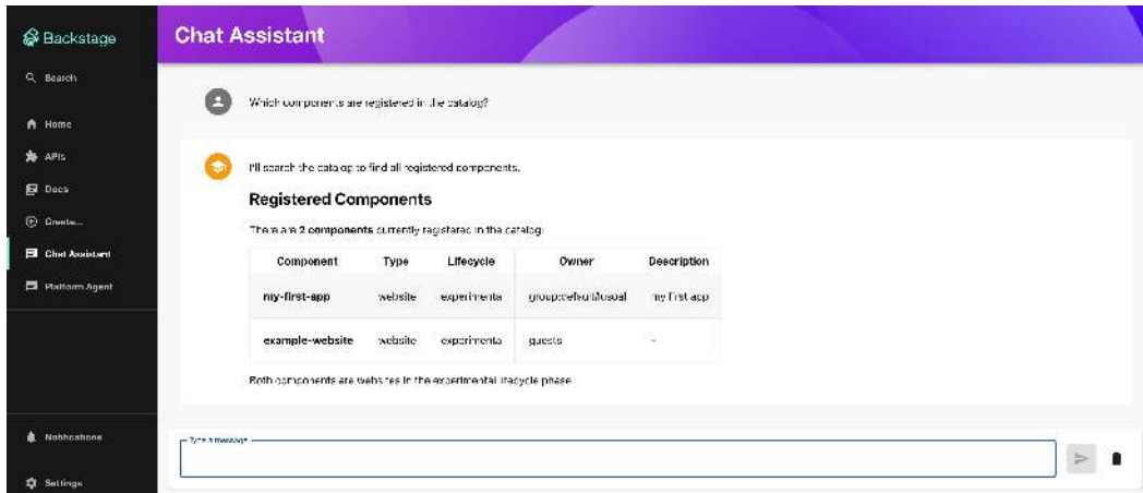
Figure 5.9: The assistant answering from real catalog entities after the Backstage actions are registered
