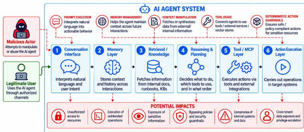
Figure 8.10: Attack surface of an AI agent system
