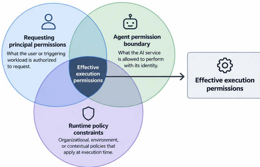
Figure 8.7: Effective execution permissions across requester, agent, and runtime policy constraints
