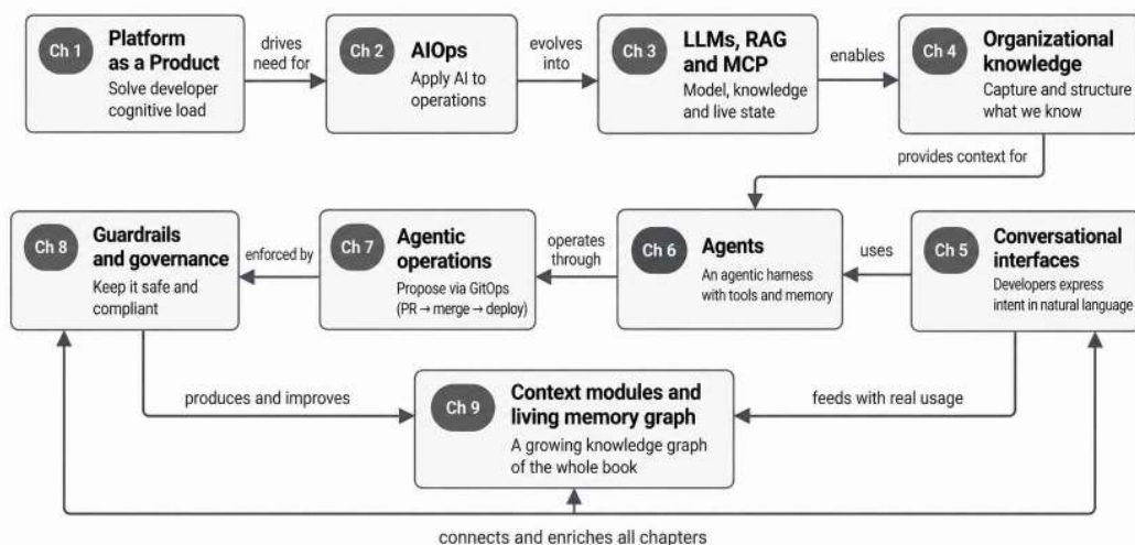
Figure 9.2: The spine of the living memory graph
