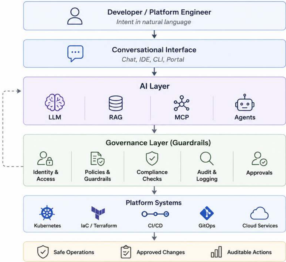
Figure 8.1: Governance layers for AI-driven platform workflows
