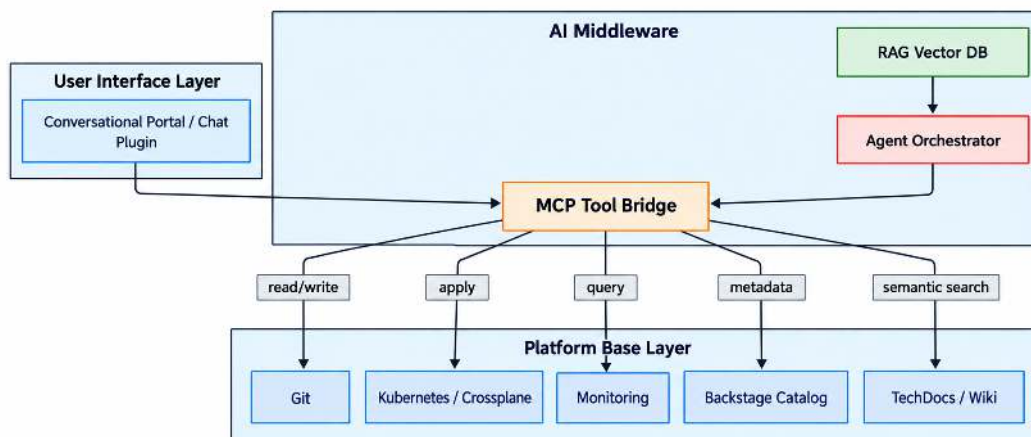
Figure 3.4: AI platform engineering high-level architecture
