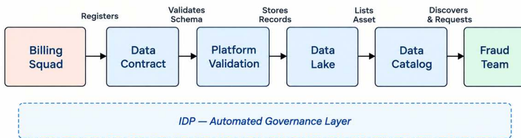
Figure 2.1: End-to-end data governance flow on an internal developer platform
