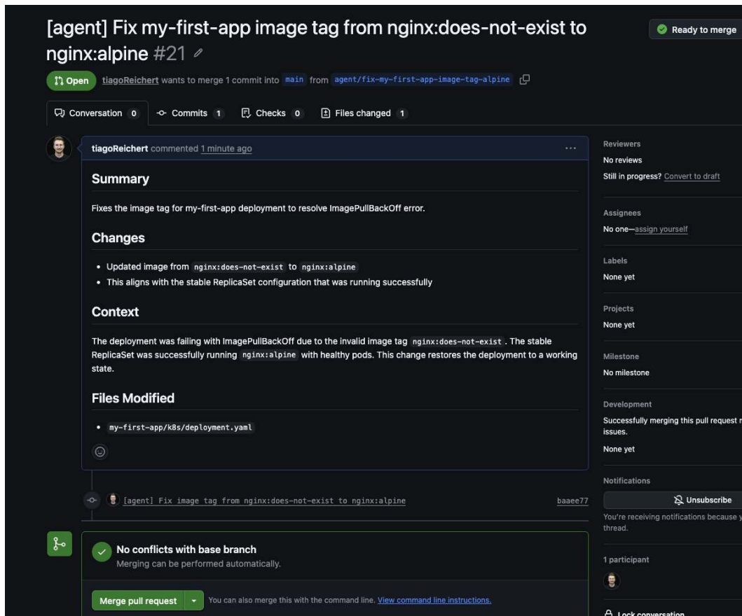
Figure 7.9: GitHub pull request opened by the agent
