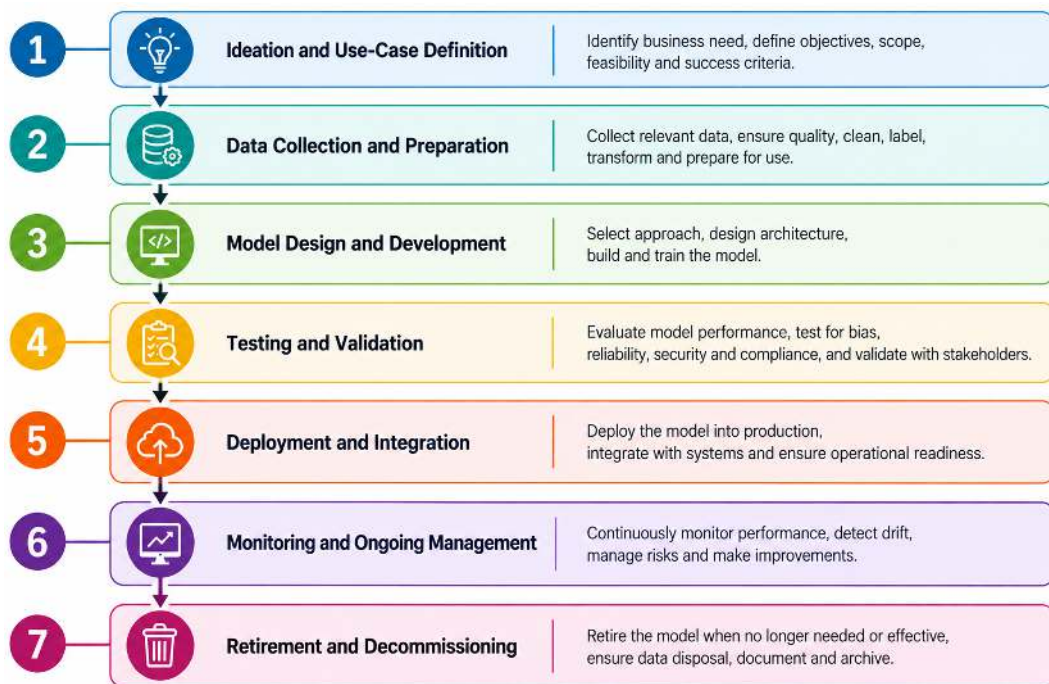
Figure 14.2: AI lifecycle
