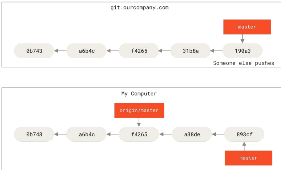
Figure 31. Local and remote work can diverge
