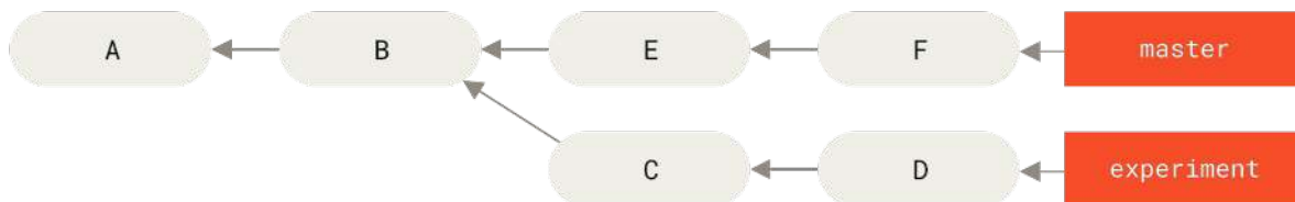
Figure 136. Example history for range selection
