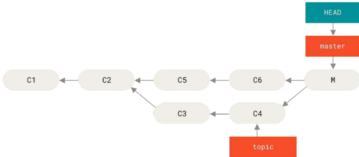
Figure 155. Accidental merge commit
