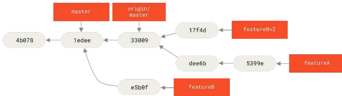
Figure 71. Commit history after featureBv2 work
