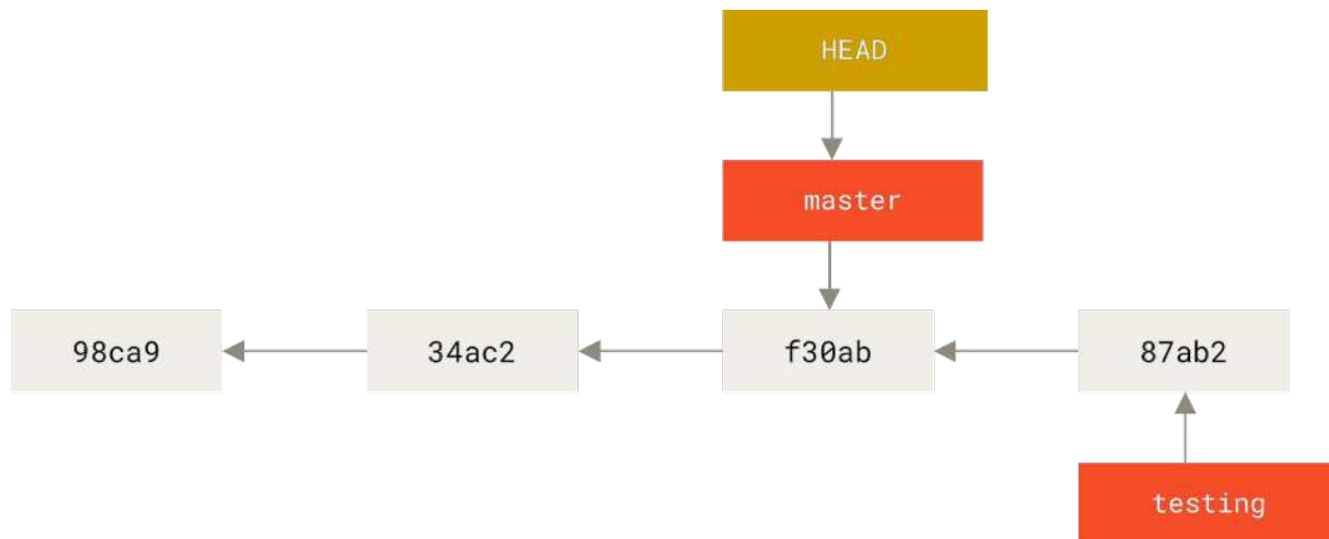
Figure 16. HEAD moves when you checkout
