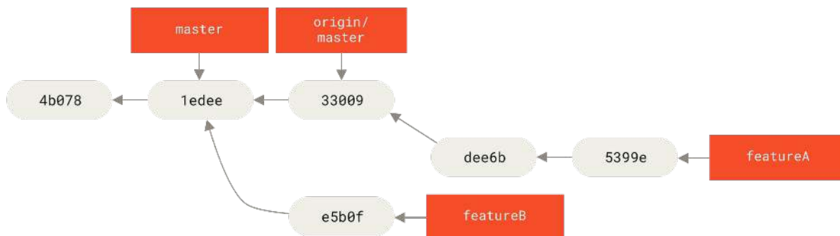
Figure 70. Commit history after featureA work
