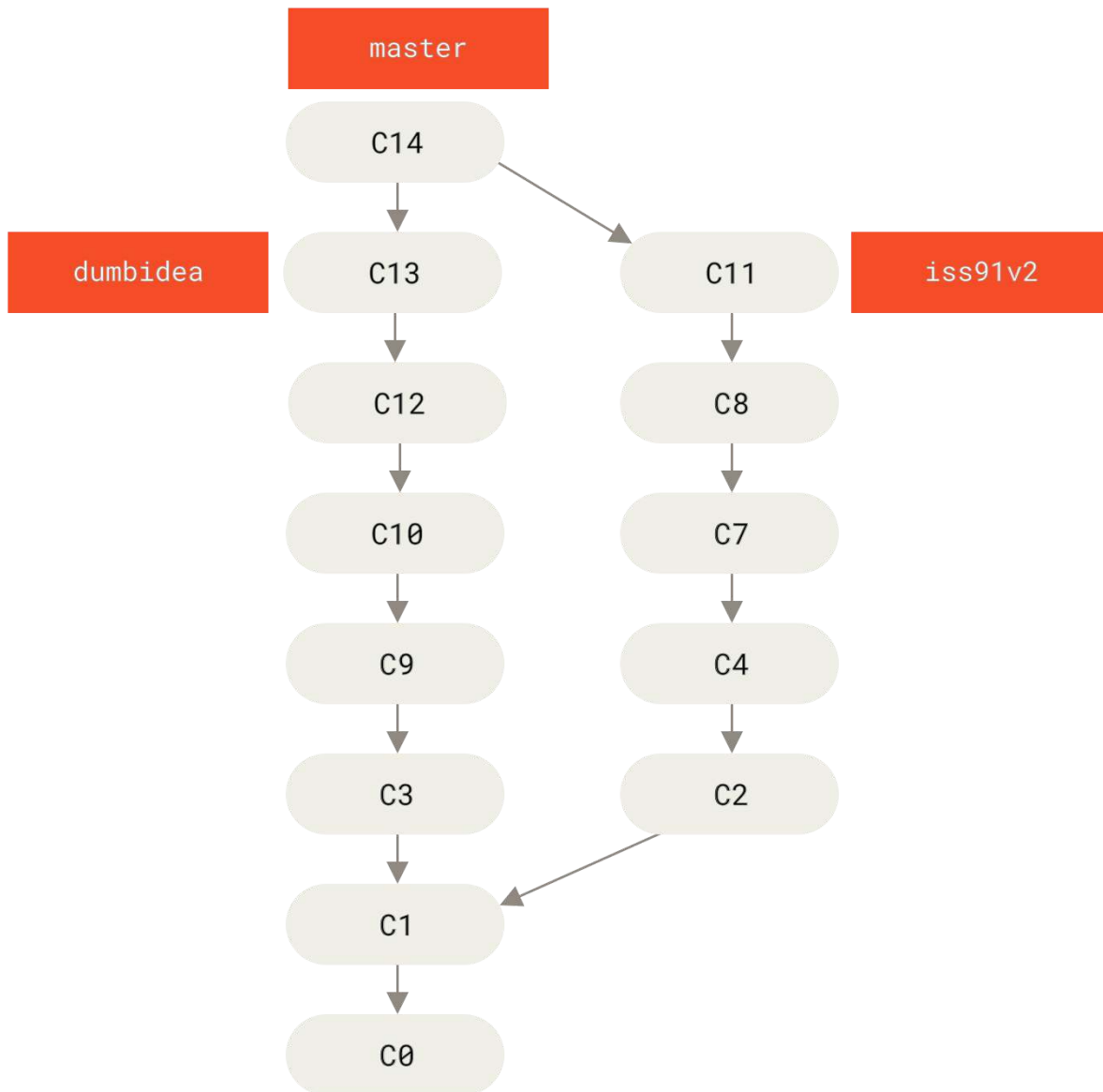
Figure 29. History after merging dumbidea and iss91v2
