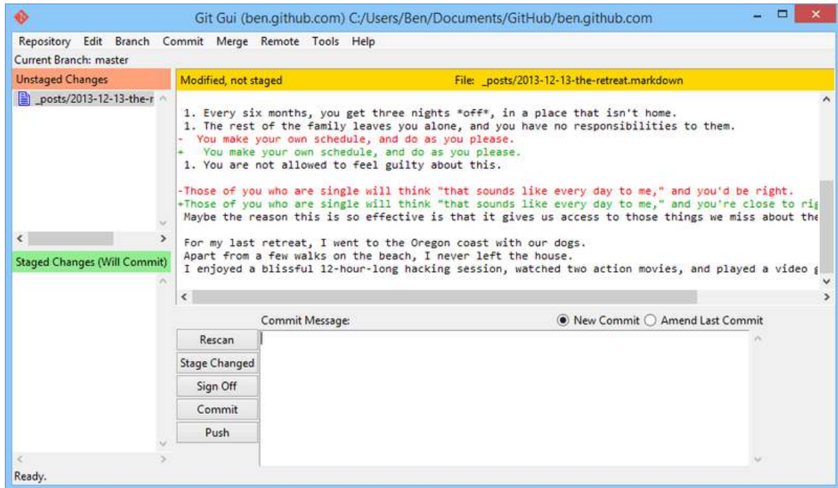
Figure 178. The git-gui commit tool
