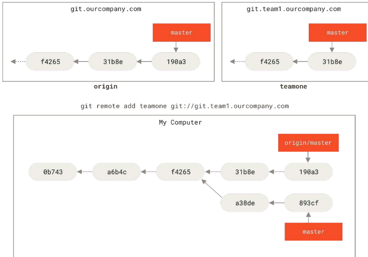
Figure 33. Adding another server as a remote
