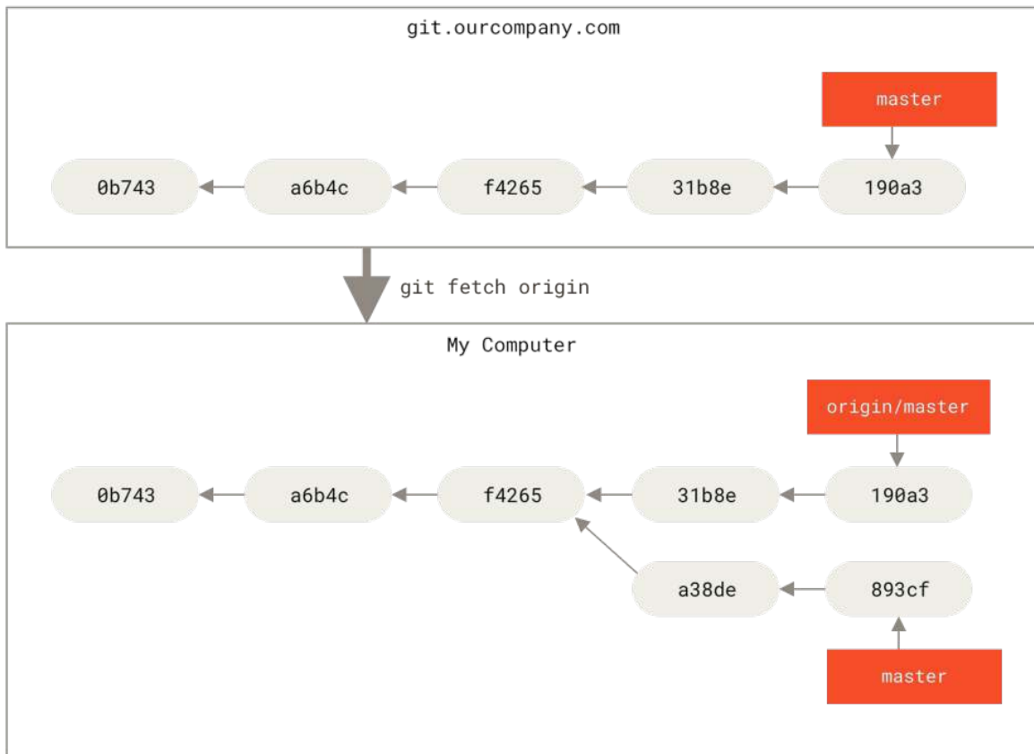
Figure 32. git fetch updates your remote-tracking branches
