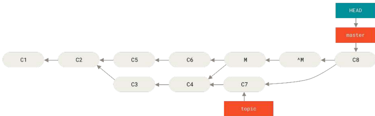
Figure 158. History with a bad merge
