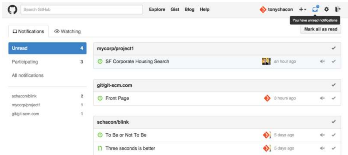
Figure 121. Notification center
