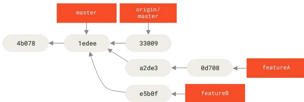
Figure 69. Initial commit history with featureB work
