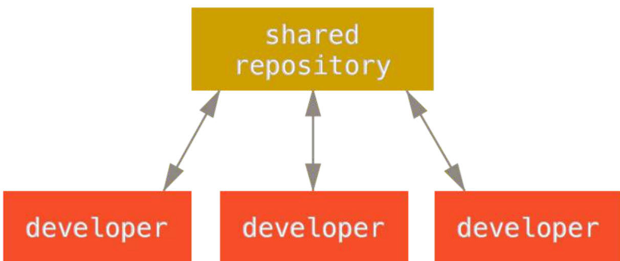
Figure 53. Centralized workflow
