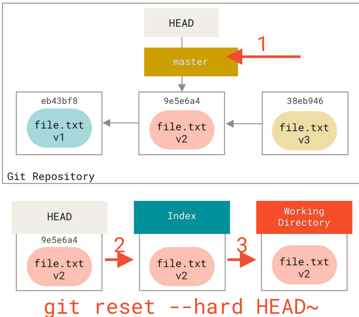
Figure 147. Hard reset
