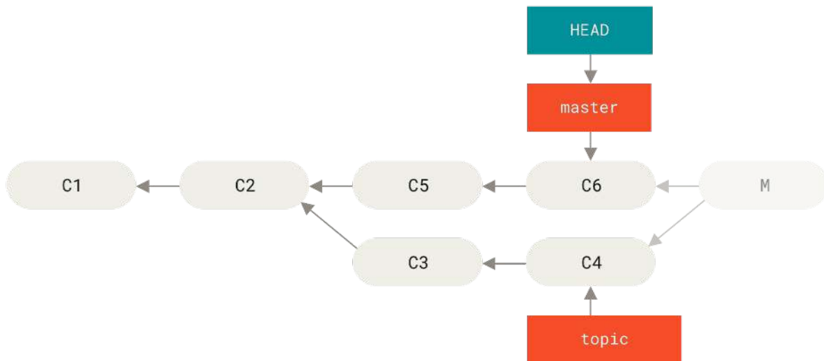
Figure 156. History after git reset --hard HEAD~
