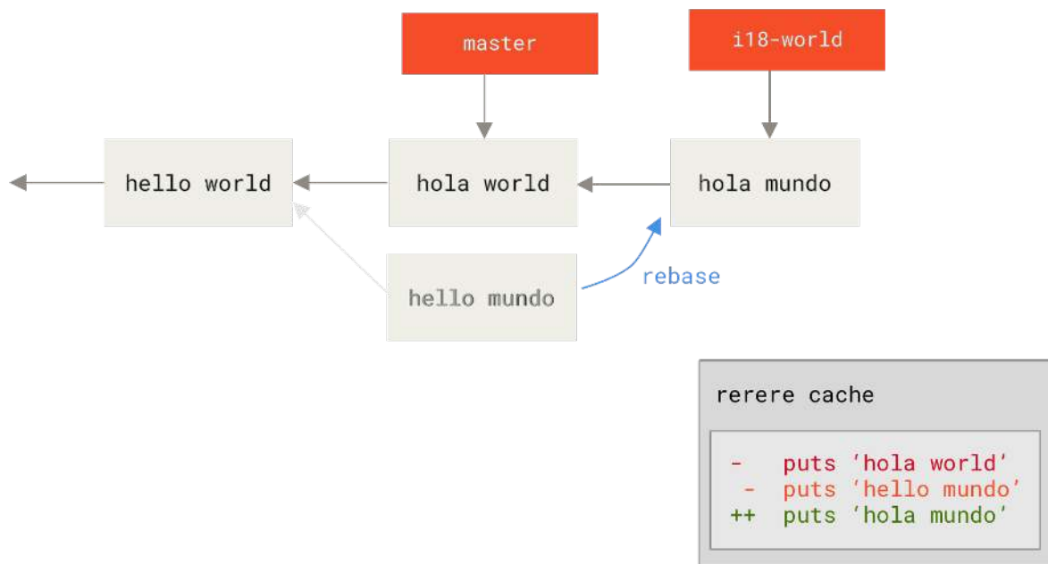
Figure 162. Automatically resolved merge conflict using previous resolution
