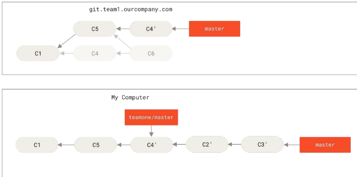
Figure 48. Rebase on top of force-pushed rebase work
