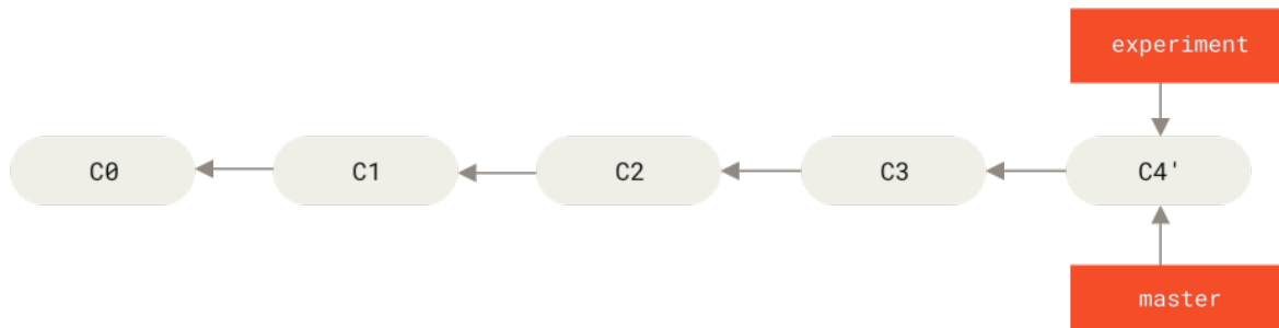
Figure 38. Fast-forwarding the master branch
