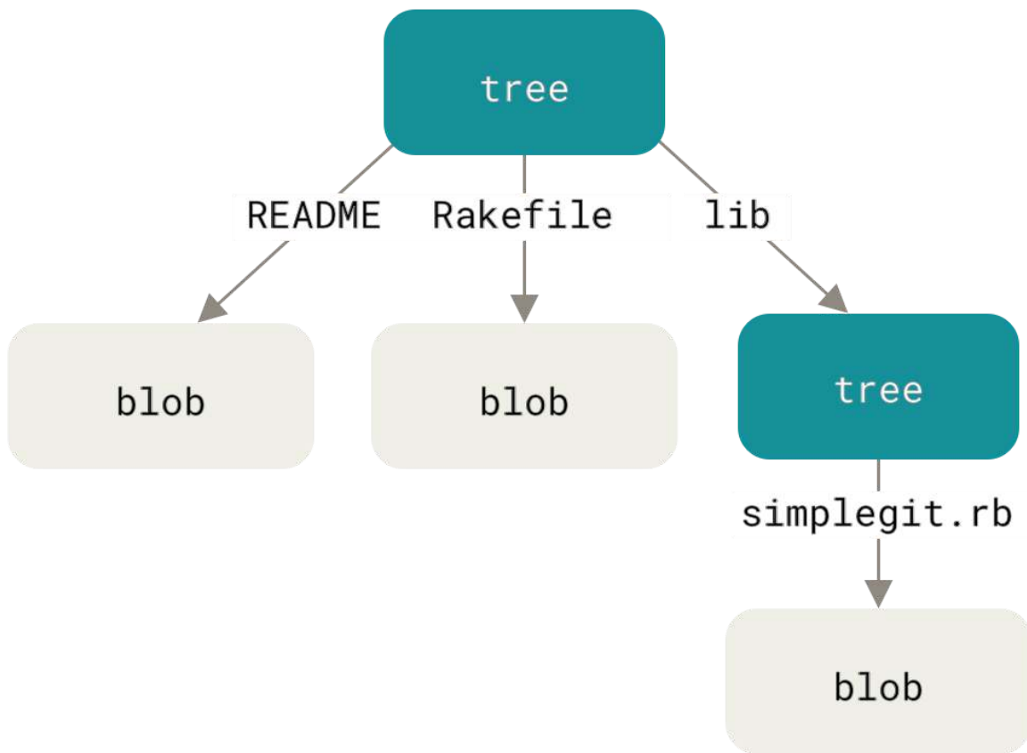
Figure 173. Simple version of the Git data model
