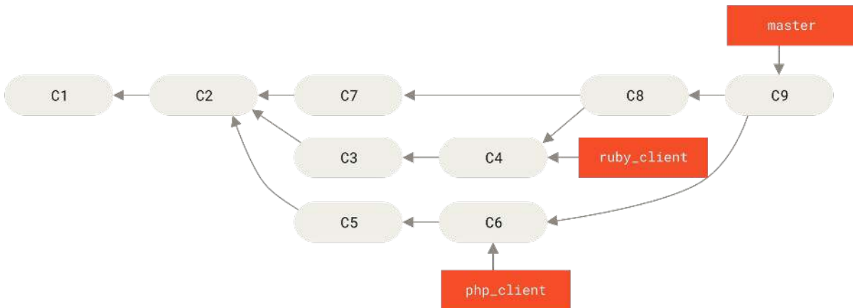
Figure 73. After a topic branch merge
