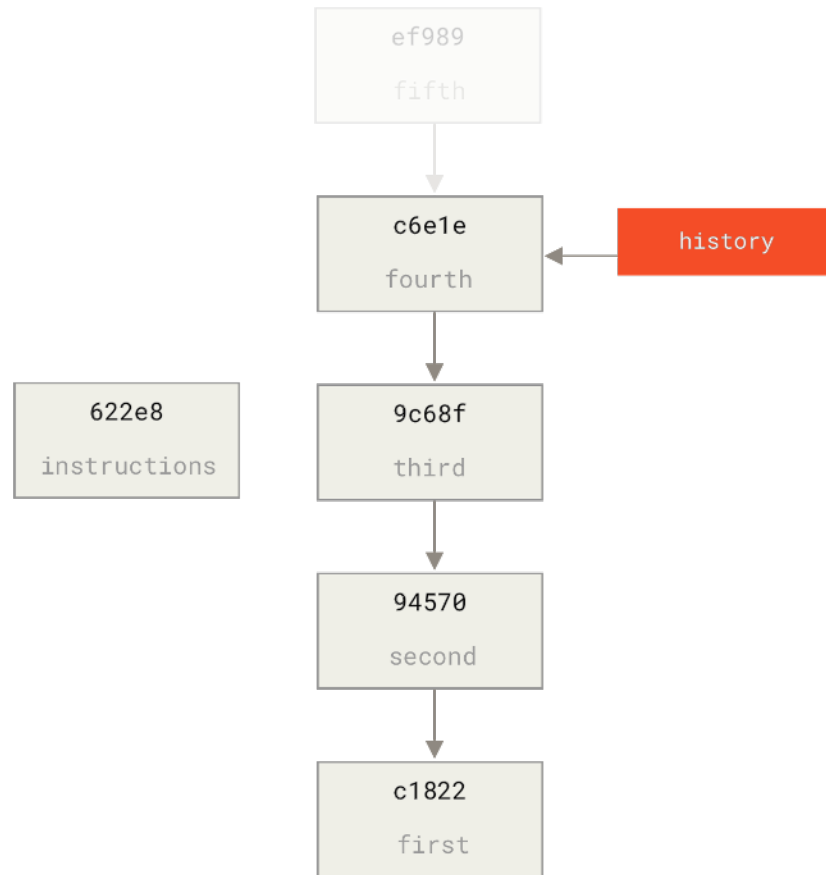
Figure 165. Creating a base commit using commit-tree
