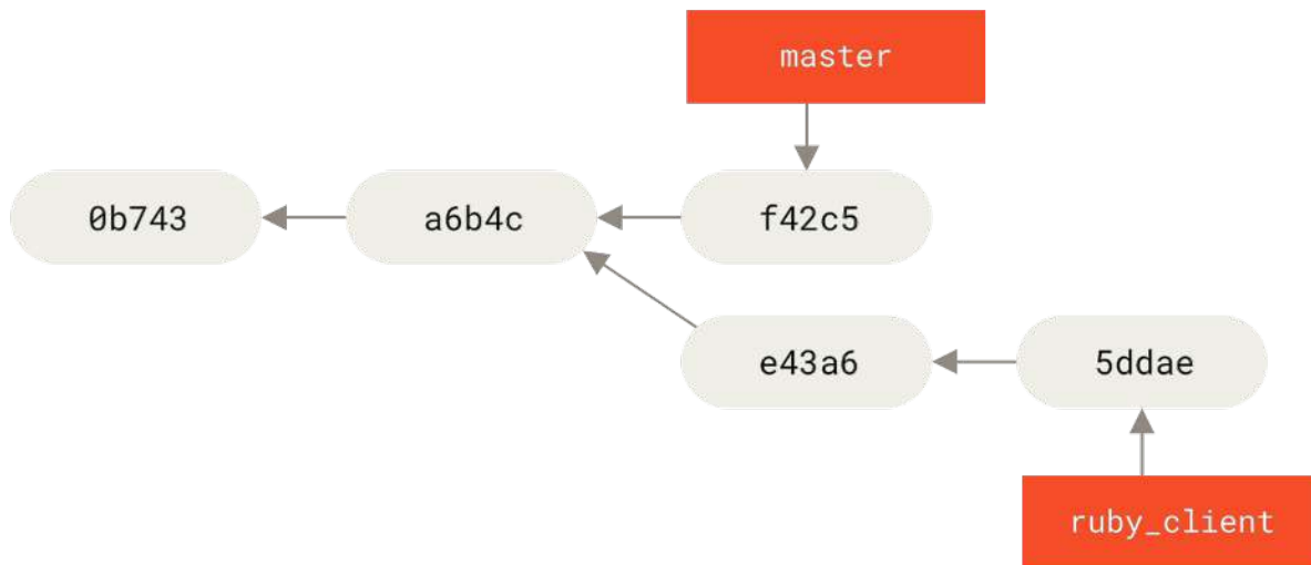
Figure 79. Example history before a cherry-pick
