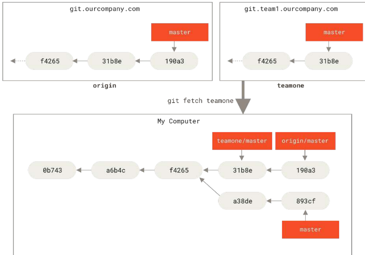
Figure 34. Remote-tracking branch for teamone/master
