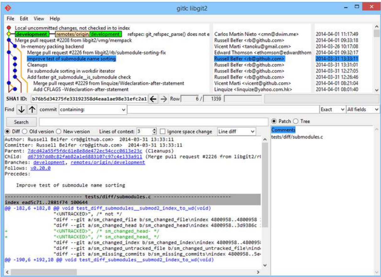
Figure 177. The gitk history viewer
