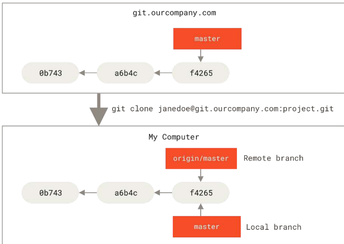
Figure 30. Server and local repositories after cloning
