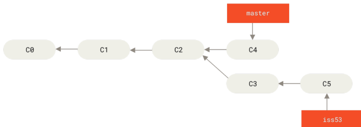
Figure 23. Work continues on iss53
