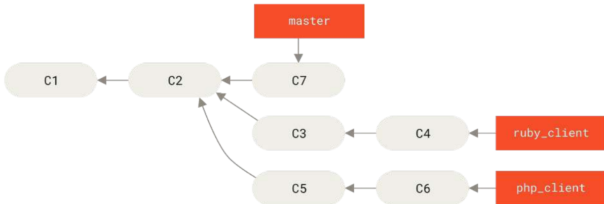
Figure 72. History with several topic branches
