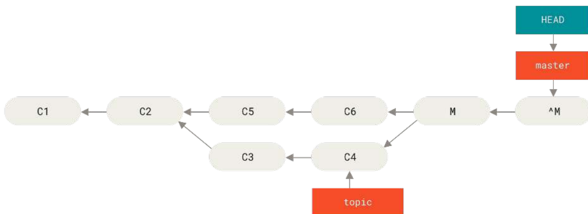
Figure 157. History after git revert -m 1
