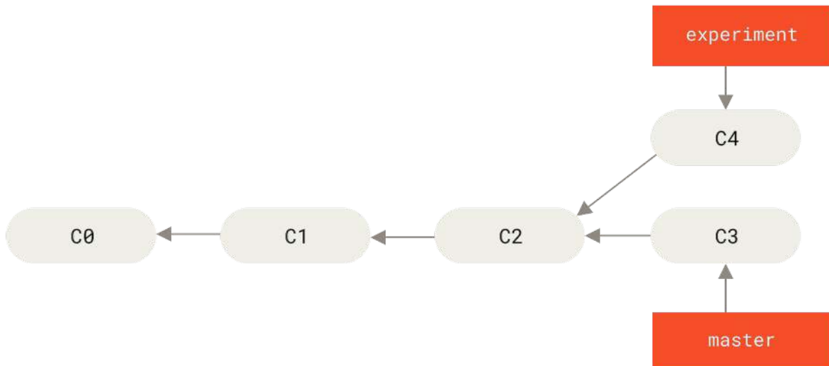
Figure 35. Simple divergent history
