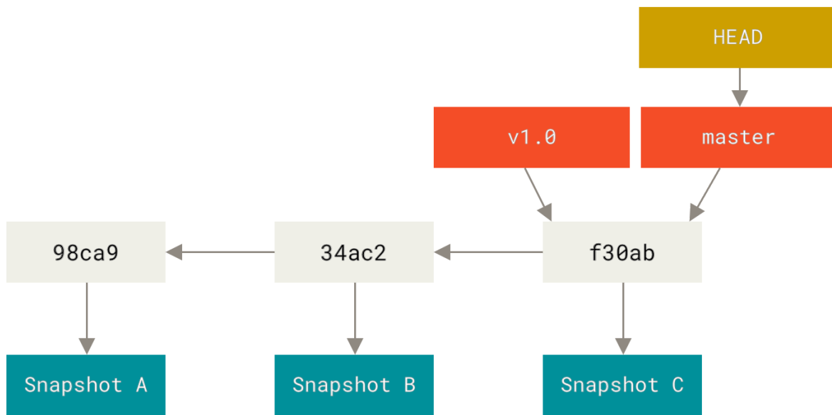
Figure 11. A branch and its commit history
