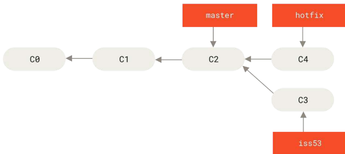
Figure 21. Hotfix branch based on master
