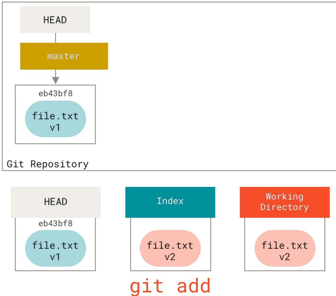
Figure 142. Staging change to index
