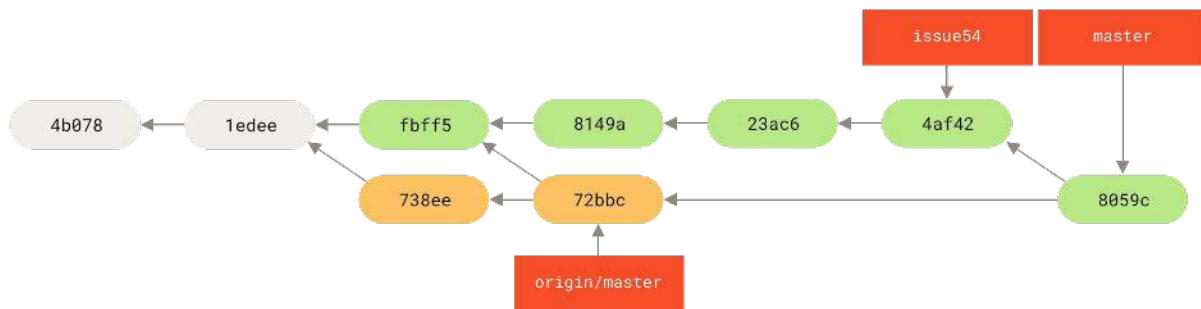
Figure 62. Jessica's history after merging John's changes
