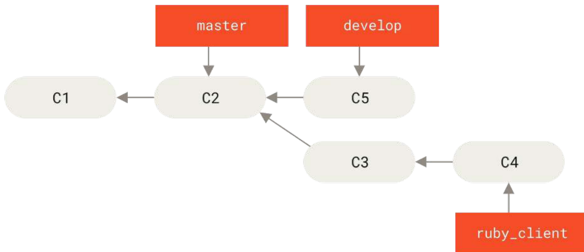
Figure 74. Before a topic branch merge
