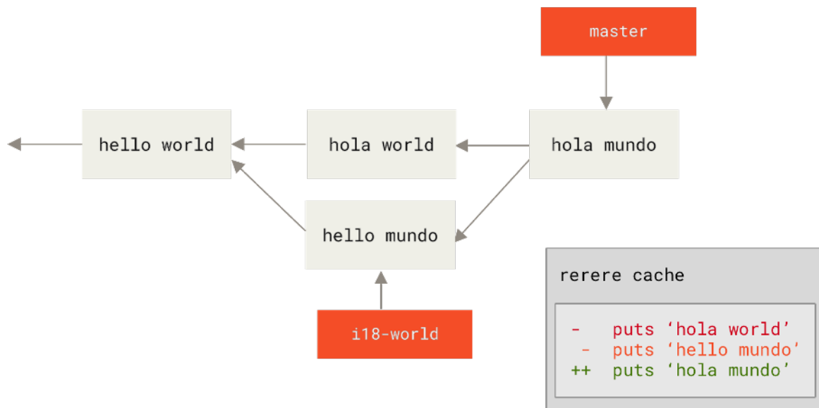
Figure 161. Recorded resolution for FILE
