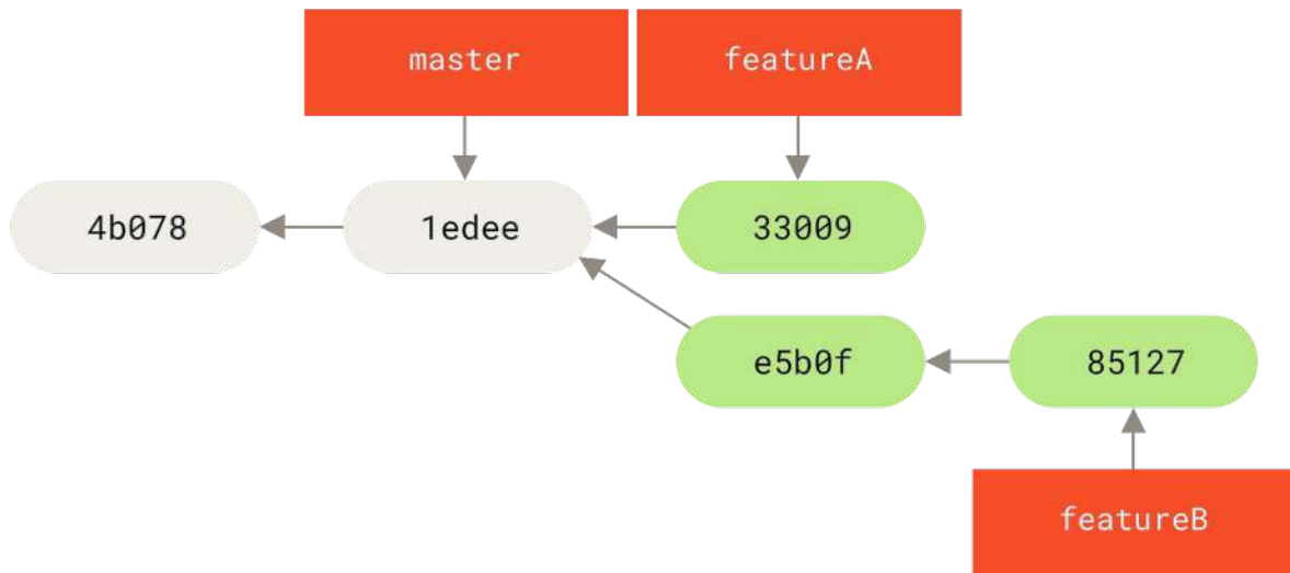
Figure 65. Jessica's initial commit history
