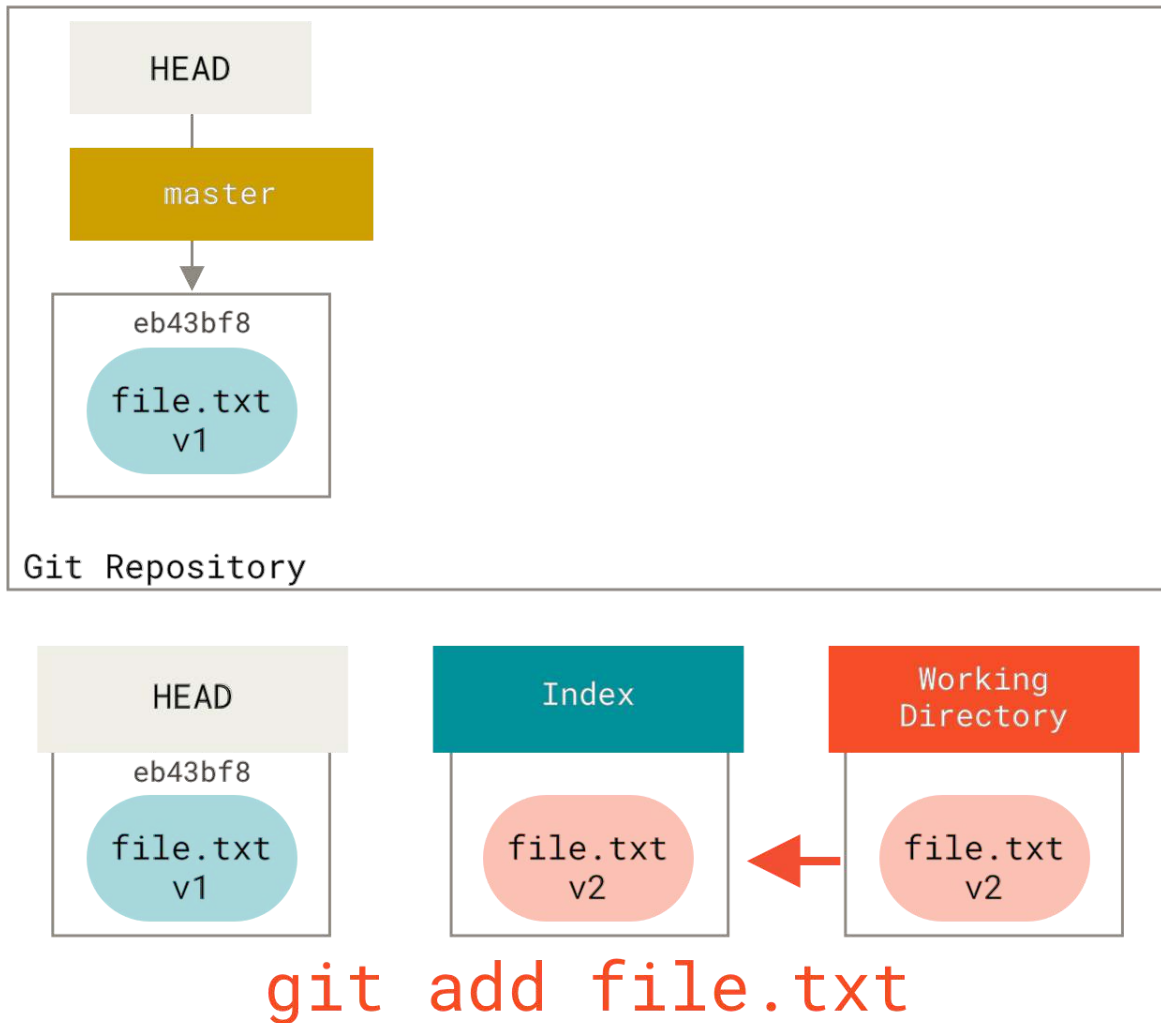
Figure 149. Staging file to index
