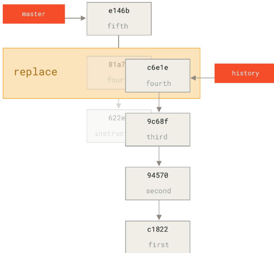
Figure 167. Combining the commits with git replace
