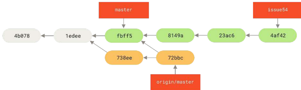
Figure 61. Jessica's history after fetching John's changes
