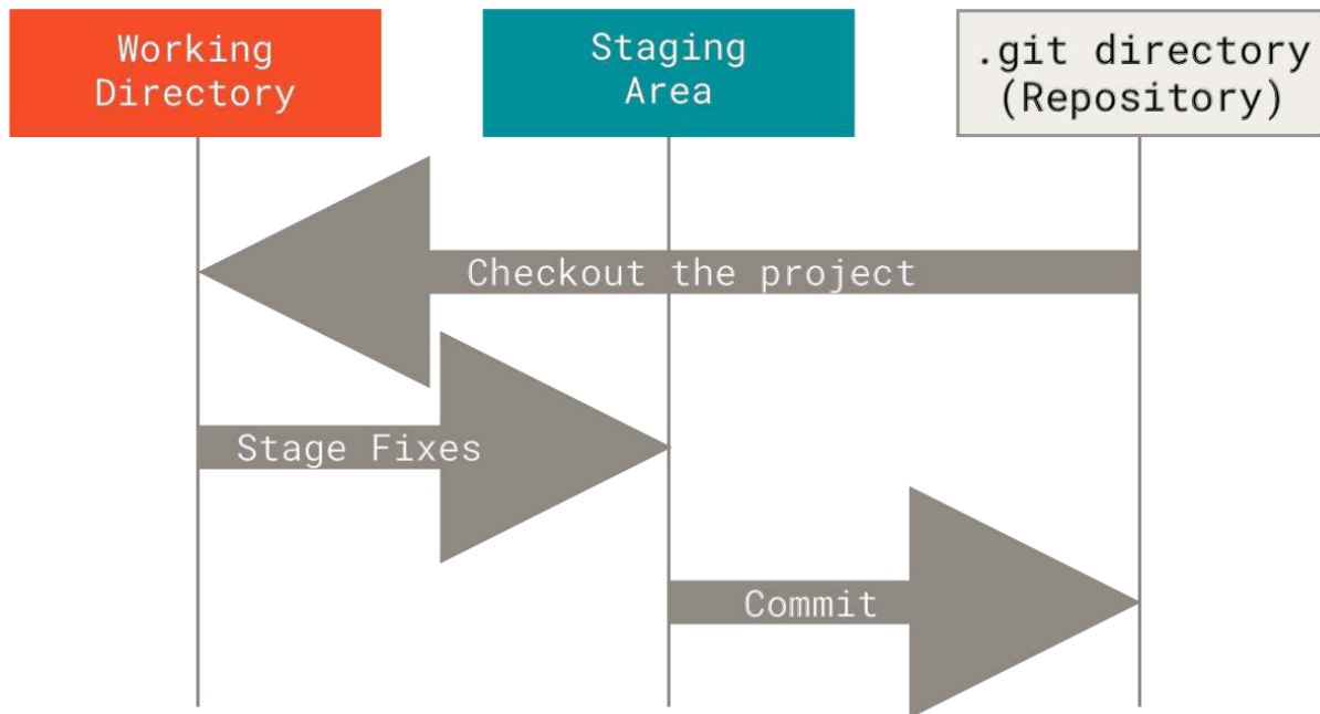
Figure 6. Working tree, staging area, and Git directory
