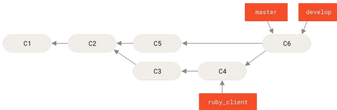
Figure 76. After a project release
