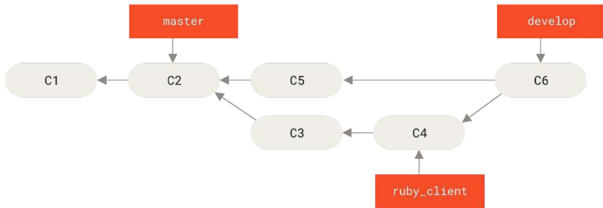
Figure 75. After a topic branch merge
