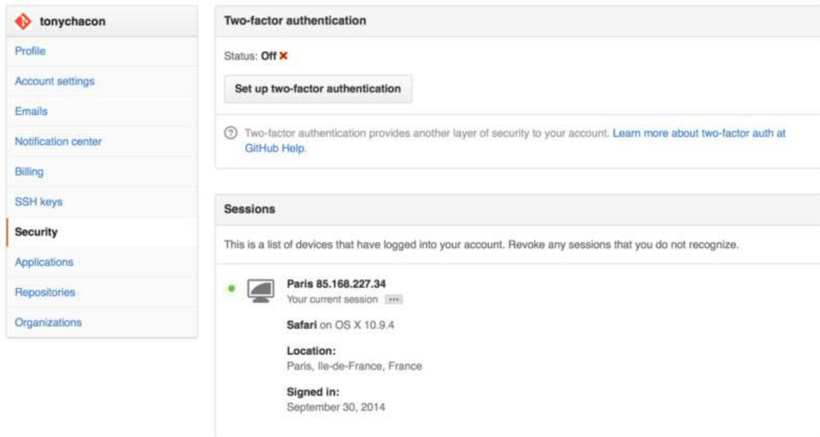
Figure 87. 2FA in the Security Tab
