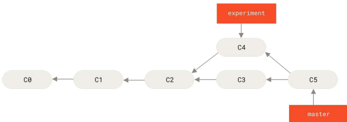
Figure 36. Merging to integrate diverged work history
