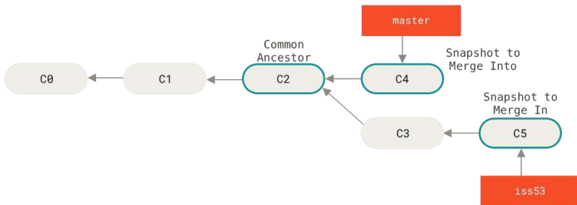
Figure 24. Three snapshots used in a typical merge
