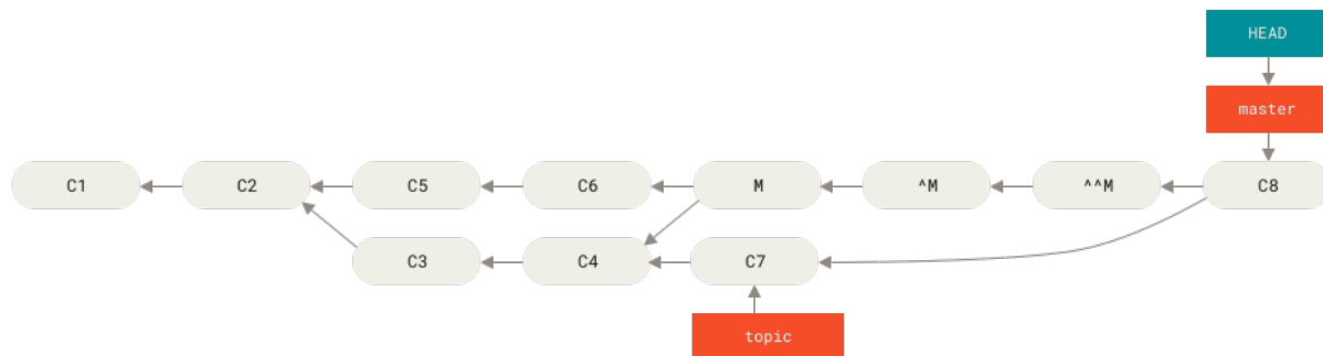
Figure 159. History after re-merging a reverted merge
