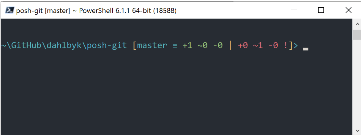
Figure 187. PowerShell with Posh-git
