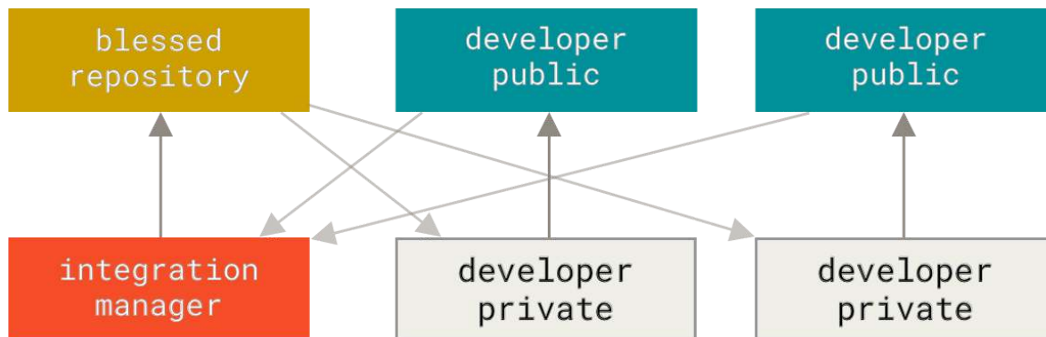
Figure 54. Integration-manager workflow
