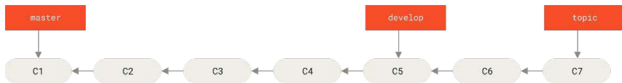
Figure 26. A linear view of progressive-stability branching
