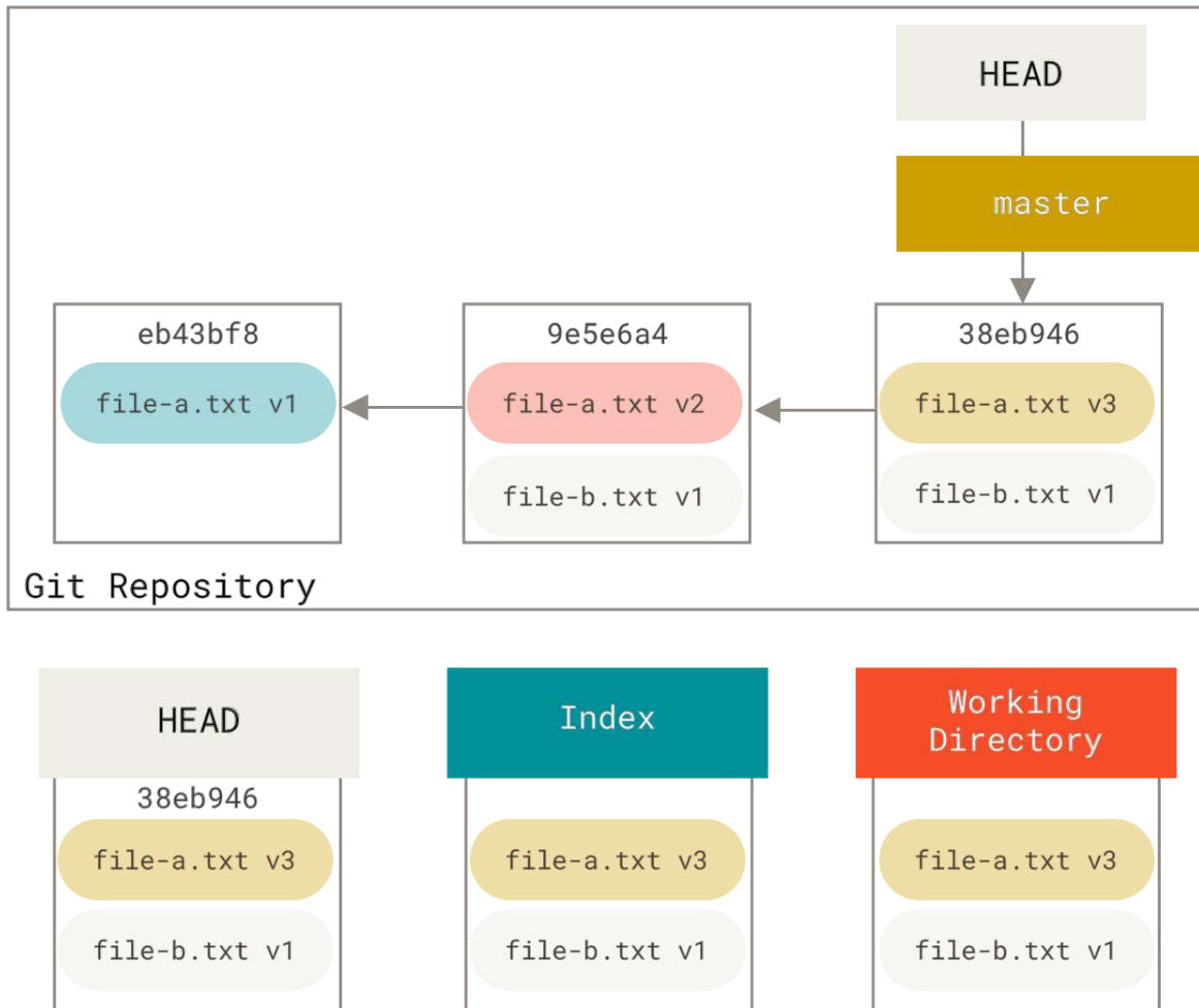
Figure 151. Git repository
