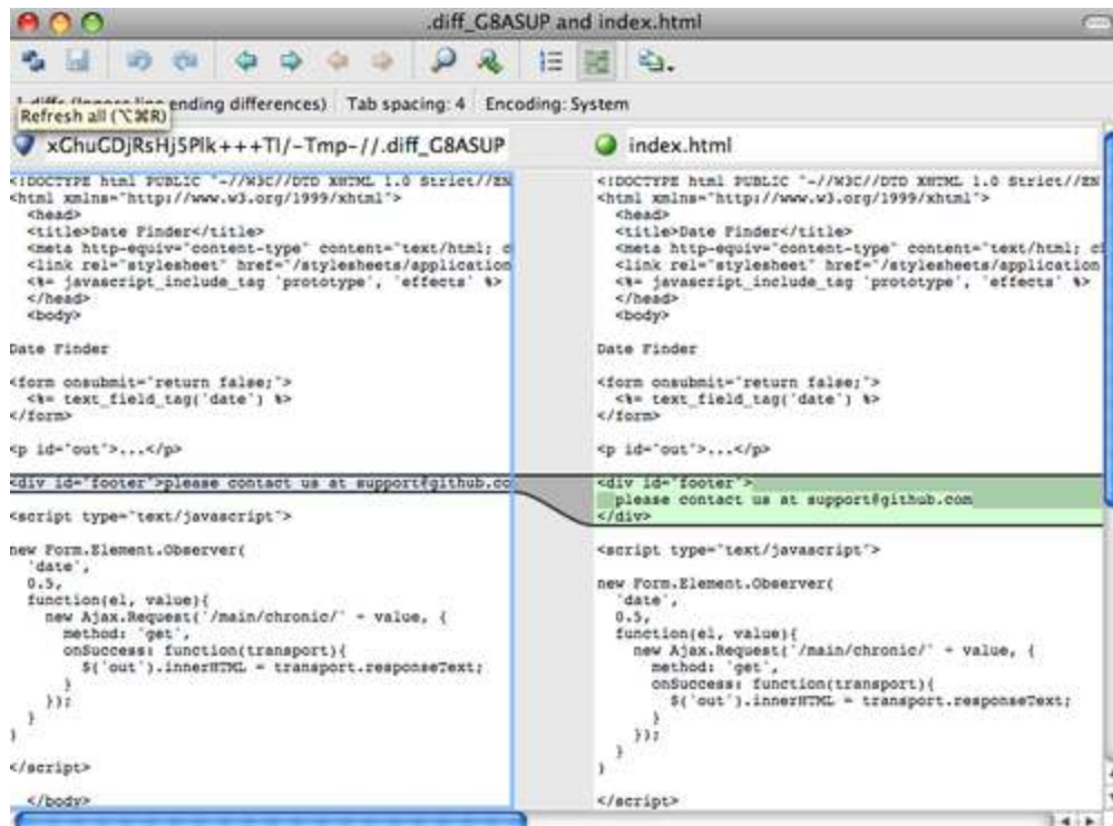
Figure 168. P4Merge
