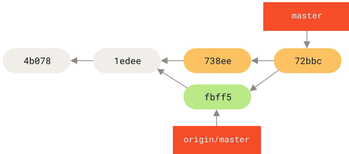
Figure 58. John's repository after merging origin/master
