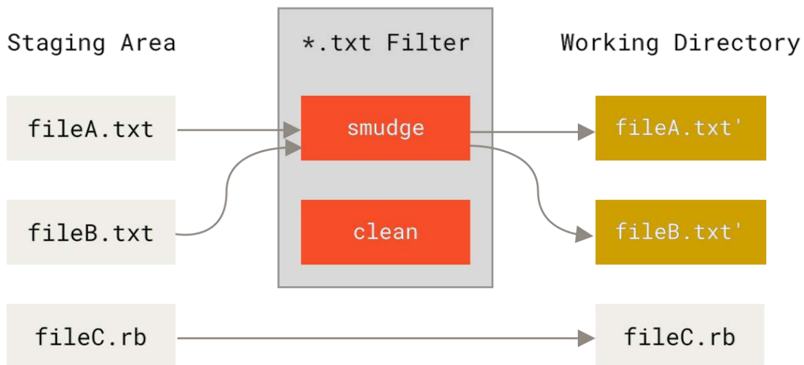
Figure 169. The “smudge” filter is run on checkout
