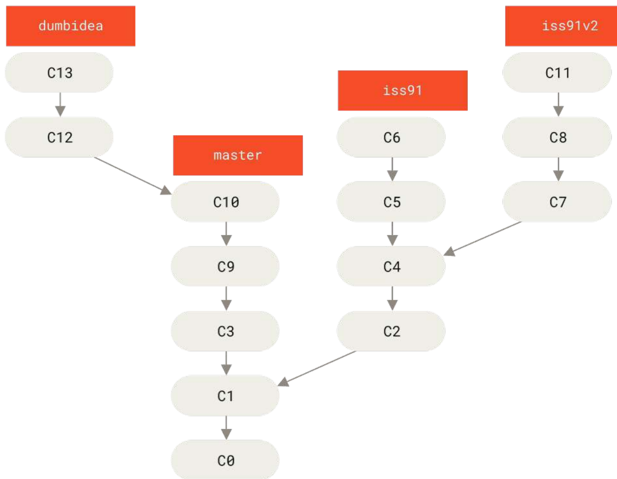
Figure 28. Multiple topic branches
