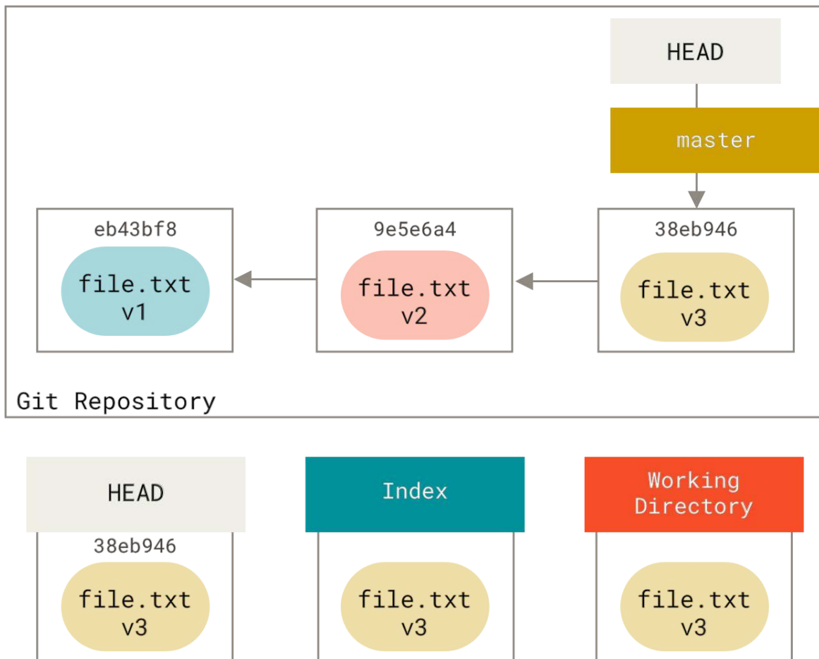
Figure 144. Git repository with three commits
