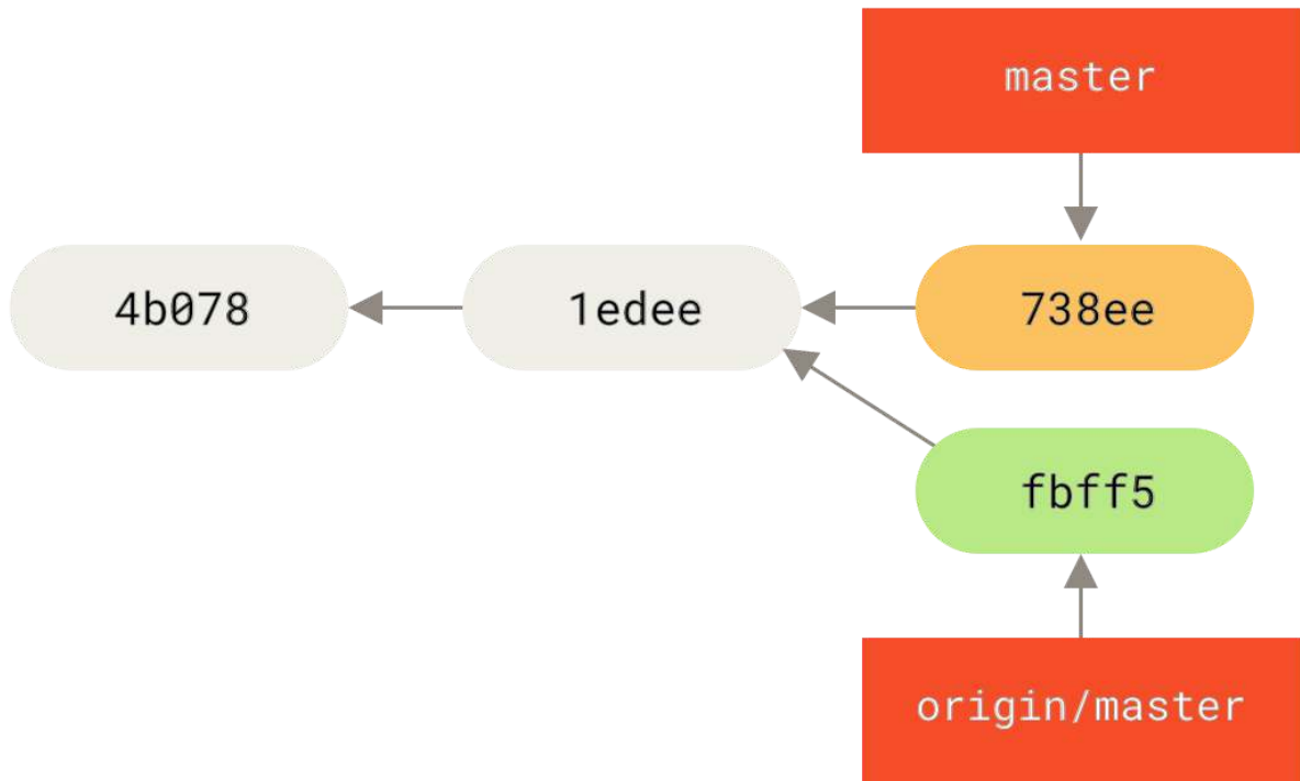
Figure 57. John's divergent history
